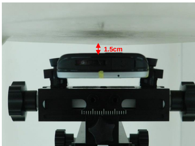
Back With Battery 1, Test Separation 1.5 cm
