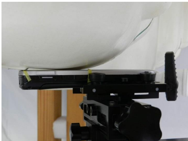
Right Cheek With Battery 1
