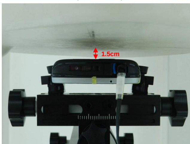
Back With Battery 1 and Headset, Test Separation 1.5 cm
