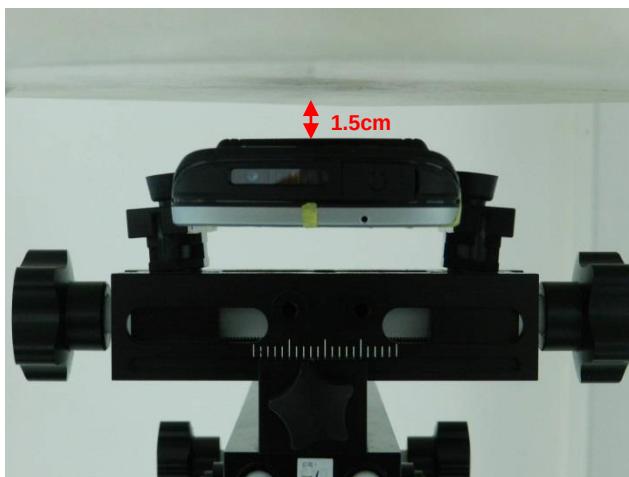
Back With Battery 2, Test Separation 1.5 cm
