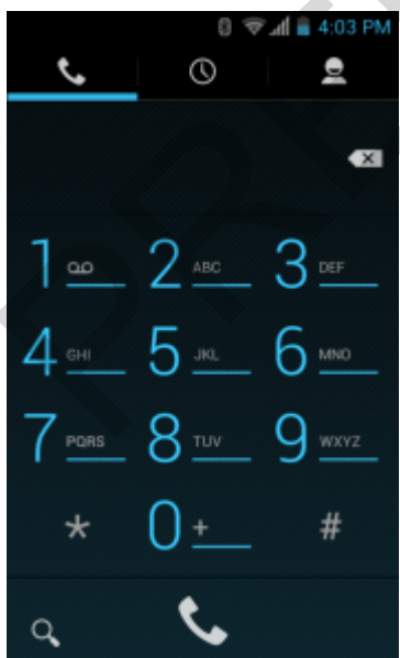
Figure 50: Dialer Screen
