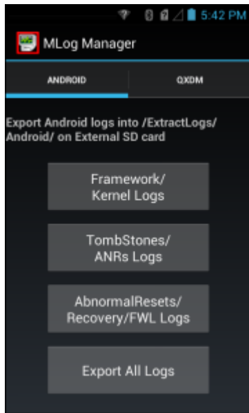
Figure 76: MLog Manager
