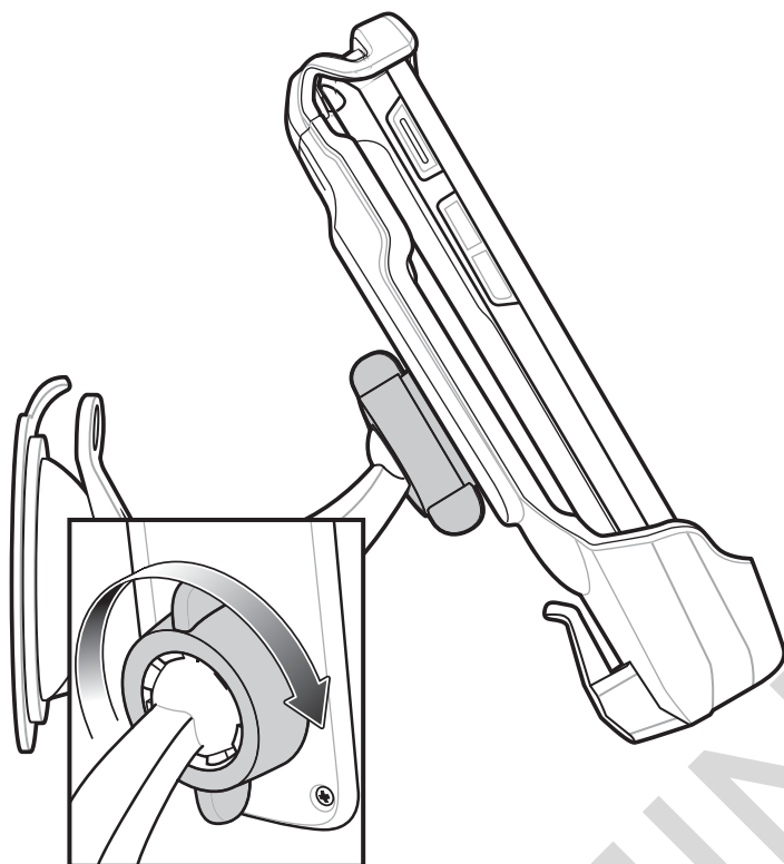
Figure 112: Tighten Nut
