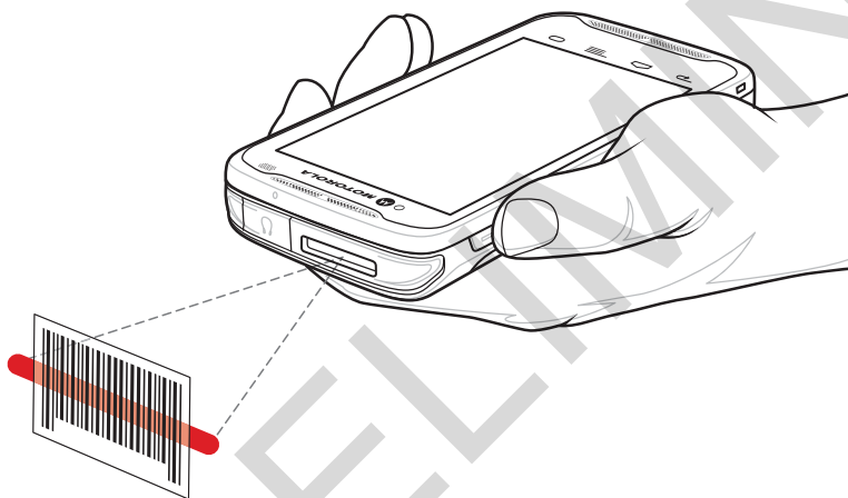
Figure 79: Scanning
