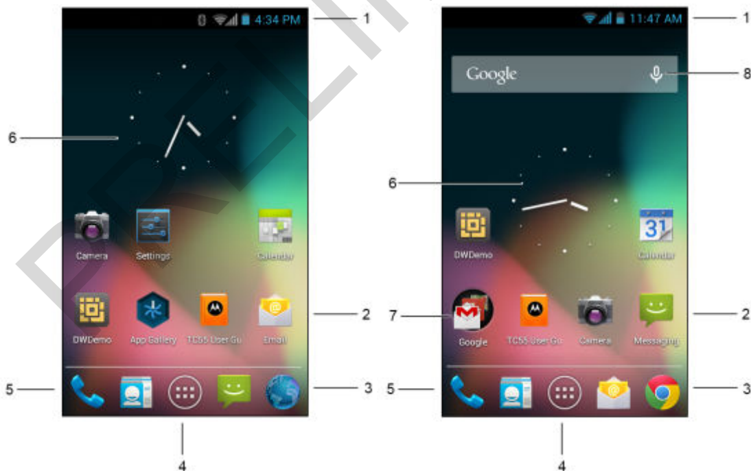
Figure 35: Home Screen
