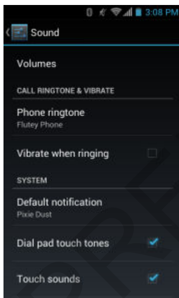
Figure 32: Sounds Screen
