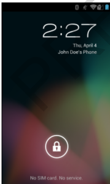
Figure 48: Lock Screen
