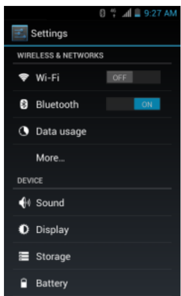
Figure 90: Settings Screen
