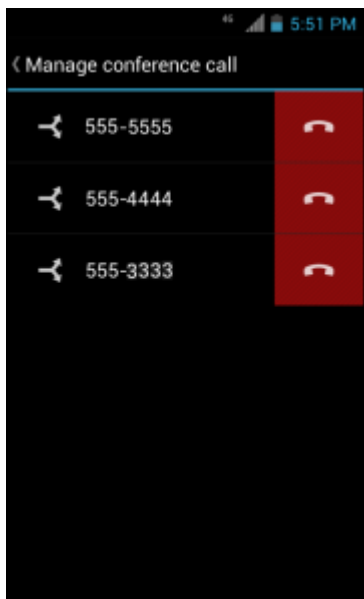
Figure 56: Un-merge Calls
