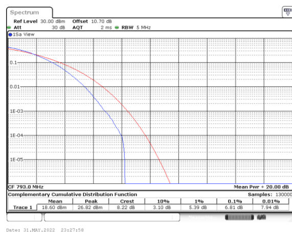
LTE Band 14 / 5MHz / 256QAM
