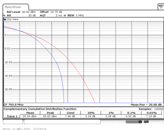
LTE Band 14 / 5MHz / 64QAM
