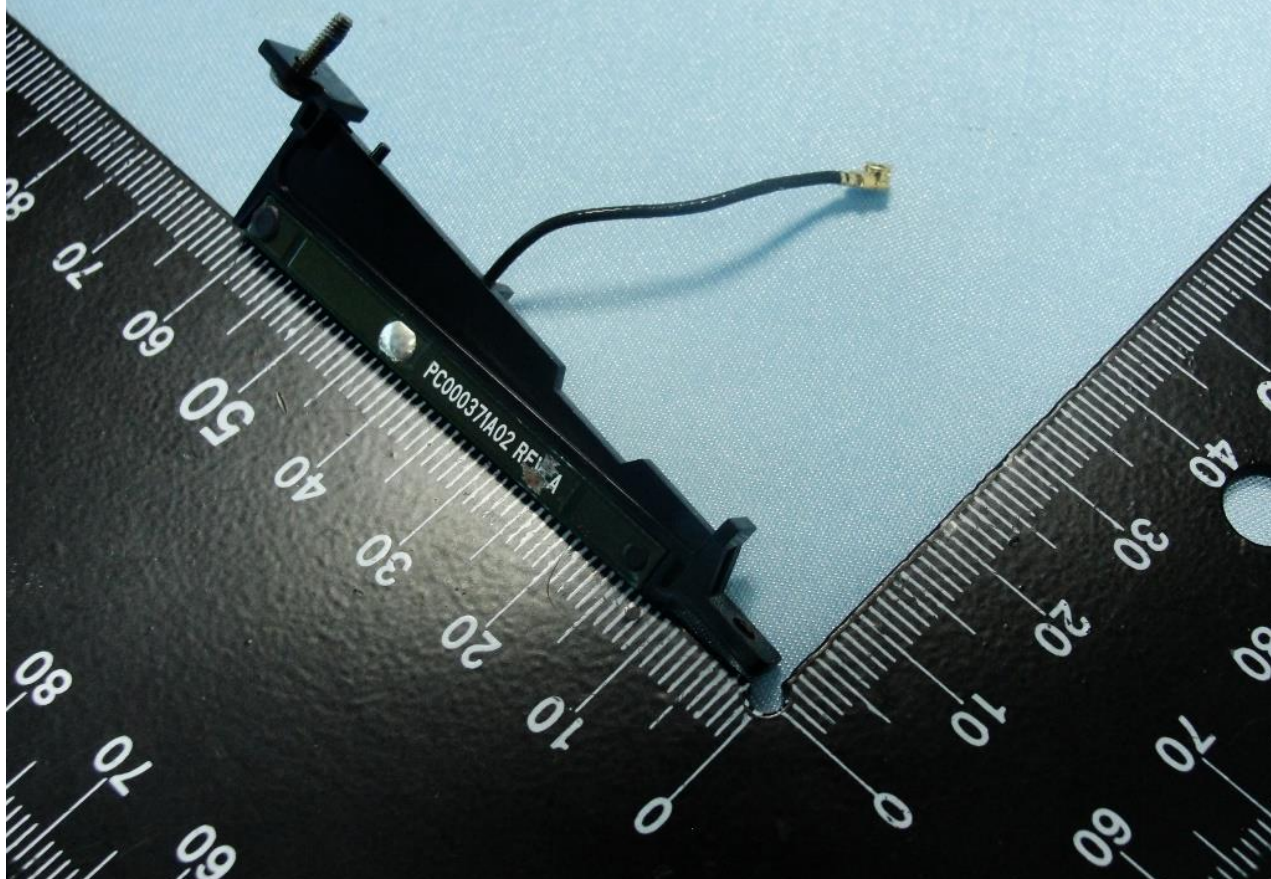
Bluetooth &amp; WLAN Antenna for Sample 1 ~ 3
