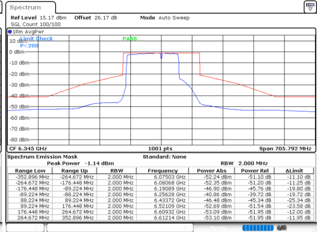
Plot on 6345 MHz
