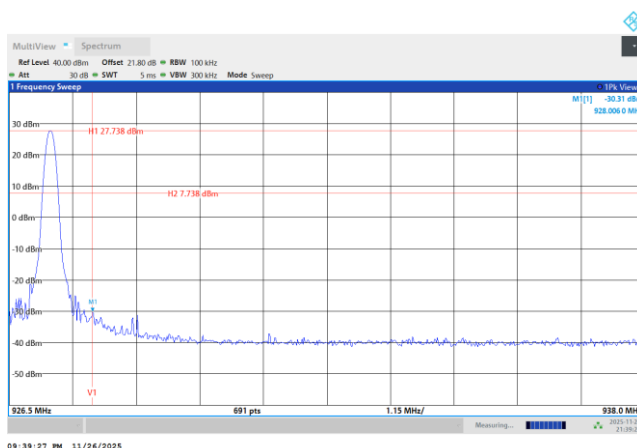
High Band Edge Plot on 927.25 MHz
