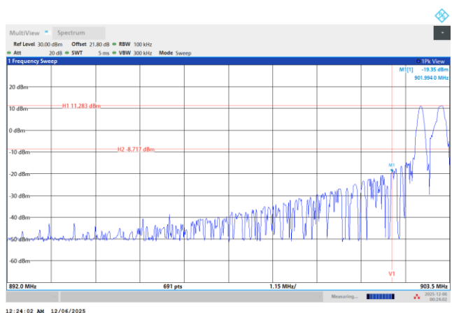
Hopping Mode Low Band Edge Plot on 902.75 MHz
