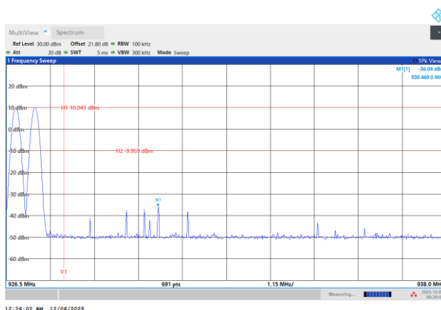
Hopping Mode High Band Edge Plot on 927.25 MHz
