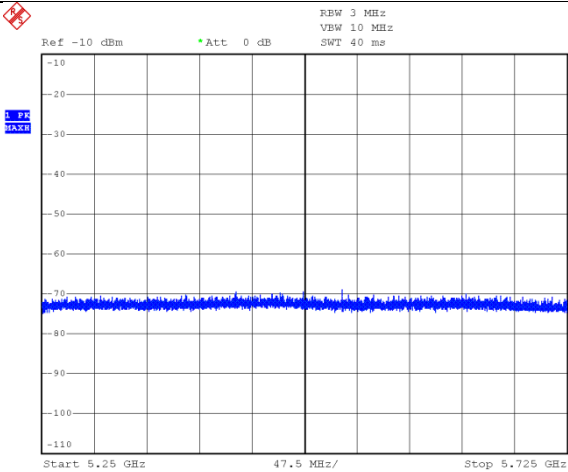
EUT (Client ) links with master on 802.11ac (VHT20) mode
