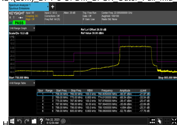
N14(10M) DFT-s-OFDM BPSK Outer Full Mid C
