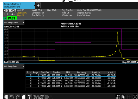
N14(5M)_DFT-s-OFDM_QPSK_Edge_1RB_Right_H igh CH
