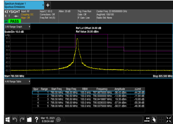
N14(5M)_DFT-s-OFDM_QPSK_Edge_1RB_Left_Mi d_CH
