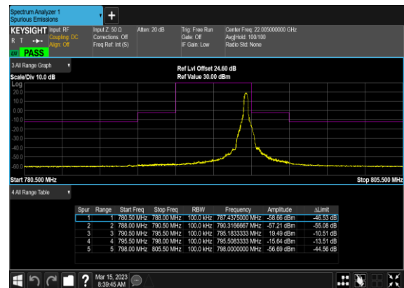
N14(5M)_DFT-s-OFDM_QPSK_Edge_1RB_Right_M id_CH
