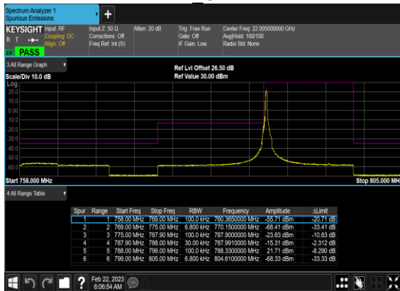
N14(5M)_DFT-s-OFDM_BPSK_Edge_1RB_Left_Lo w CH
