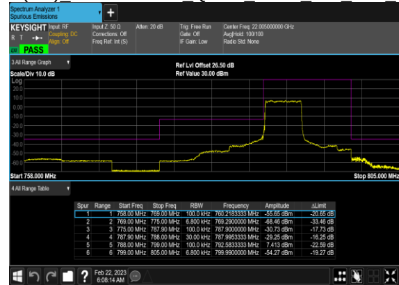
N14(5M)_DFT-s-OFDM_QPSK_Outer_Full_Low_CH
