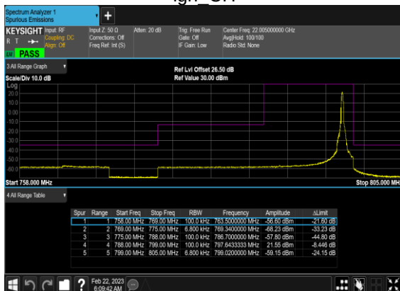
N14(5M)_DFT-s-OFDM_BPSK_Edge_1RB_Right_H igh CH
