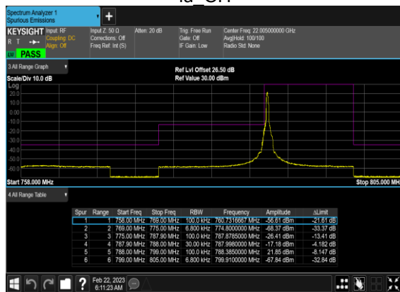
N14(10M)_DFT-s-OFDM_BPSK_Edge_1RB_Left_Mid_CH
