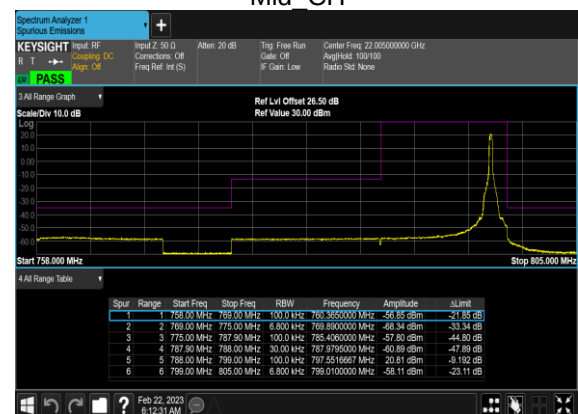
N14(10M)_DFT-s-OFDM_QPSK_Edge_1RB_Right_Mid_CH
