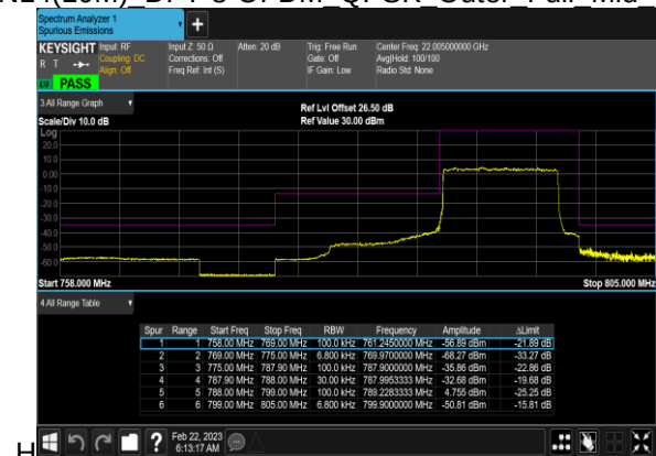
N14(10M) DFT-s-OFDM QPSK Outer Full Mid C
