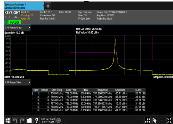
N14(5M)_DFT-s-OFDM_QPSK_Edge_1RB_Left_Lo w CH
