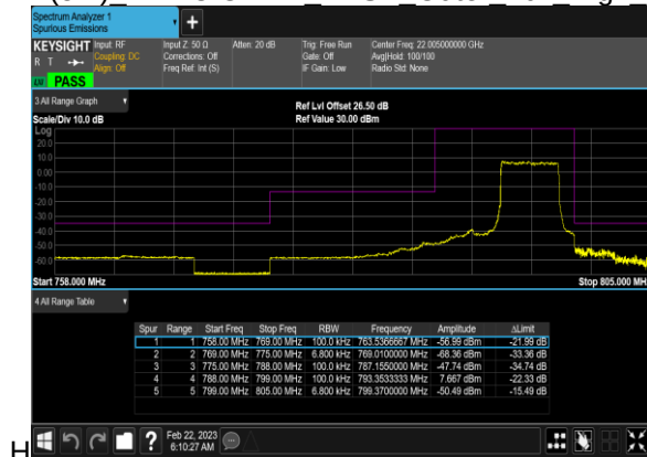
N14(5M)_DFT-s-OFDM_BPSK_Outer_Full_High_C
