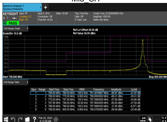
N14(10M)_DFT-s-OFDM_BPSK_Edge_1RB_Right_Mid_CH
