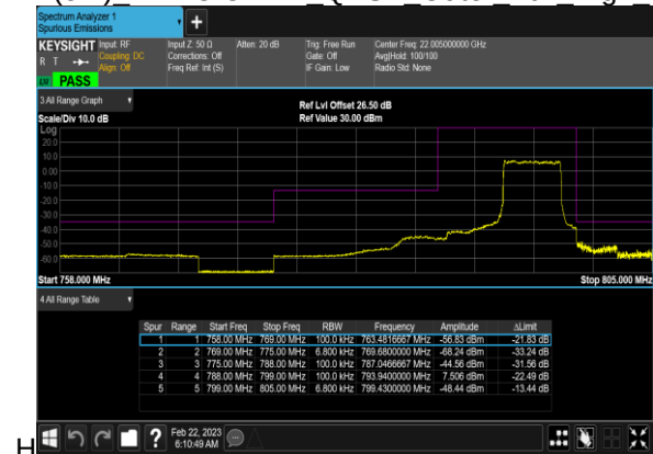
N14(5M)_DFT-s-OFDM_QPSK_Outer_Full_High_C
