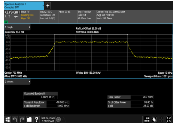
N14(5M)_CP-OFDM_16 QAM_Outer_Full_Mid_CH
