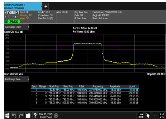
N14(5M)_DFT-s-OFDM_QPSK_Outer_Full_Mid_CH
