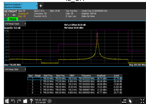
N14(10M)_DFT-s-OFDM_QPSK_Edge_1RB_Left_Mid_CH
