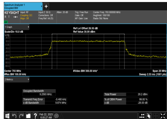
N14(10M)_CP-OFDM_16 QAM_Outer_Full_Mid_CH
