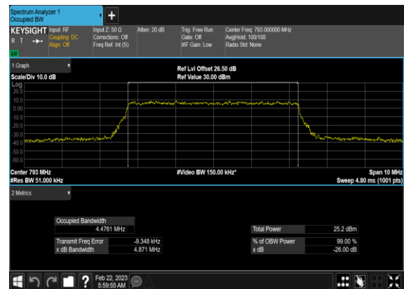
N14(5M)_CP-OFDM_256 QAM_Outer_Full_Mid_CH
