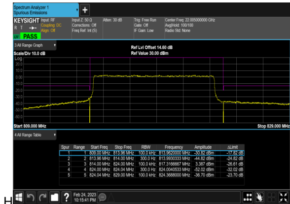
N26(10M)_DFT-s-OFDM_QPSK_Outer_Full_Mid_C
