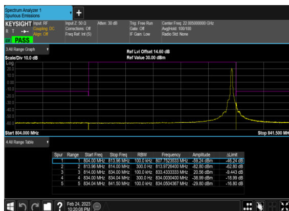
N26(20M)_DFT-s-OFDM_BPSK_Edge_1RB_Right_
