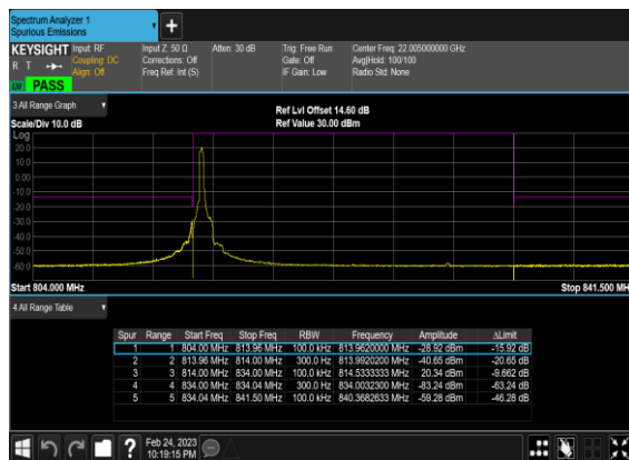
N26(20M)_DFT-s-OFDM_BPSK_Edge_1RB_Right_
