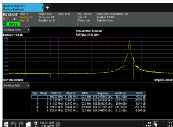
N26(10M)_DFT-s-OFDM_BPSK_Edge_1RB_Right_
