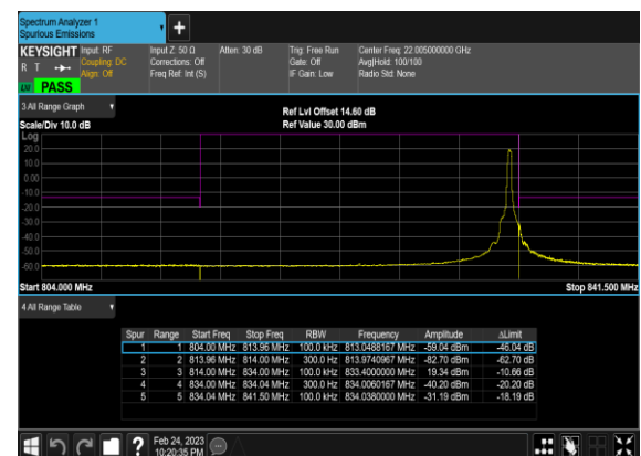
N26(20M)_DFT-s-OFDM_QPSK_Edge_1RB_Right_
