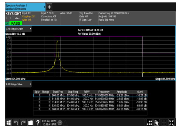
N26(20M)_DFT-s-OFDM_QPSK_Edge_1RB_Right_
