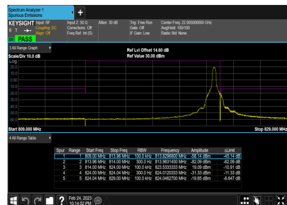
N26(10M)_DFT-s-OFDM_QPSK_Edge_1RB_Right_
