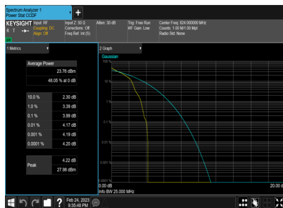
N26(20M)_DFT-s-OFDM_PI_2-BPSK_Edge_1RB _Left_Mid_CH
