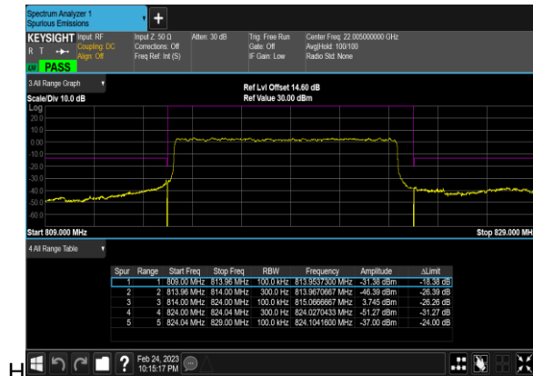
N26(10M)_DFT-s-OFDM_BPSK_Outer_Full_Mid_C
