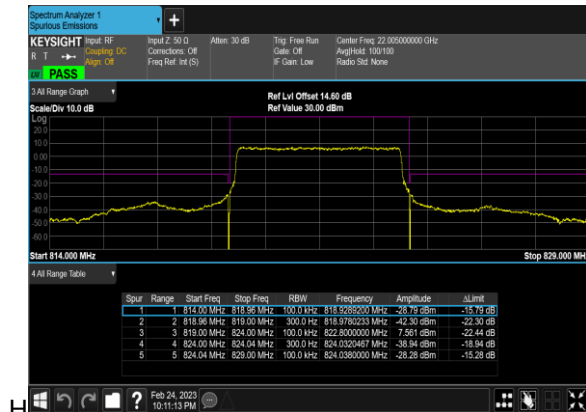
N26(5M)_DFT-s-OFDM_BPSK_Outer_Full_High_C
