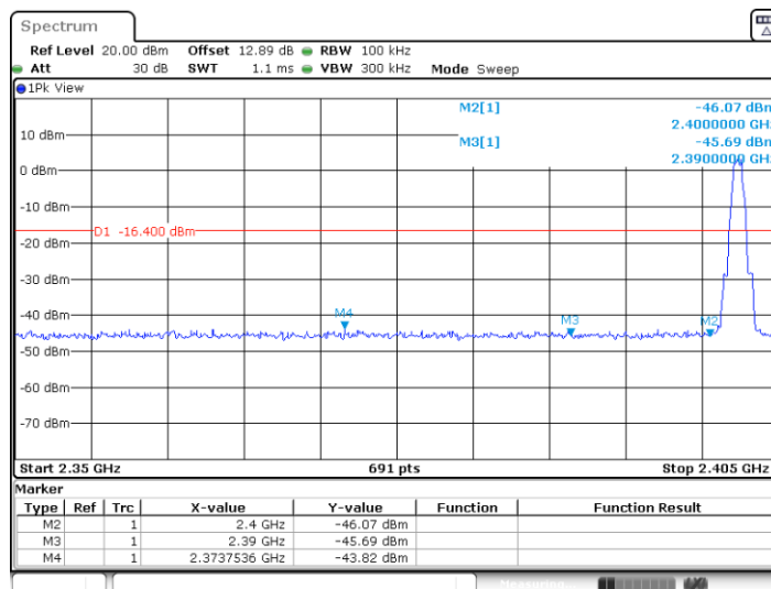
BLE_1M_Ant7_Low_2402
