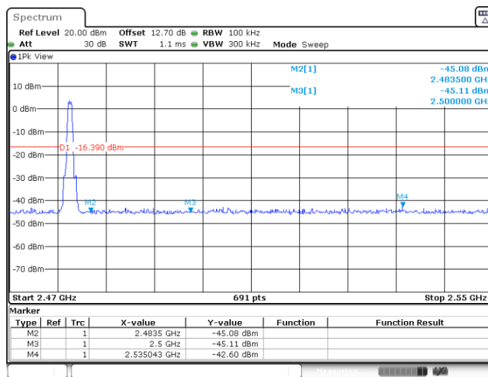
BLE_1M_Ant7_High_2480
