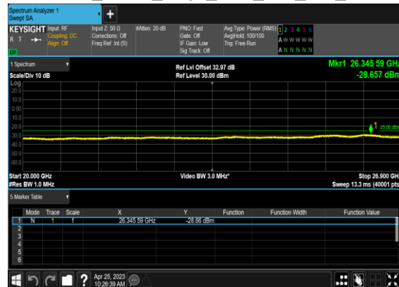
N41(20M)_DFT-s- OFDM_BPSK_Edge_1RB_Left_Mid_CH
