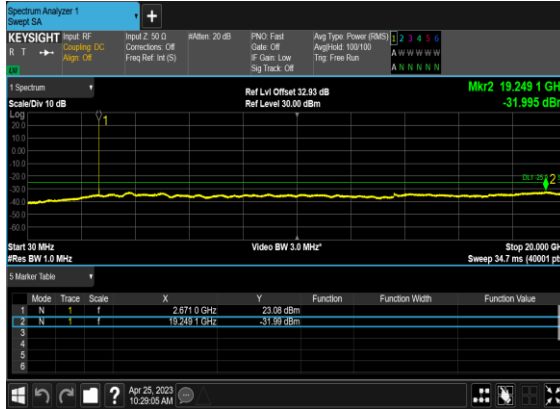
N41(20M)_DFT-s- OFDM_BPSK_Edge_1RB_Left_High_CH
