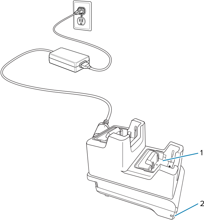
Figure 4 2-Slot Charge Only Cradle
