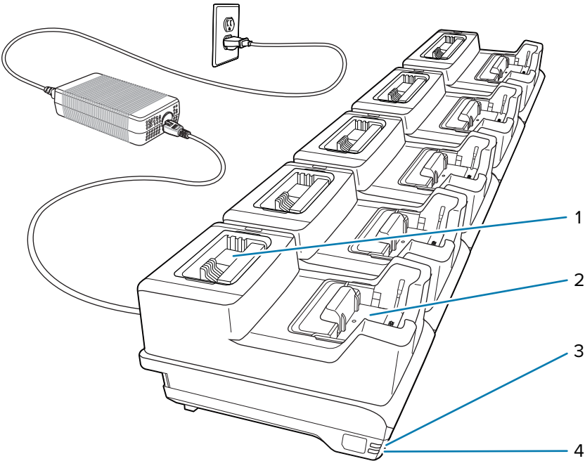
Figure 6 5-Slot Ethernet Cradle with Battery Charger
