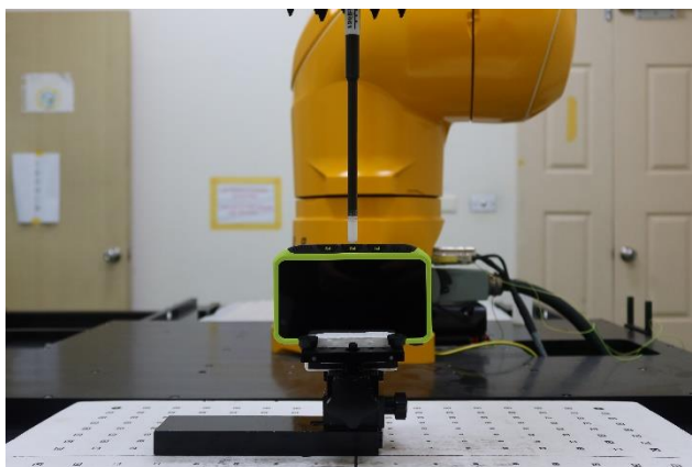
Bottom Side with Battery 2 at 2 mm
