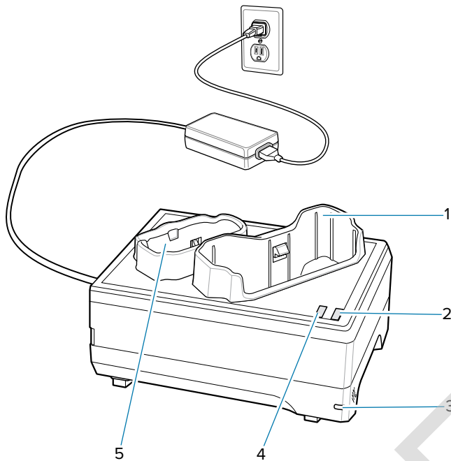
Figure 13 2-Slot Device/RS6000 Charging Cradle
