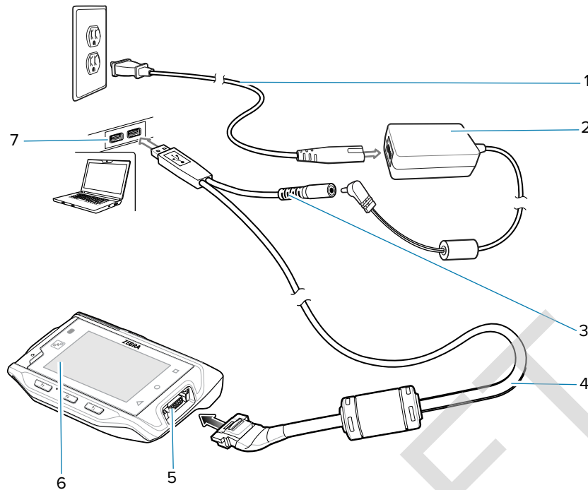
Figure 20 USB and Charging Cable
