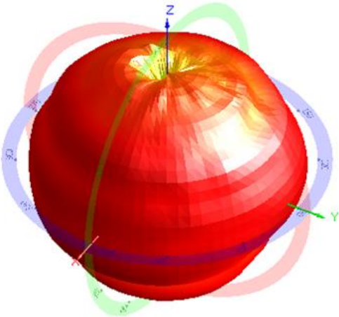
[3D Radiation Pattern : On the EVB @2442 MHz]
