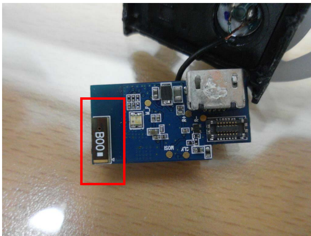
BT Antenna
