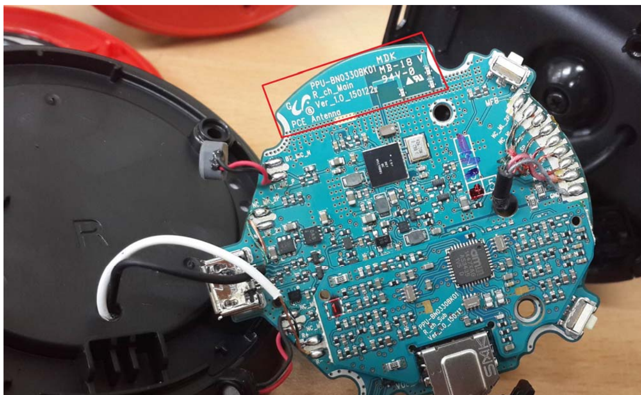
BT Antenna
