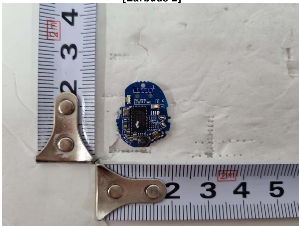
[Earbuds L]
