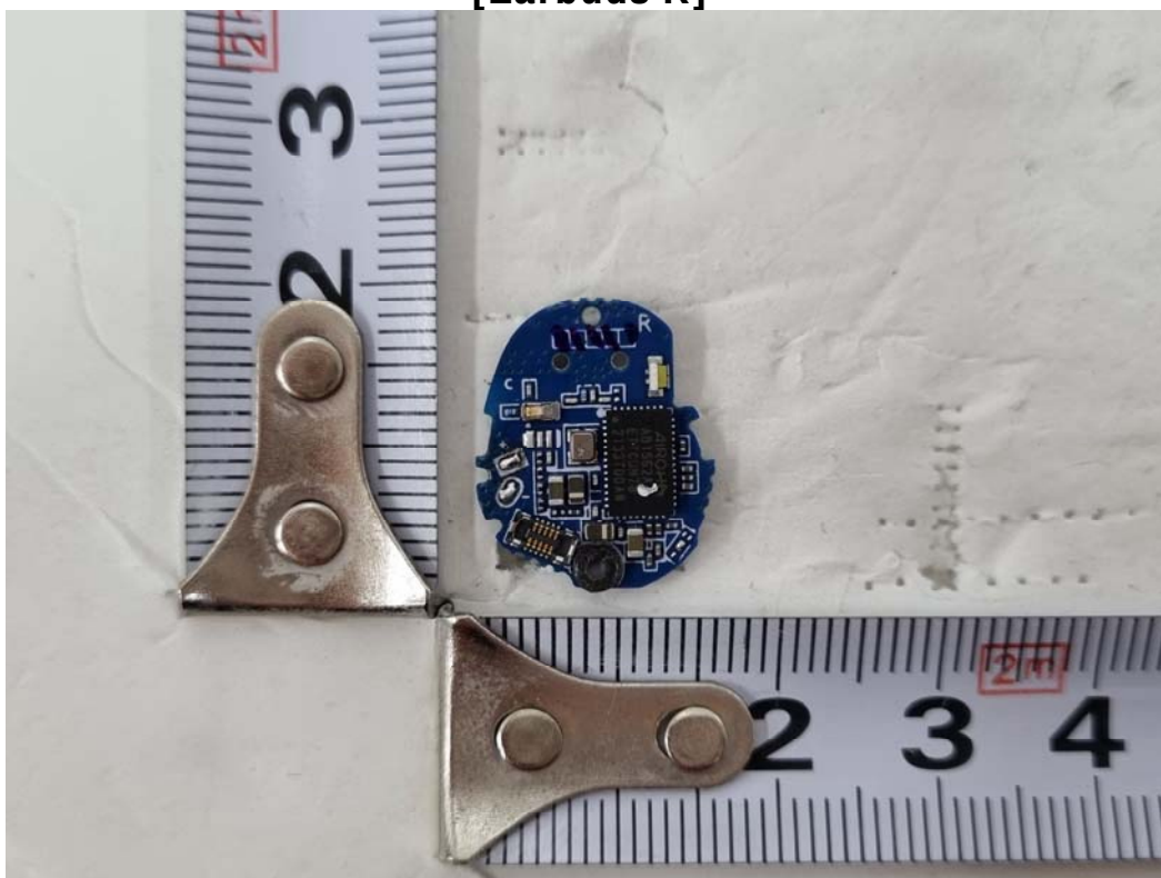
[Earbuds R]
