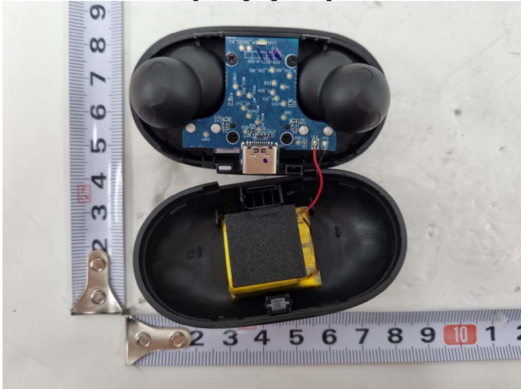
[Charging case]
