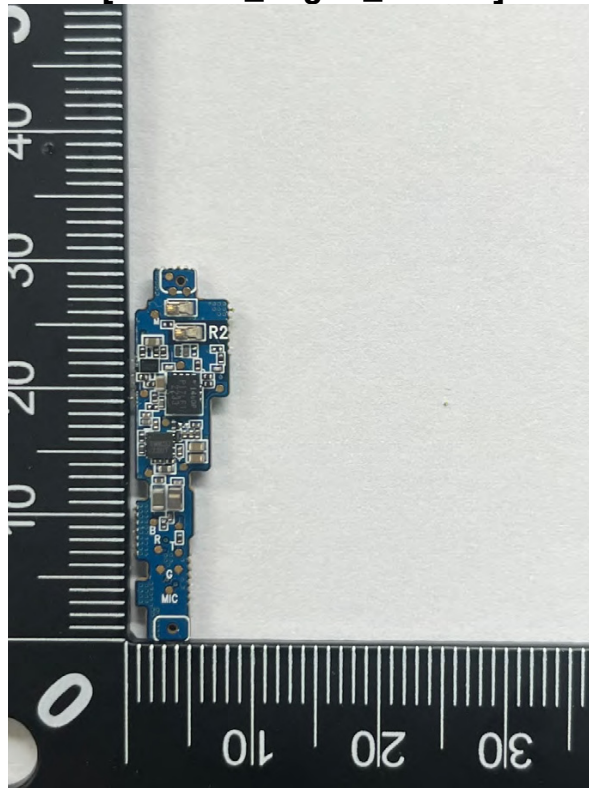
[Earbud_Right_Board]
