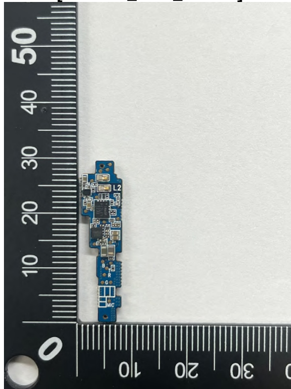
[Earbud_Left_Board]
