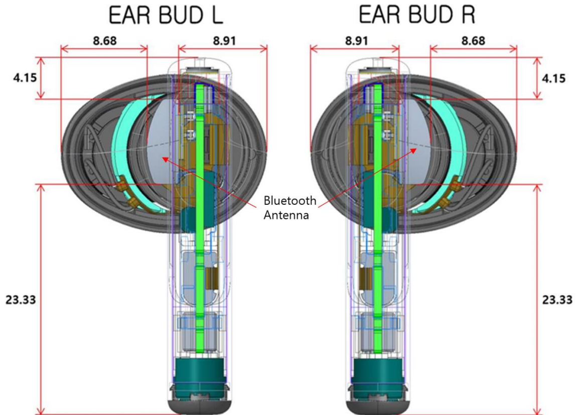
Figure E-1 Antenna Location (Rear Side View)
