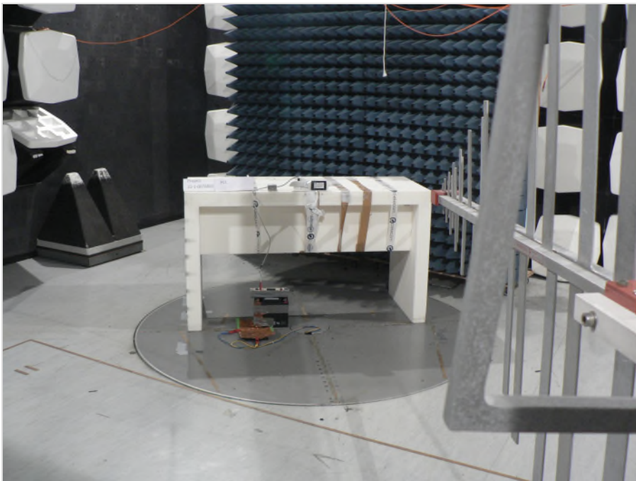
Photograph 6: Setup in the semi anechoic chamber, measurement >30 MHz, overview, with NFC-Tag
