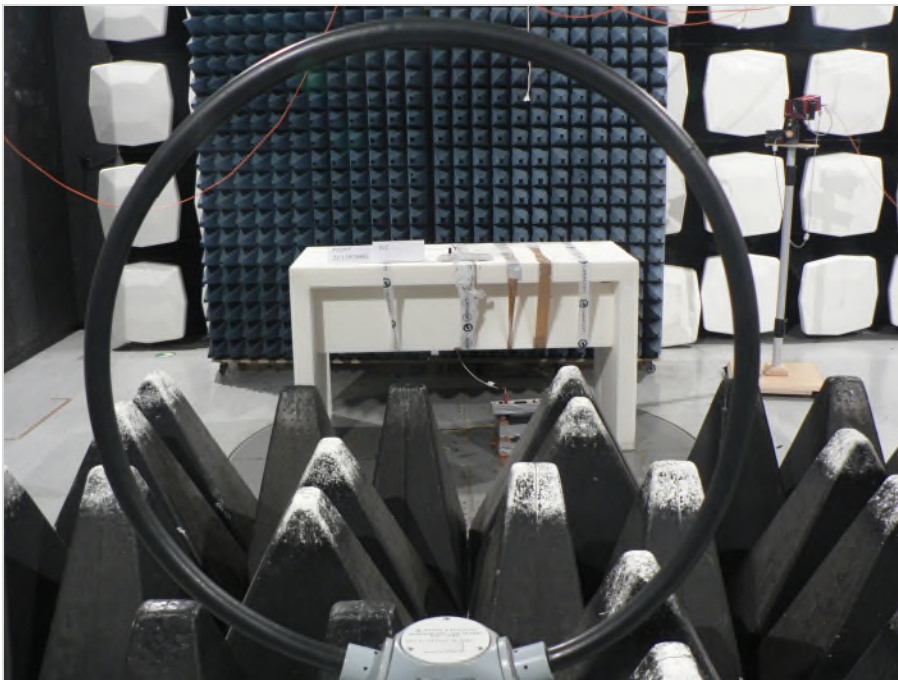
Photograph 4: Setup in the semi anechoic chamber, measurement <30 MHz, overview, without NFC-Tag
