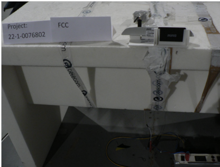
Photograph 5: Setup in the semi anechoic chamber, measurement <30 MHz, close up view, with NFC-Tag
