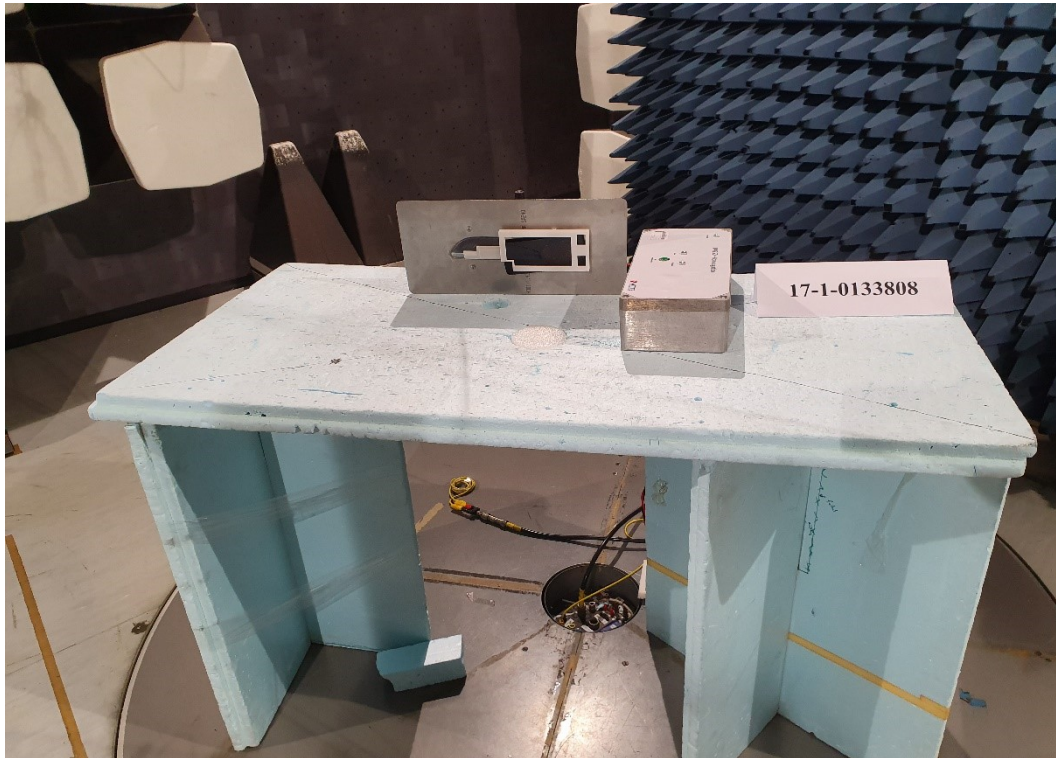
Photograph 1: Close view EUT position standing
