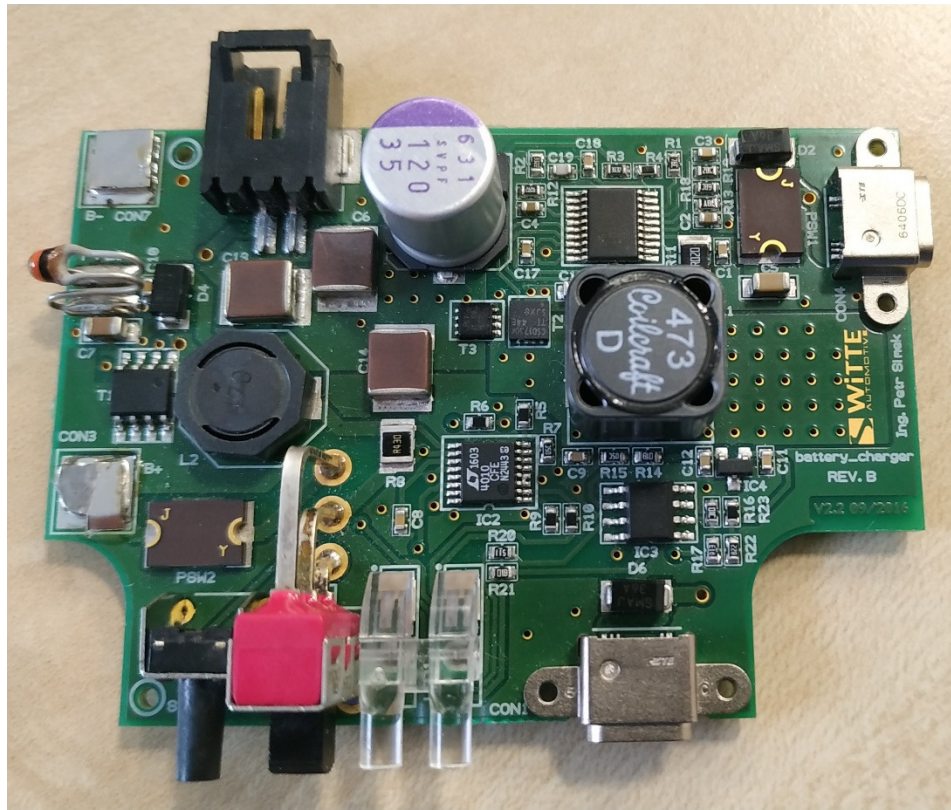
PCB 2 top side
