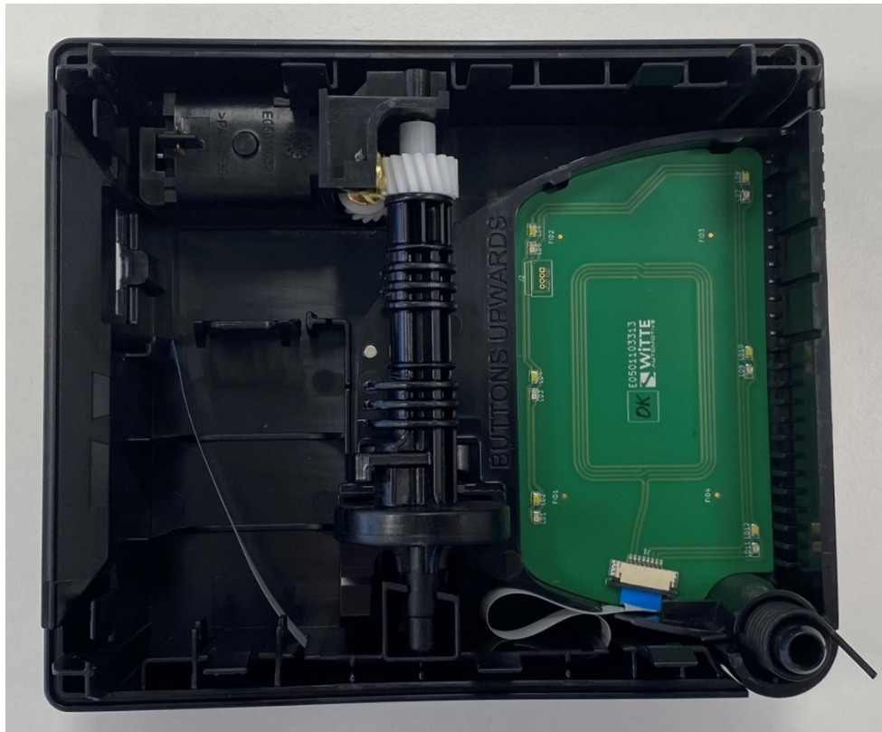
flinkey BLE lower part without main PCB and without keyboard
