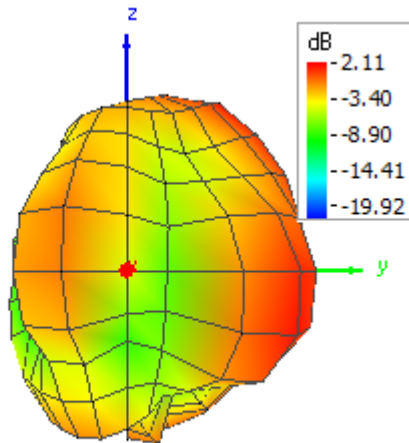
Theta = 90, Phi = 270
