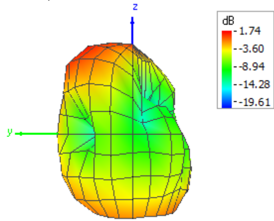
Theta = 90, Phi = 180
