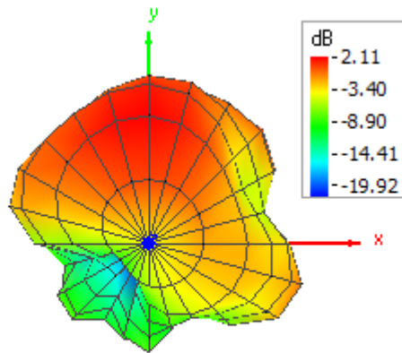
Theta = 0, Phi = 0
