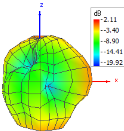
Theta = 90, Phi = 270
