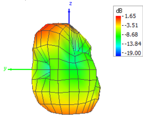
Theta = 90, Phi = 180
