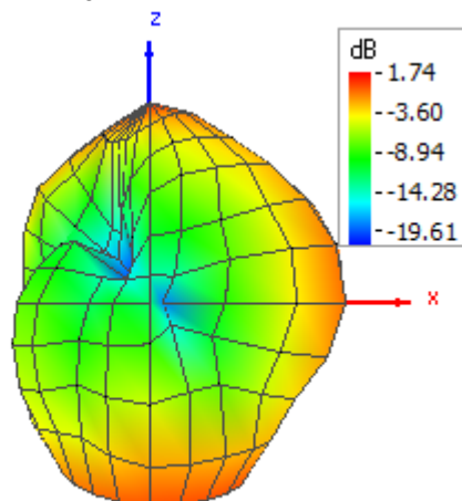
Theta = 90, Phi = 270
