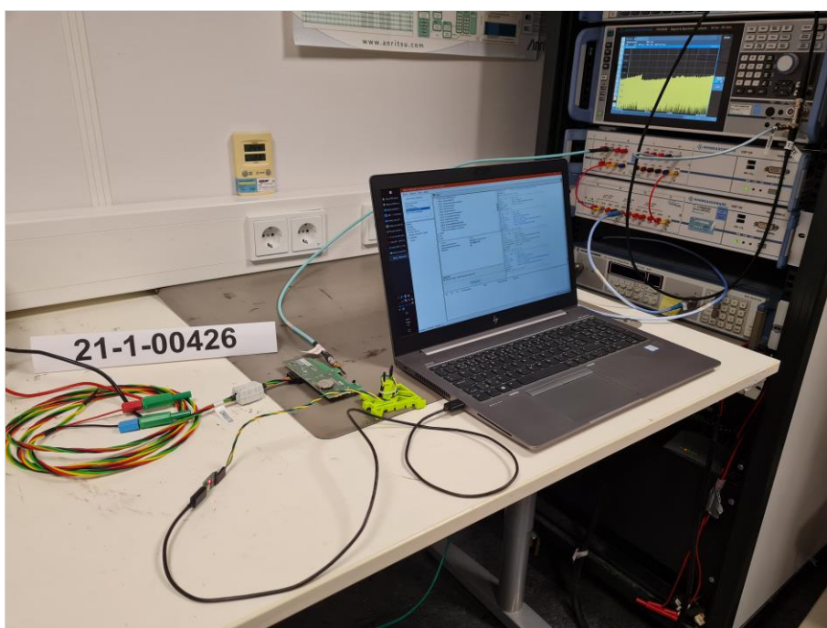
Photograph 8: EUT setup conducted measurement, overview
