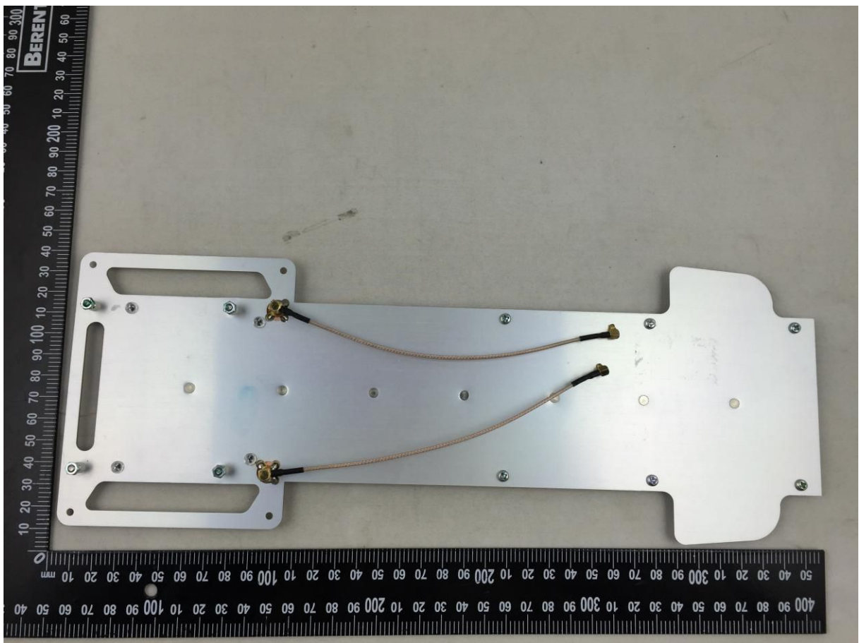
18 dBi Antenna
