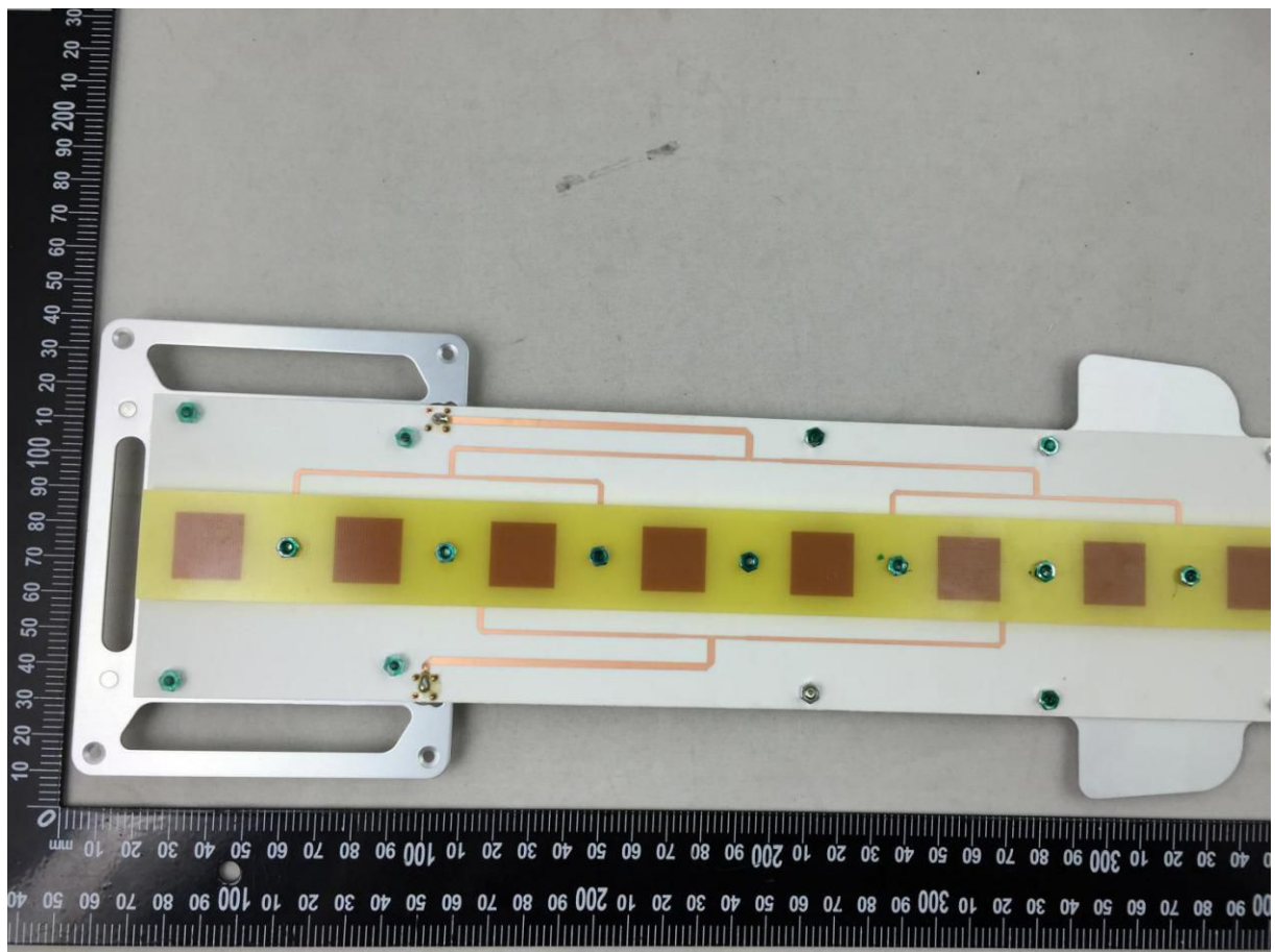
18 dBi Antenna
