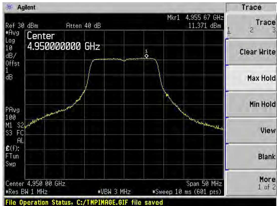
Chain 1 PSD (3 dBi Antenna)-Low Channel
