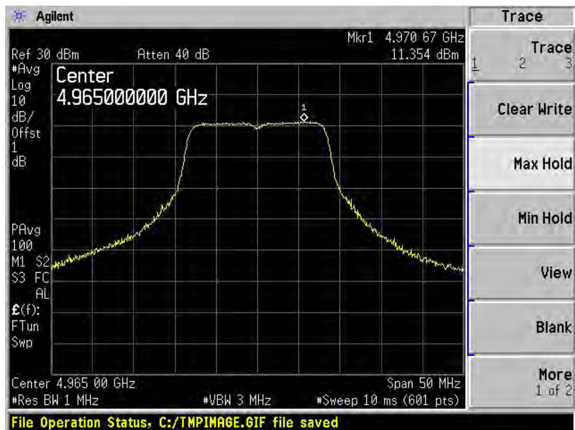
Chain 1 PSD (3 dBi Antenna)-Mid Channel
