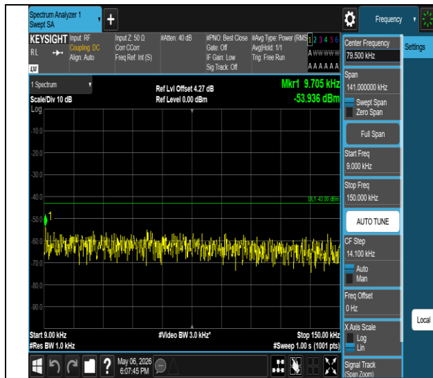
Band IV-1312-0.009~0.15MHz-PASS
