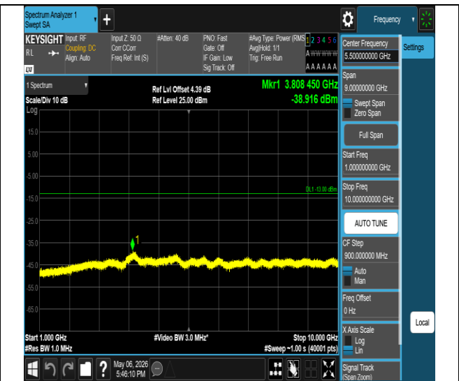
Band V-4182-1000~10000MHz-PASS
