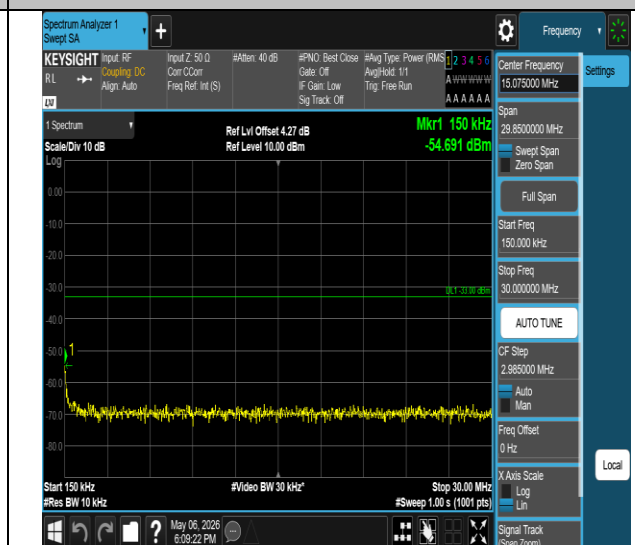
Band IV-1513-0.15~30MHz-PASS
