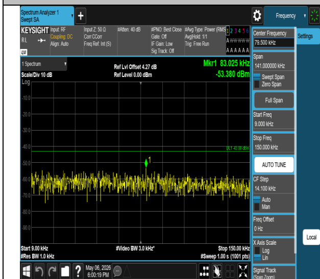
Band II-9538-0.009~0.15MHz-PASS
