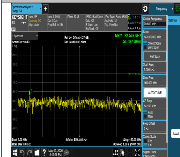
Band V-4233-0.009~0.15MHz-PASS
