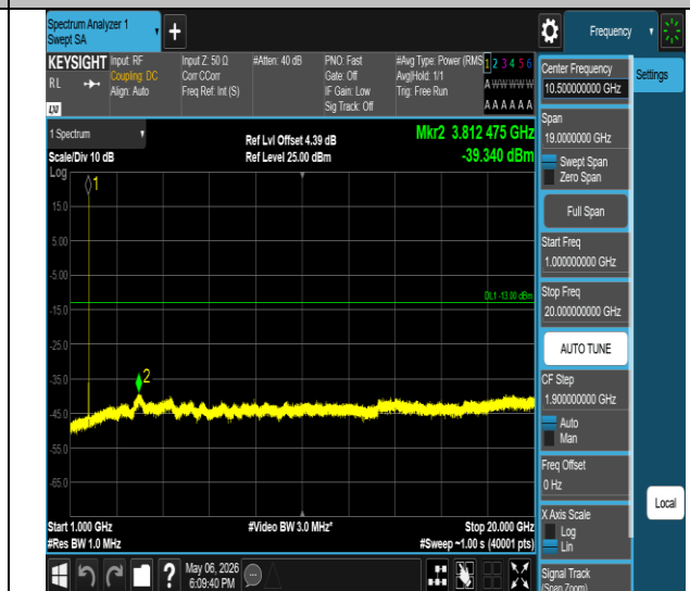
Band IV-1513-1000~20000MHz-PASS
