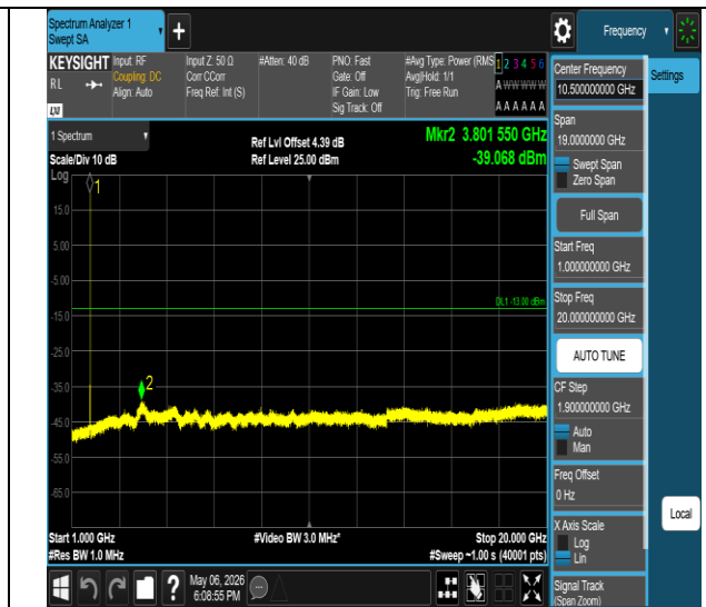
Band IV-1413-1000~20000MHz-PASS
