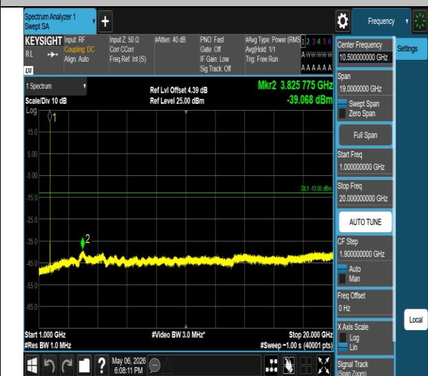
Band IV-1312-1000~20000MHz-PASS
