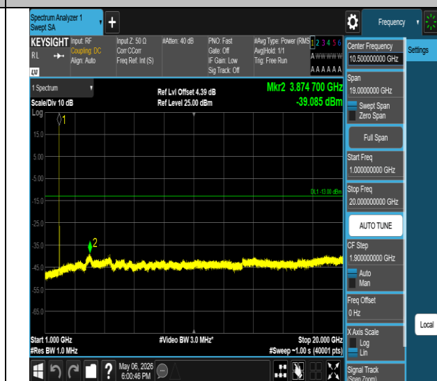
Band II-9538-1000~20000MHz-PASS
