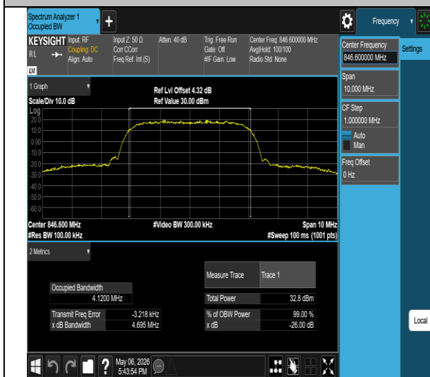
Band V-4233-PASS
