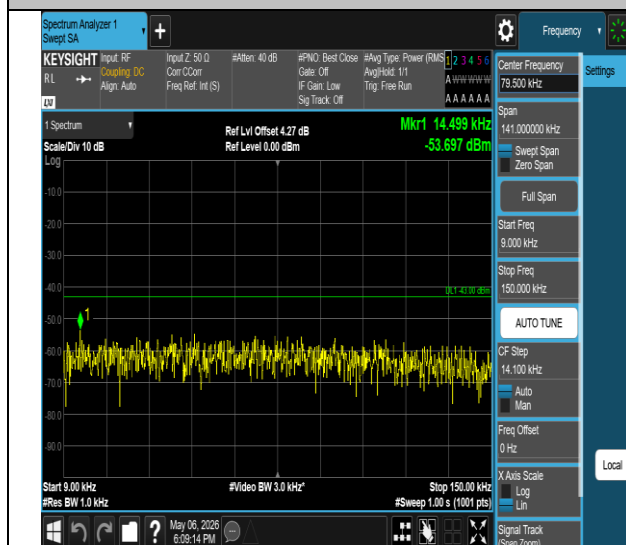
Band IV-1513-0.009~0.15MHz-PASS
