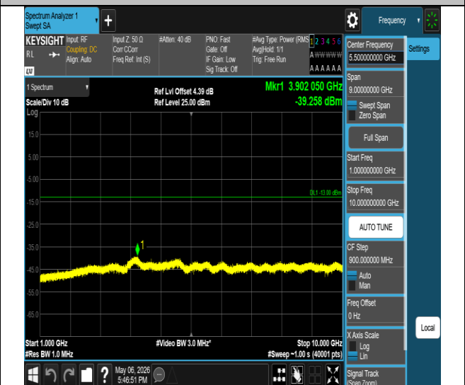
Band V-4233-1000~10000MHz-PASS
