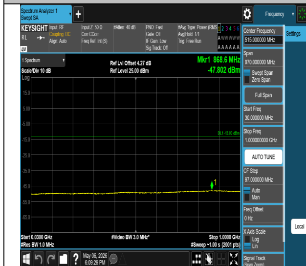
Band IV-1513-30~1000MHz-PASS
