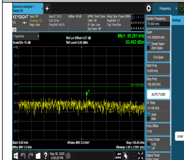
Band IV-1413-0.009~0.15MHz-PASS
