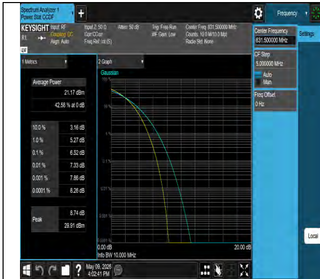
Band26(824-849)-15MHz-64QAM-26865-75RB#0-PASS
