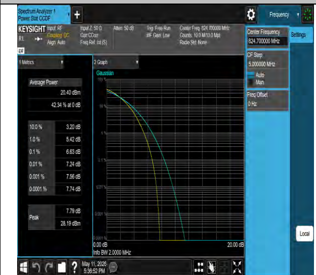
Band26(824-849)-1.4MHz-256QAM-26797-6RB#0-PASS
