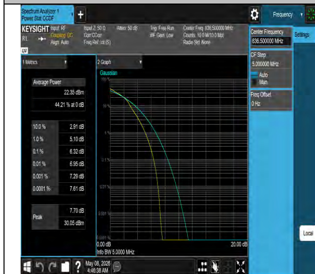
Band26(824-849)-5MHz-16QAM-26915-25RB#0-PASS
