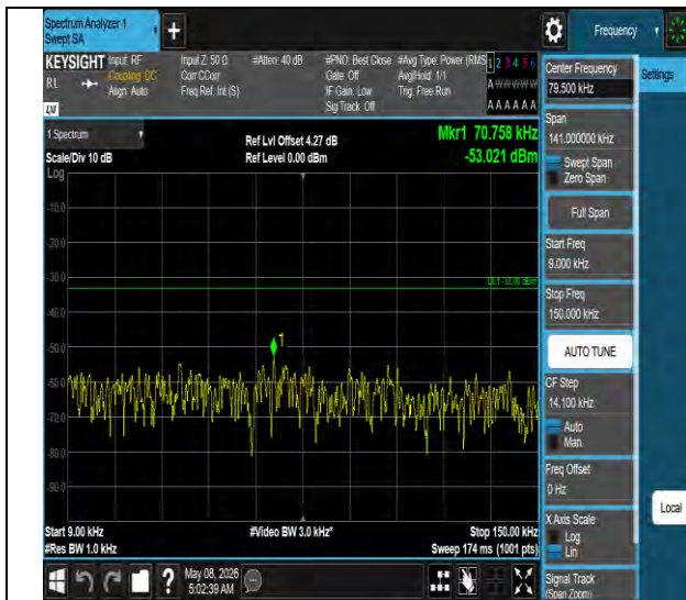
Band26(824-849)-15MHz-QPSK-26965-1RB#0-0.009~0.15-PASS
