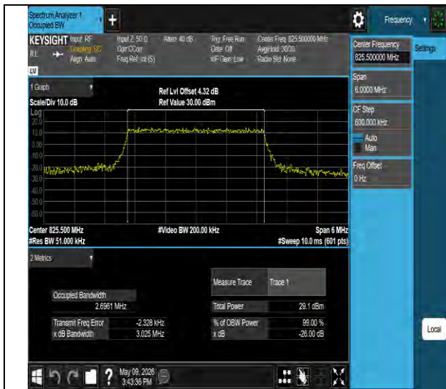
Band26(824-849)-3MHz-64QAM-26805-15RB#0-PASS
