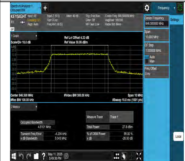
Band26(824-849)-5MHz-256QAM-27015-25RB#0-PASS
