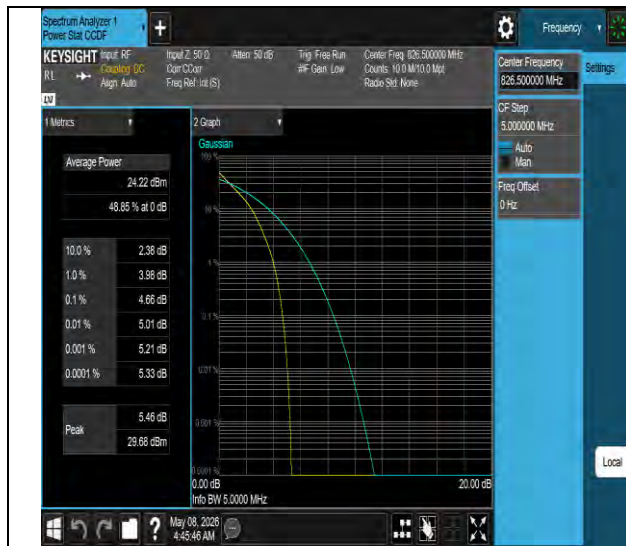
Band26(824-849)-5MHz-QPSK-26815-25RB#0-PASS
