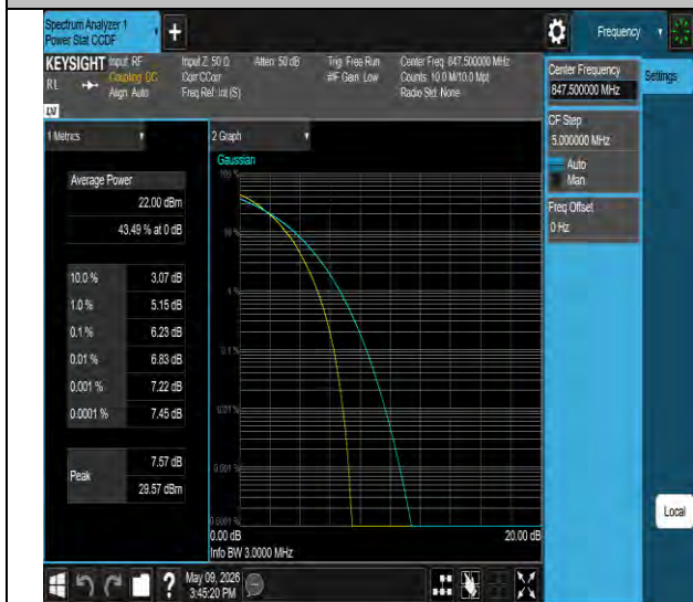
Band26(824-849)-3MHz-64QAM-27025-15RB#0-PASS
