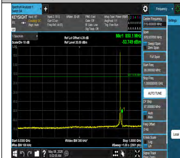
Band26(824-849)-15MHz-QPSK-26965-1RB#0-30~1000-PASS
