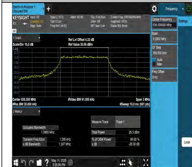
Band26(824-849)-1.4MHz-256QAM-26915-6RB#0-PASS
