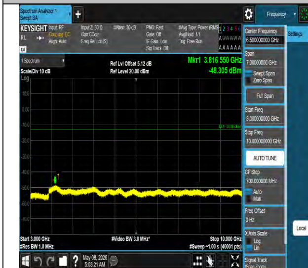
Band26(824-849)-15MHz-QPSK-26965-1RB#0-3000~10000- PASS
