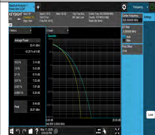
Band26(824-849)-3MHz-256QAM-26805-15RB#0-PASS
