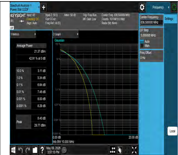
Band26(824-849)-10MHz-64QAM-26915-50RB#0-PASS
