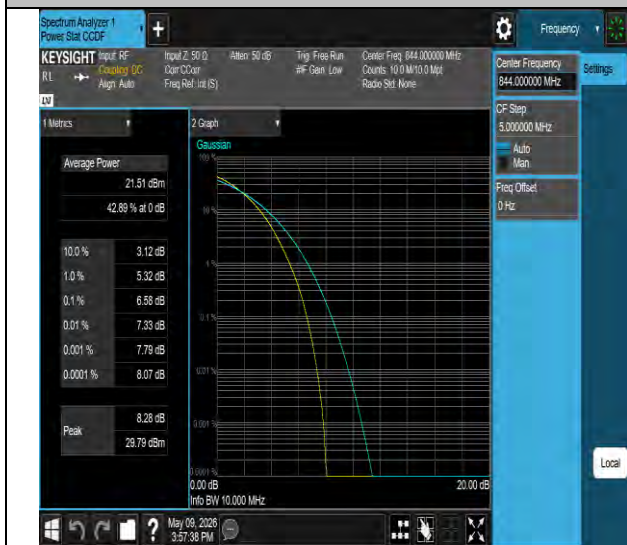
Band26(824-849)-10MHz-64QAM-26990-50RB#0-PASS
