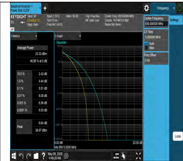
Band26(824-849)-5MHz-QPSK-26915-25RB#0-PASS
