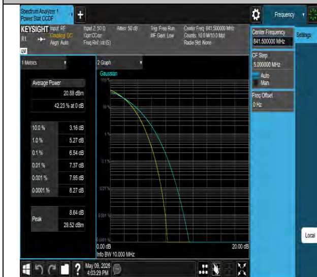
Band26(824-849)-15MHz-64QAM-26965-75RB#0-PASS
