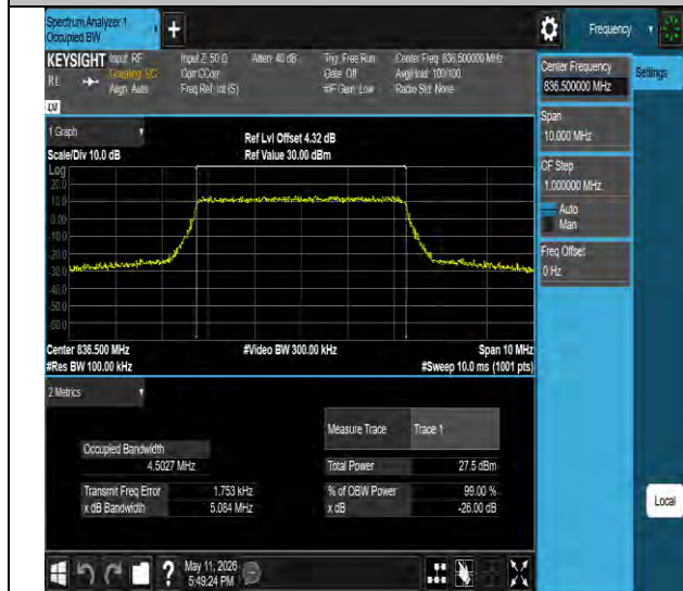
Band26(824-849)-5MHz-256QAM-26915-25RB#0-PASS
