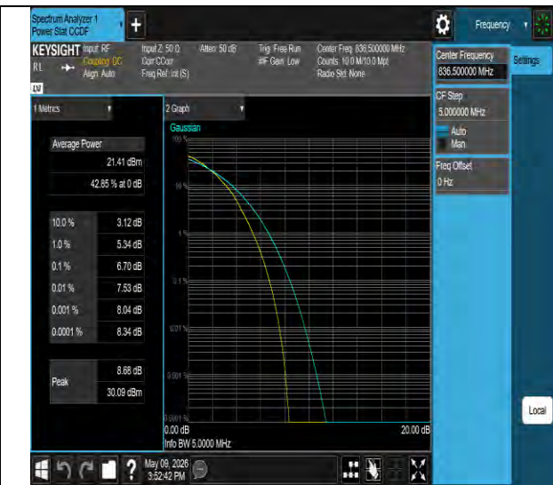
Band26(824-849)-5MHz-64QAM-26915-25RB#0-PASS
