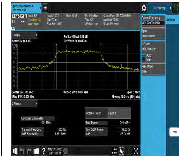
Band26(824-849)-1.4MHz-64QAM-26797-6RB#0-PASS
