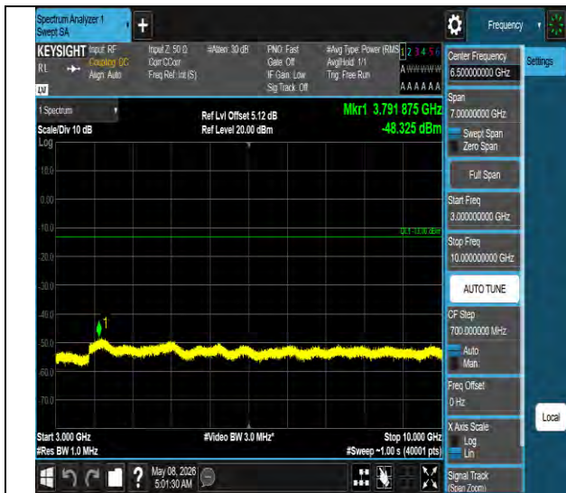
Band26(824-849)-15MHz-QPSK-26865-1RB#0-3000~10000-PASS
