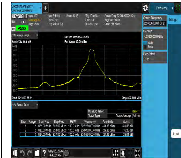
Band26(824-849)-10MHz-QPSK-26840-1RB#0-PASS
