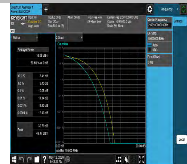
Band41-10MHz-256QAM-39700-50RB#0-PASS
