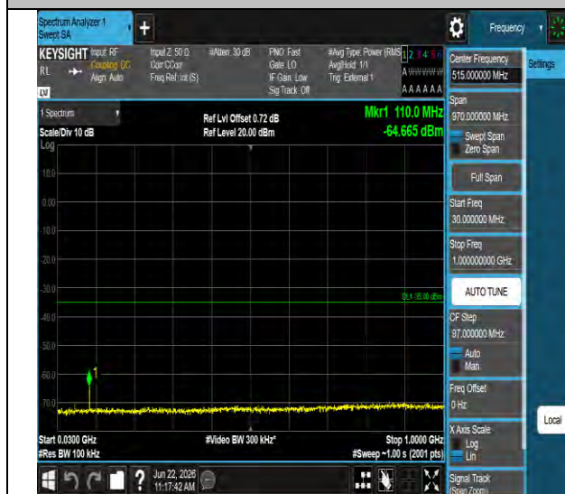
Band41-20MHz-QPSK-41490-1RB#0-30~1000-PASS
