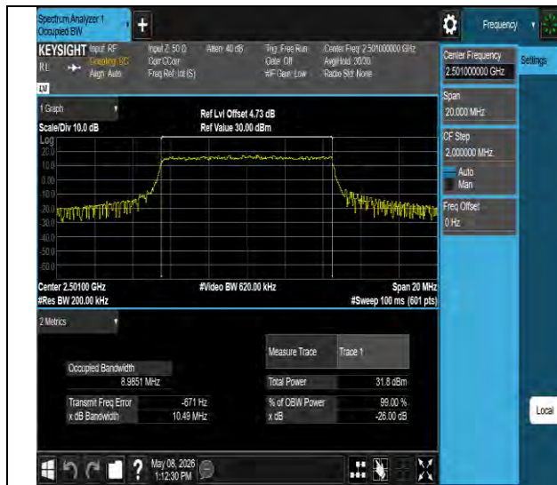
Band41-10MHz-QPSK-39700-50RB#0-PASS
