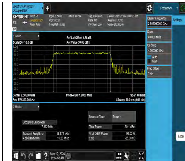
Band41-20MHz-64QAM-39750-100RB#0-PASS
