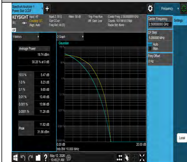
Band41-10MHz-16QAM-40620-50RB#0-PASS
