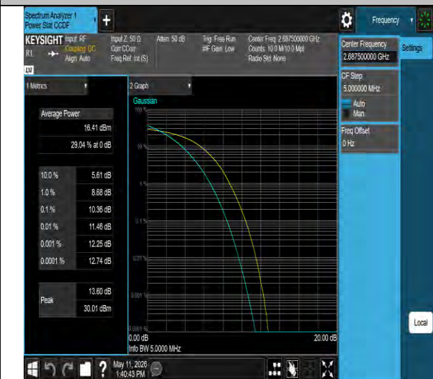
Band41-5MHz-256QAM-41565-25RB#0-PASS
