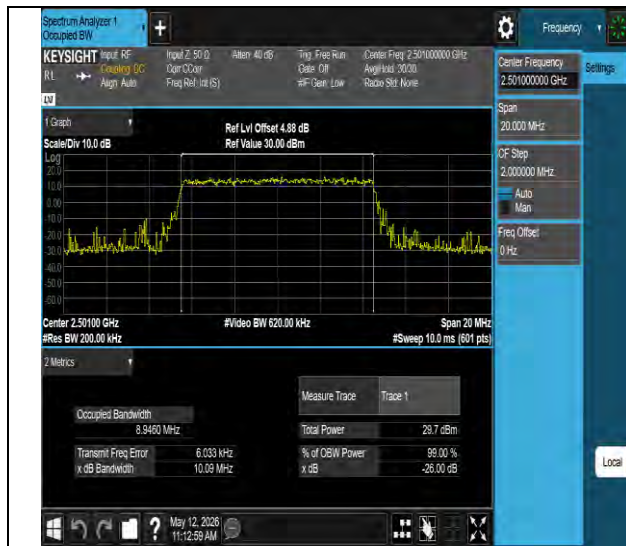
Band41-10MHz-64QAM-39700-50RB#0-PASS
