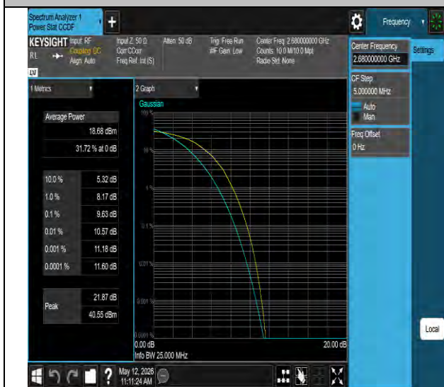
Band41-20MHz-64QAM-41490-100RB#0-PASS
