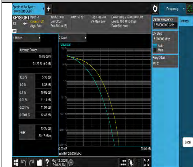
Band41-20MHz-256QAM-40620-100RB#0-PASS
