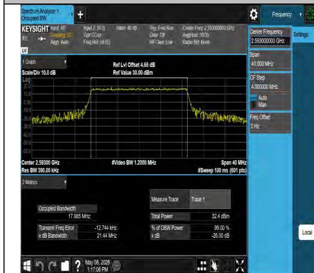
Band41-20MHz-16QAM-40620-100RB#0-PASS
