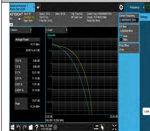
Band41-10MHz-64QAM-41540-50RB#0-PASS
