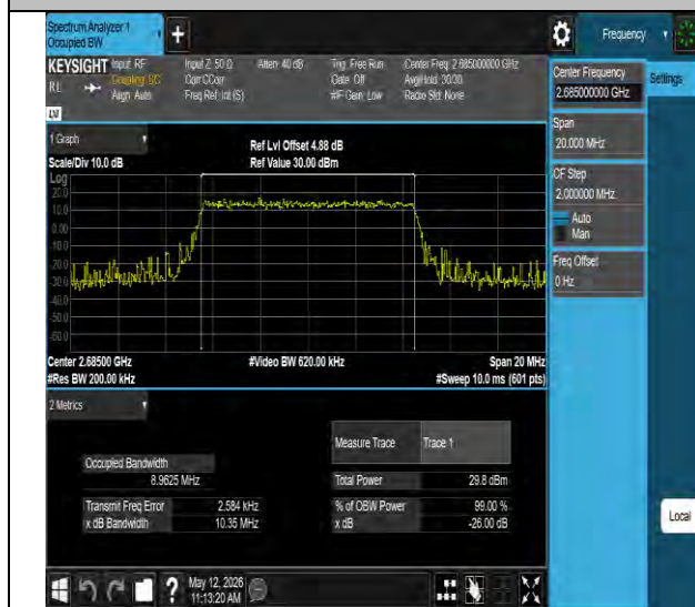
Band41-10MHz-64QAM-41540-50RB#0-PASS
