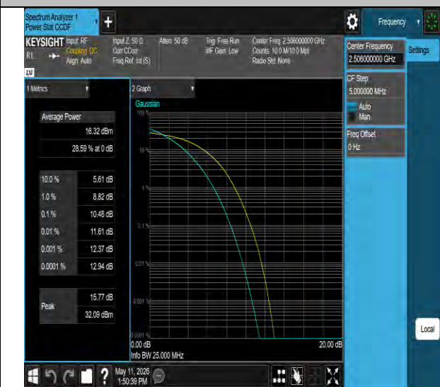
Band41-20MHz-256QAM-39750-100RB#0-PASS
