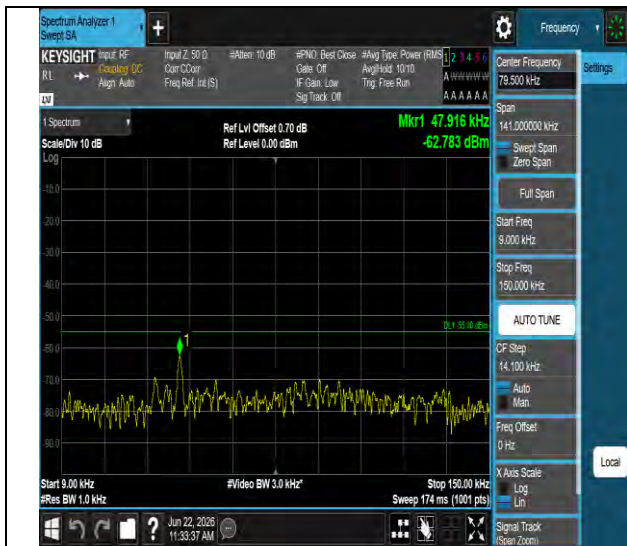
Band41-20MHz-QPSK-40620-1RB#0-0.009~0.15-PASS
