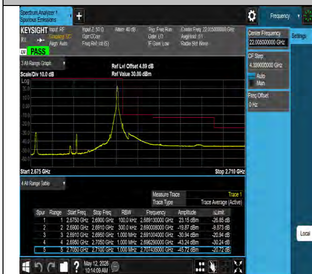
Band41-15MHz-QPSK-41515-1RB#74-PASS
