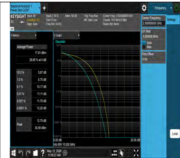
Band41-15MHz-64QAM-40620-75RB#0-PASS
