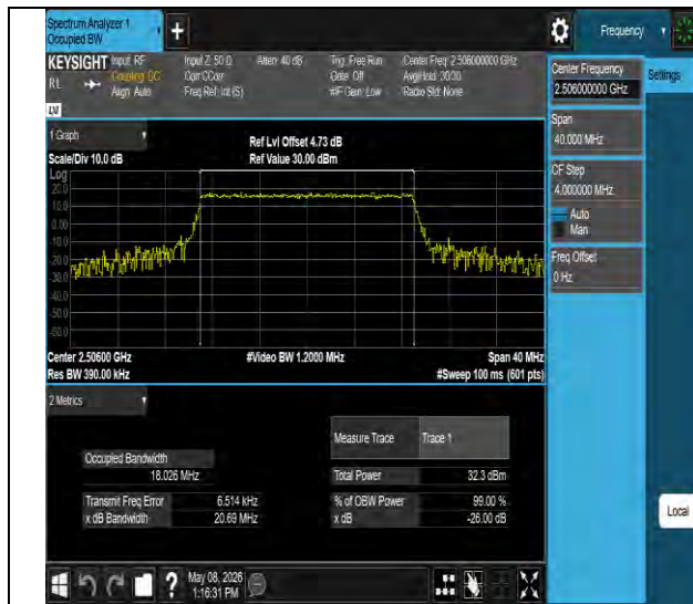
Band41-20MHz-QPSK-39750-100RB#0-PASS
