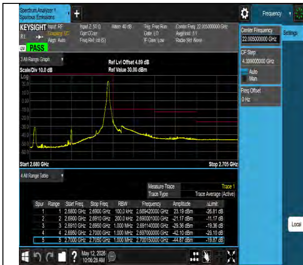
Band41-10MHz-QPSK-41540-1RB#49-PASS
