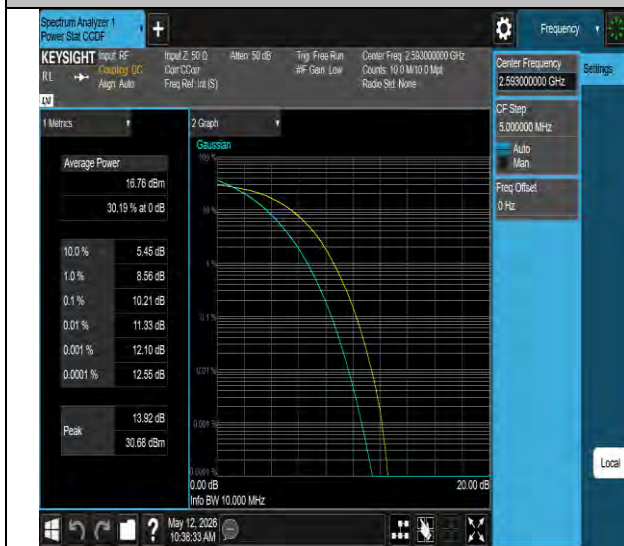
Band41-10MHz-256QAM-40620-50RB#0-PASS
