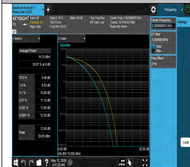
Band41-15MHz-256QAM-40620-75RB#0-PASS
