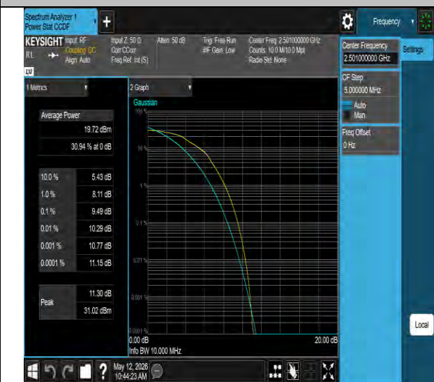
Band41-10MHz-16QAM-39700-50RB#0-PASS
