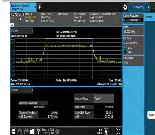
Band41-10MHz-256QAM-40620-50RB#0-PASS
