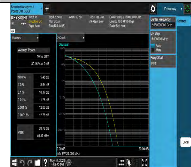
Band41-20MHz-256QAM-41490-100RB#0-PASS
