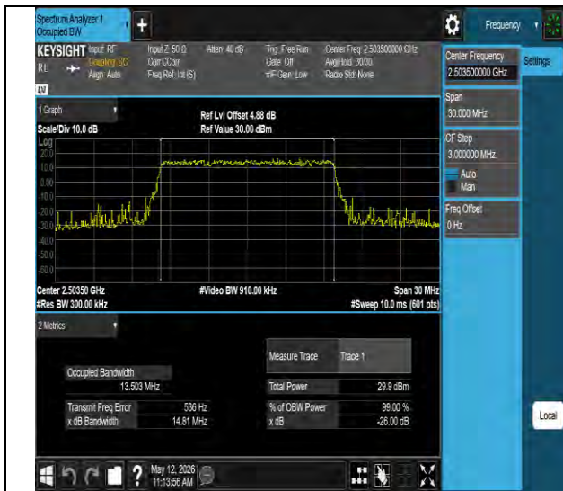
Band41-15MHz-64QAM-39725-75RB#0-PASS
