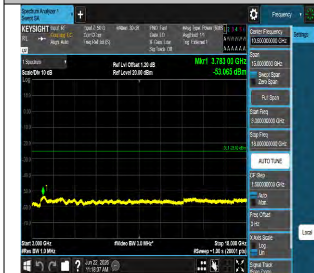
Band41-20MHz-QPSK-41490-1RB#0-3000~18000-PASS
