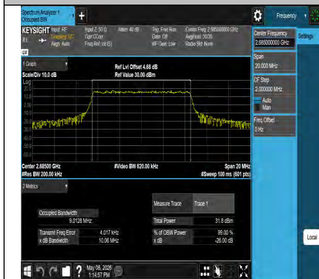
Band41-10MHz-QPSK-41540-50RB#0-PASS
