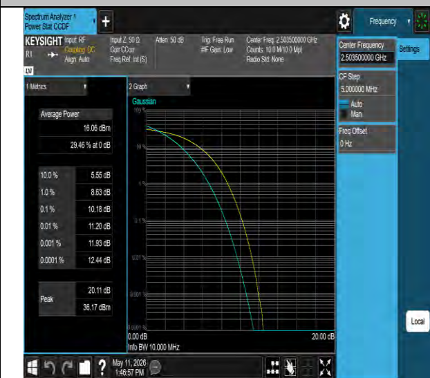
Band41-15MHz-256QAM-39725-75RB#0-PASS
