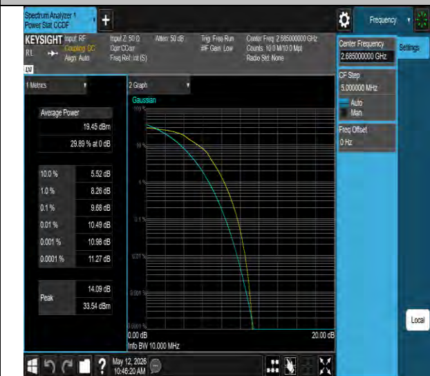
Band41-10MHz-16QAM-41540-50RB#0-PASS
