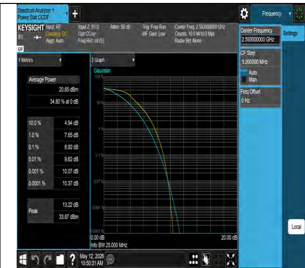
Band41-20MHz-QPSK-40620-100RB#0-PASS
