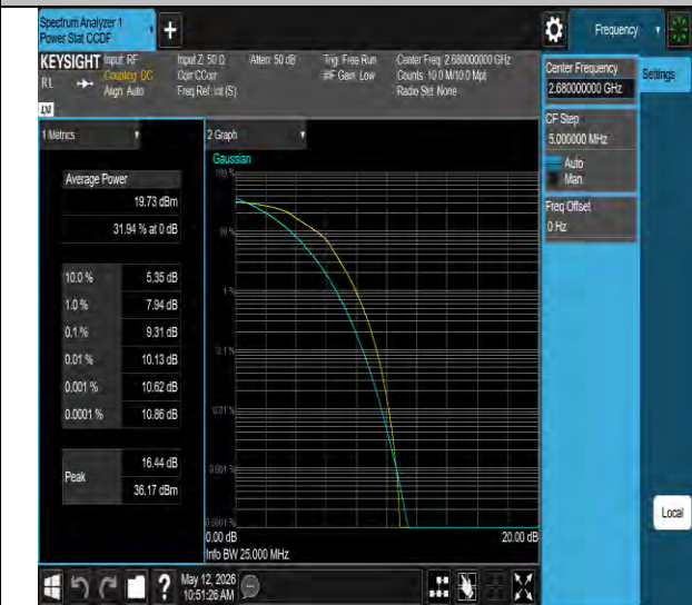
Band41-20MHz-16QAM-41490-100RB#0-PASS
