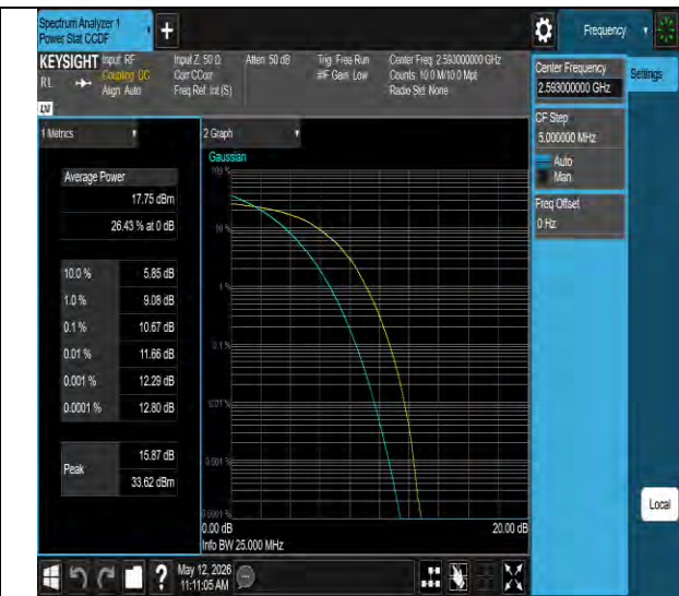
Band41-20MHz-64QAM-40620-100RB#0-PASS
