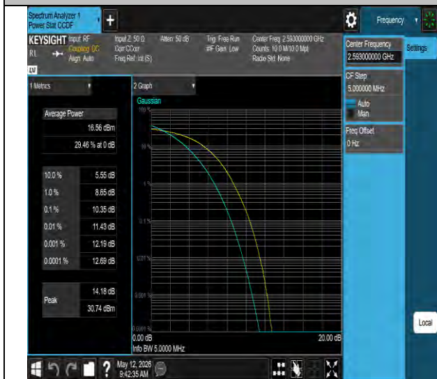
Band41-5MHz-256QAM-40620-25RB#0-PASS
