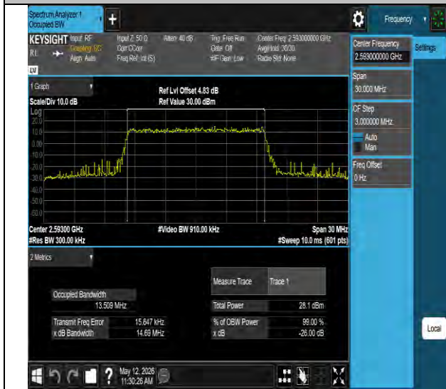
Band41-15MHz-256QAM-40620-75RB#0-PASS
