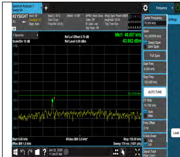
Band41-20MHz-QPSK-41490-1RB#0-0.009~0.15-PASS
