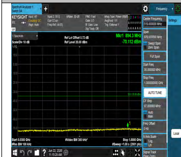
Band41-20MHz-QPSK-40620-1RB#0-30~1000-PASS
