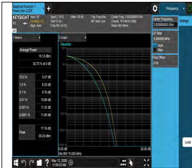
Band41-15MHz-64QAM-39725-75RB#0-PASS
