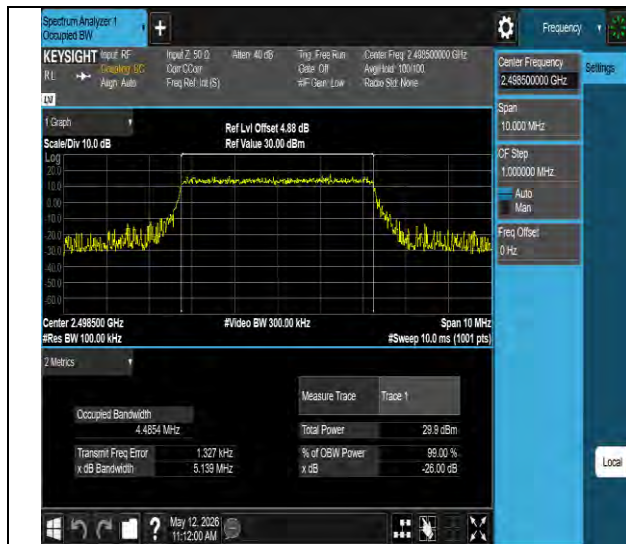
Band41-5MHz-64QAM-39675-25RB#0-PASS
