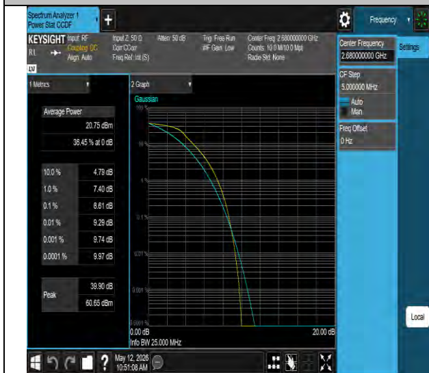
Band41-20MHz-QPSK-41490-100RB#0-PASS
