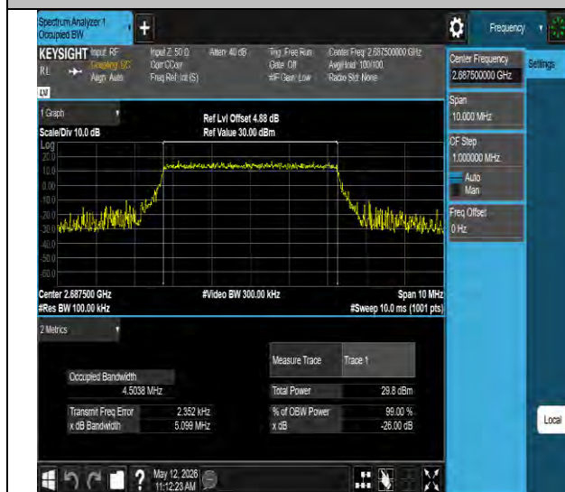
Band41-5MHz-64QAM-41565-25RB#0-PASS
