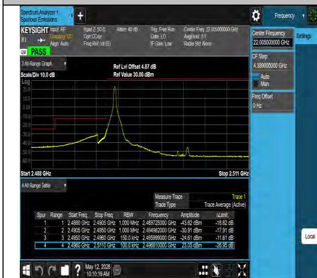
Band41-15MHz-QPSK-39725-1RB#0-PASS
