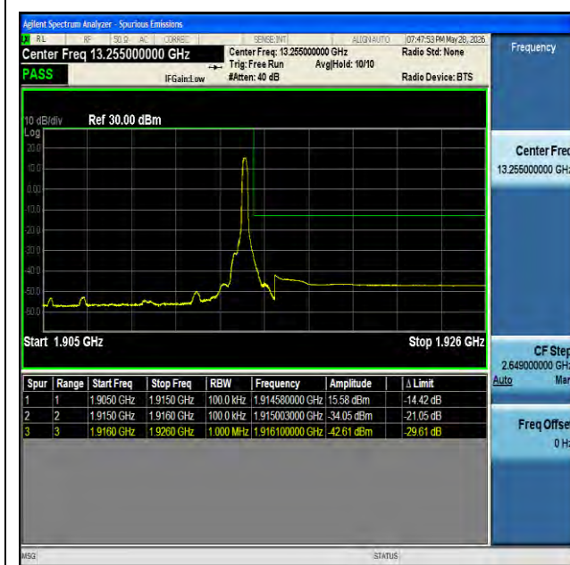
NTNV-n25-PC3-15-10-H-CP-QPSK-Edge_1RB_Right-PASS
