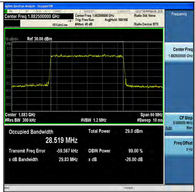
NTVN-n25-PC3-15-30-M-DFT-256QAM-Outer_Full-Ant1-PASS
