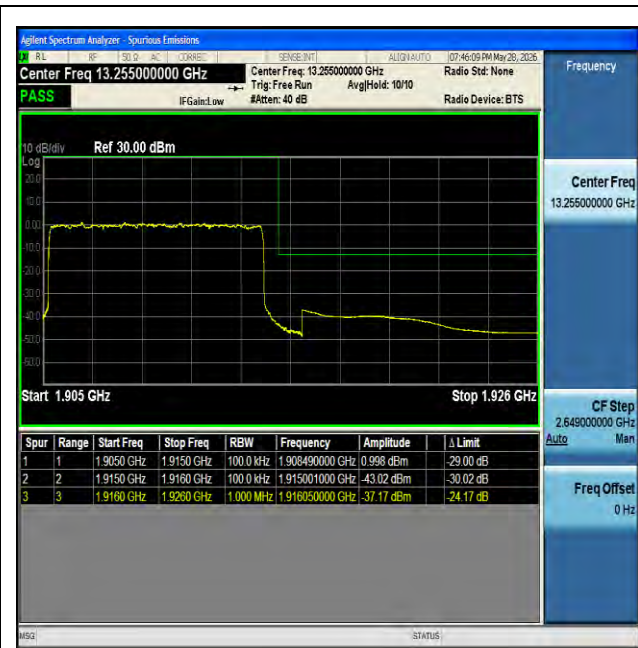
NTNV-n25-PC3-15-10-H-DFT-BPSK-Outer_Full-PASS
