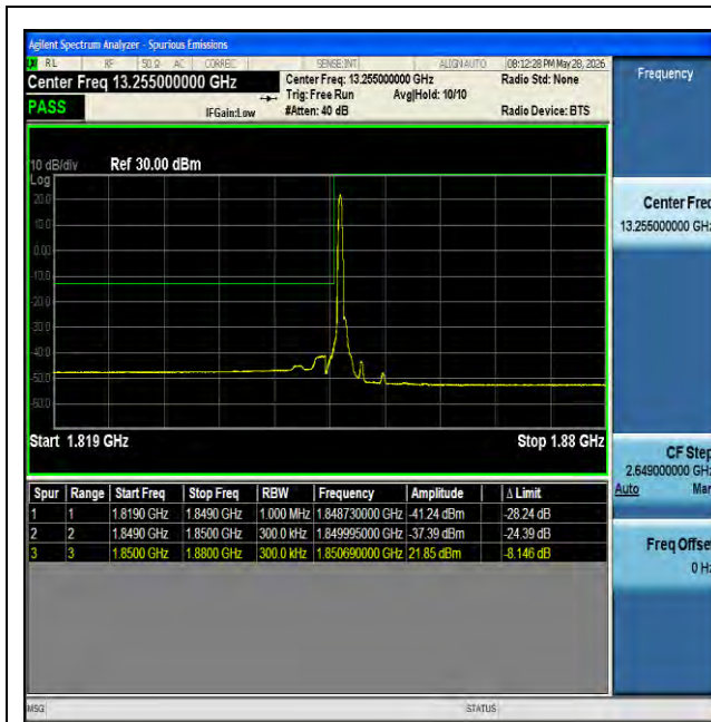
NTNV-n25-PC3-15-30-L-DFT-BPSK-Edge_1RB_Left-PASS
