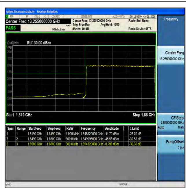
NTNV-n25-PC3-15-30-L-DFT-BPSK-Outer_Full-PASS
