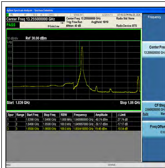
NTNV-n25-PC3-15-10-L-DFT-BPSK-Edge_1RB_Left-PASS
