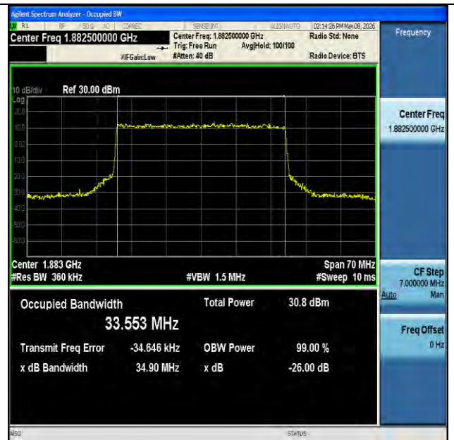
NTNV-n25-PC3-15-35-M-CP-QPSK-Outer_Full-Ant1-PASS
