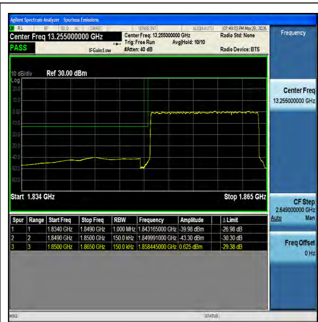
NTNV-n25-PC3-15-15-L-DFT-BPSK-Outer_Full-PASS
