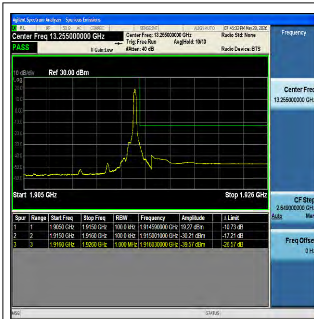
NTNV-n25-PC3-15-10-H-DFT-BPSK-Edge_1RB_Right-PASS
