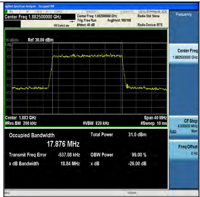
NTVN-n25-PC3-15-20-M-DFT-64QAM-Outer_Full-Ant1-PASS
