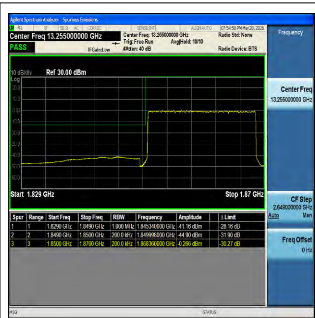
NTNV-n25-PC3-15-20-L-DFT-BPSK-Outer_Full-PASS
