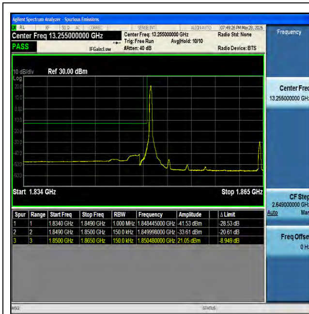
NTNV-n25-PC3-15-15-L-DFT-BPSK-Edge_1RB_Left-PASS
