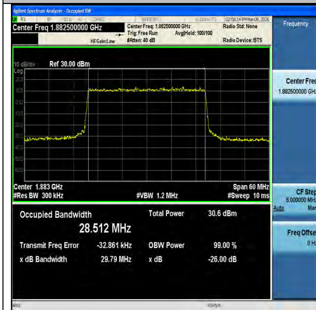
NTVN-n25-PC3-15-30-M-CP-QPSK-Outer_Full-Ant1-PASS
