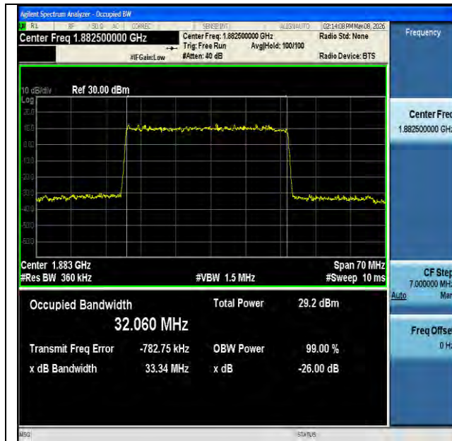
NTNV-n25-PC3-15-35-M-DFT-256QAM-Outer_Full-Ant1-PASS
