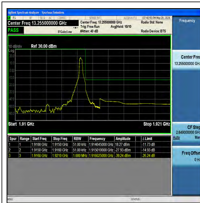
NTNV-n25-PC3-15-5-H-DFT-BPSK-Edge_1RB_Right-PASS
