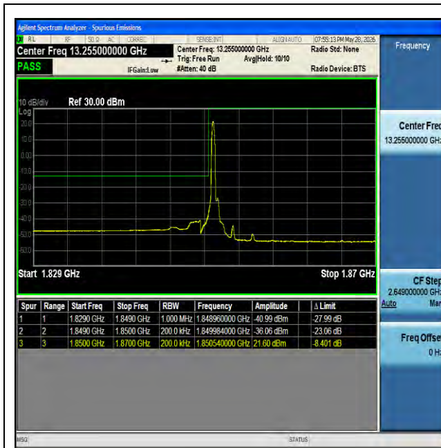
NTNV-n25-PC3-15-20-L-DFT-BPSK-Edge_1RB_Left-PASS
