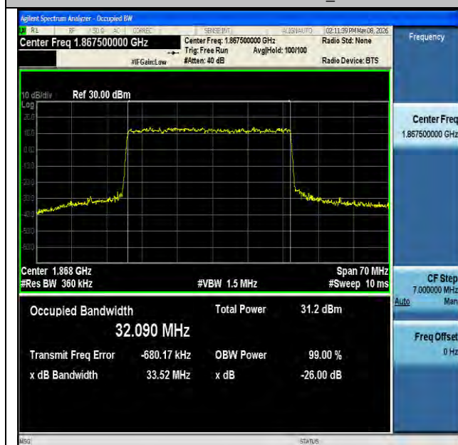
NTNV-n25-PC3-15-35-L-DFT-64QAM-Outer_Full-Ant1-PASS
