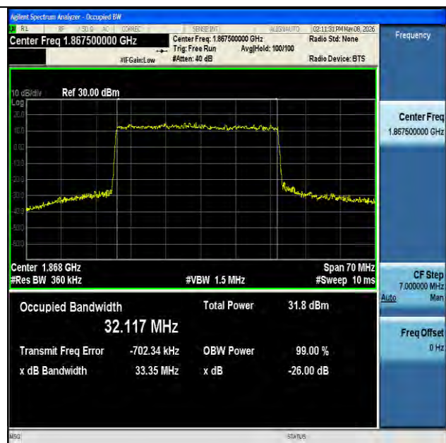
NTNV-n25-PC3-15-35-L-DFT-16QAM-Outer_Full-Ant1-PASS
