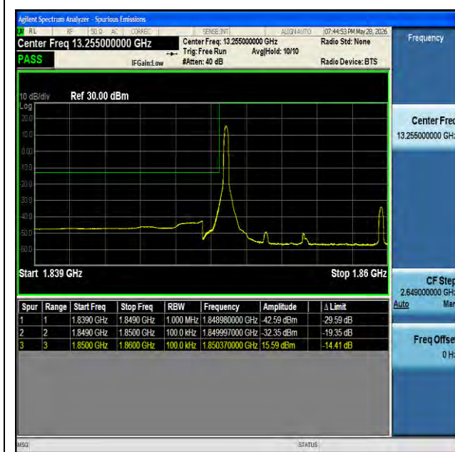
NTNV-n25-PC3-15-10-L-CP-QPSK-Edge_1RB_Left-PASS
