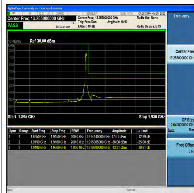
NTNV-n25-PC3-15-20-H-CP-QPSK-Edge_1RB_Right-PASS
