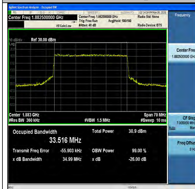
NTNV-n25-PC3-15-35-M-CP-16QAM-Outer_Full-Ant1-PASS
