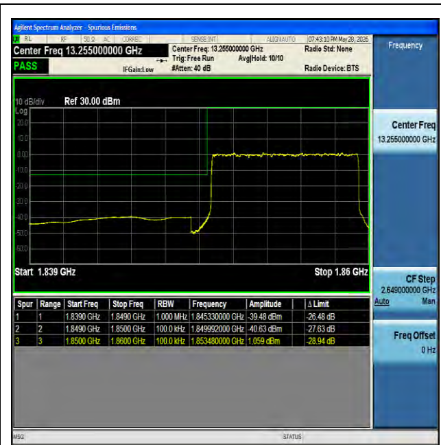
NTNV-n25-PC3-15-10-L-DFT-BPSK-Outer_Full-PASS
