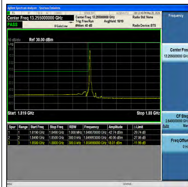
NTNV-n25-PC3-15-30-L-CP-QPSK-Edge_1RB_Left-PASS
