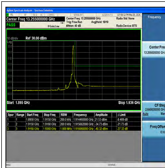
NTNV-n25-PC3-15-20-H-DFT-BPSK-Edge_1RB_Right-PASS
