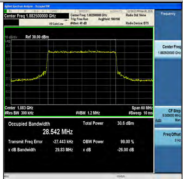
NTVN-n25-PC3-15-30-M-CP-16QAM-Outer_Full-Ant1-PASS
