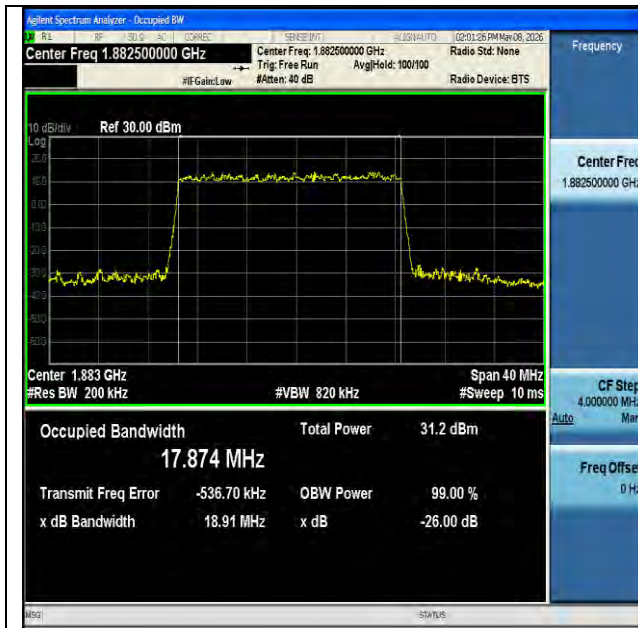
NTVN-n25-PC3-15-20-M-DFT-16QAM-Outer_Full-Ant1-PASS
