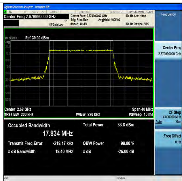
NTNV-n41-PC2-30-20-H-DFT-QPSK-Outer_Full-Ant1-PASS
