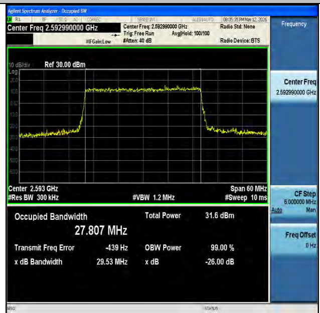
NTVN-n41-PC2-30-30-M-CP-QPSK-Outer_Full-Ant1-PASS
