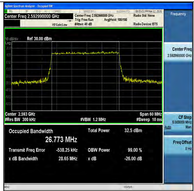
NTVN-n41-PC2-30-30-M-DFT-64QAM-Outer_Full-Ant1-PASS
