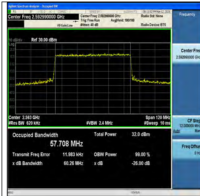
NTNV-n41-PC2-30-60-M-CP-QPSK-Outer_Full-Ant1-PASS
