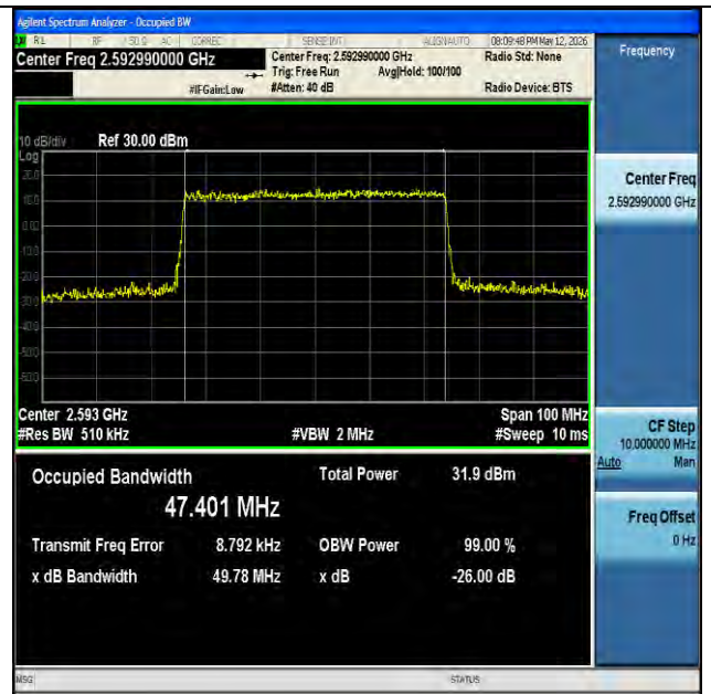
NTNV-n41-PC2-30-50-M-CP-QPSK-Outer_Full-Ant1-PASS
