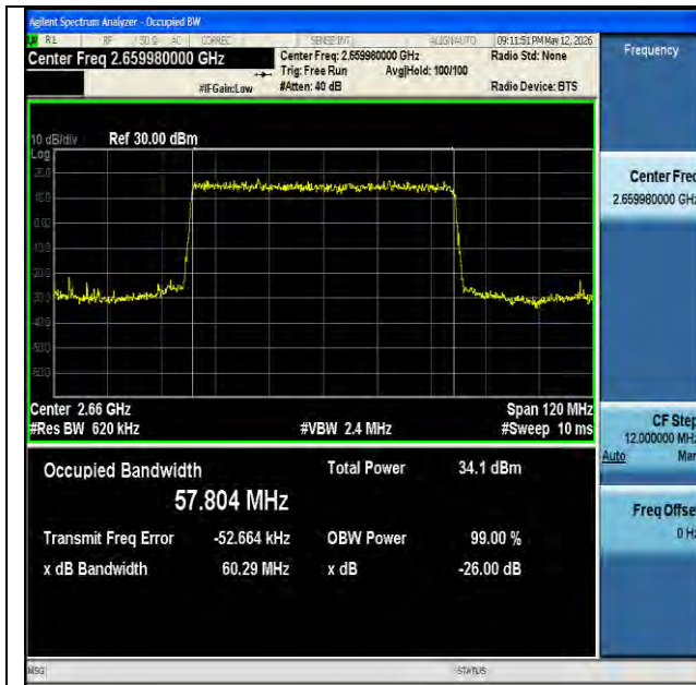
NTNV-n41-PC2-30-60-H-DFT-BPSK-Outer_Full-Ant1-PASS
