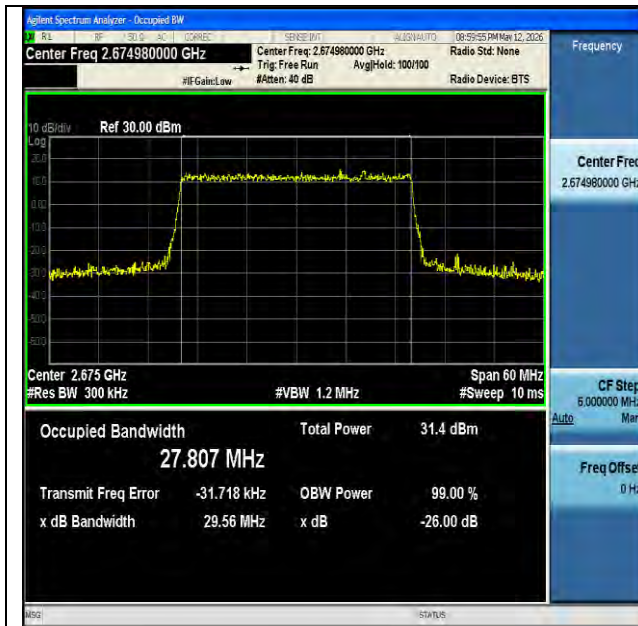
NTNV-n41-PC2-30-30-H-CP-QPSK-Outer_Full-Ant1-PASS
