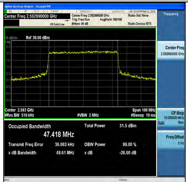
NTNV-n41-PC2-30-50-M-CP-64QAM-Outer_Full-Ant1-PASS
