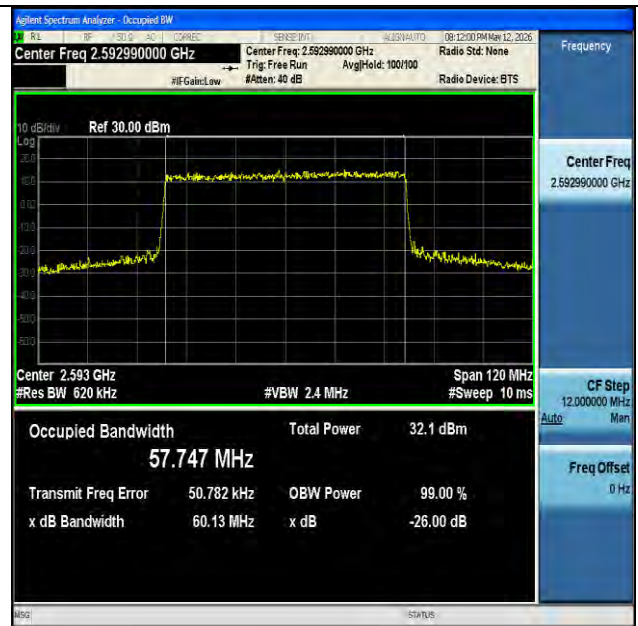
NTNV-n41-PC2-30-60-M-CP-16QAM-Outer_Full-Ant1-PASS
