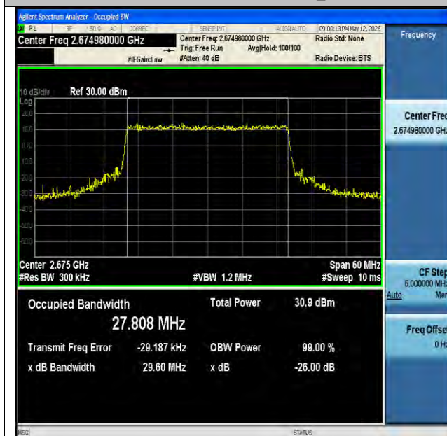
NTNV-n41-PC2-30-30-H-CP-64QAM-Outer_Full-Ant1-PASS
