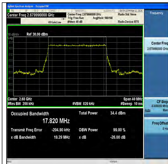
NTNV-n41-PC2-30-20-H-DFT-BPSK-Outer_Full-Ant1-PASS
