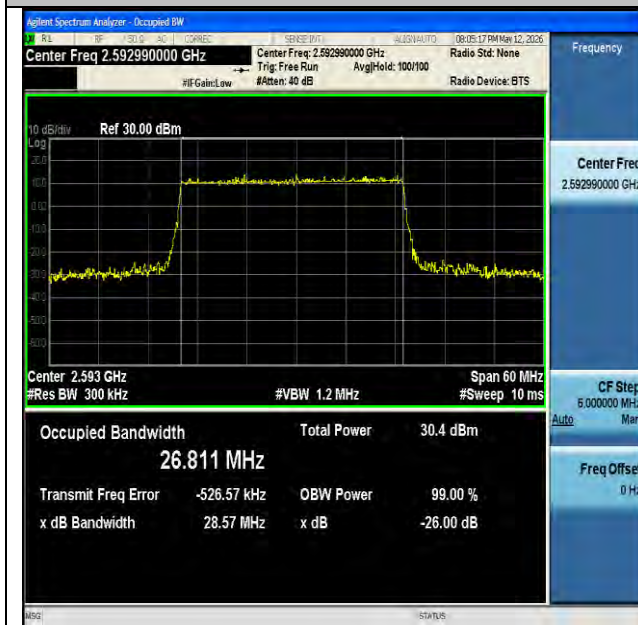
NTVN-n41-PC2-30-30-M-DFT-256QAM-Outer_Full-Ant1-PASS
