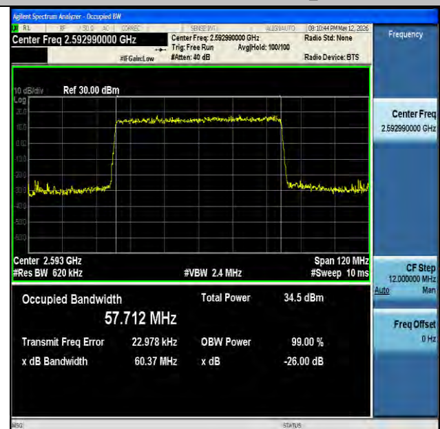
NTNV-n41-PC2-30-60-M-DFT-BPSK-Outer_Full-Ant1-PASS
