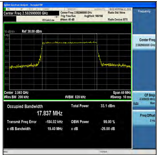
NTNV-n41-PC2-30-20-M-DFT-16QAM-Outet_Full-Ant1-PASS
