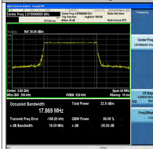
NTNV-n41-PC2-30-20-H-DFT-16QAM-Outer_Full-Ant1-PASS
