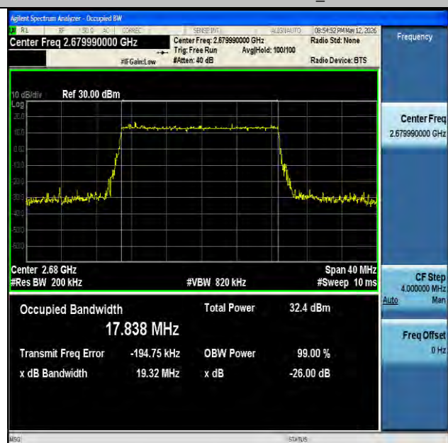
NTNV-n41-PC2-30-20-H-DFT-64QAM-Outer_Full-Ant1-PASS
