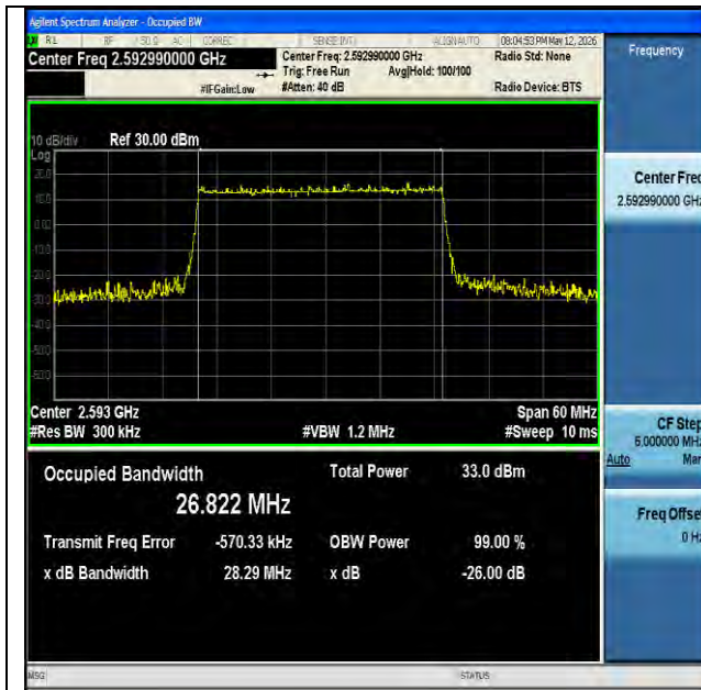
NTVN-n41-PC2-30-30-M-DFT-16QAM-Outer_Full-Ant1-PASS
