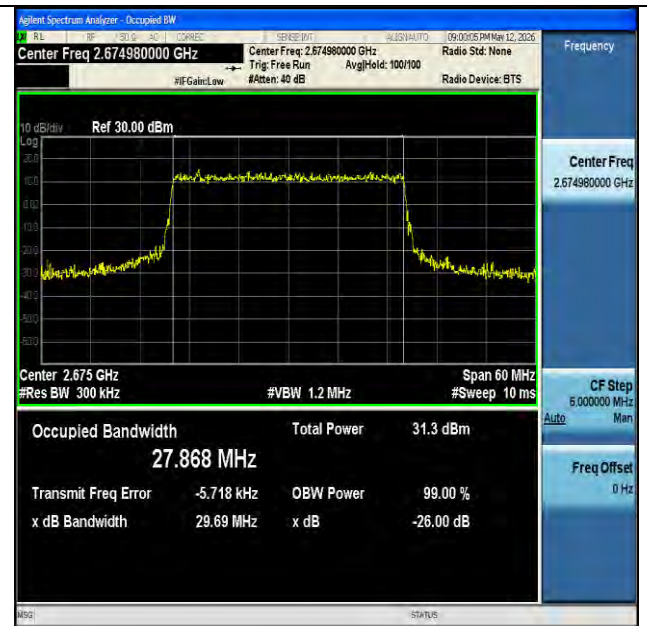
NTNV-n41-PC2-30-30-H-CP-16QAM-Outer_Full-Ant1-PASS
