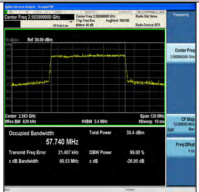
NTNV-n41-PC2-30-60-M-DFT-256QAM-Outer_Full-Ant1-PASS
