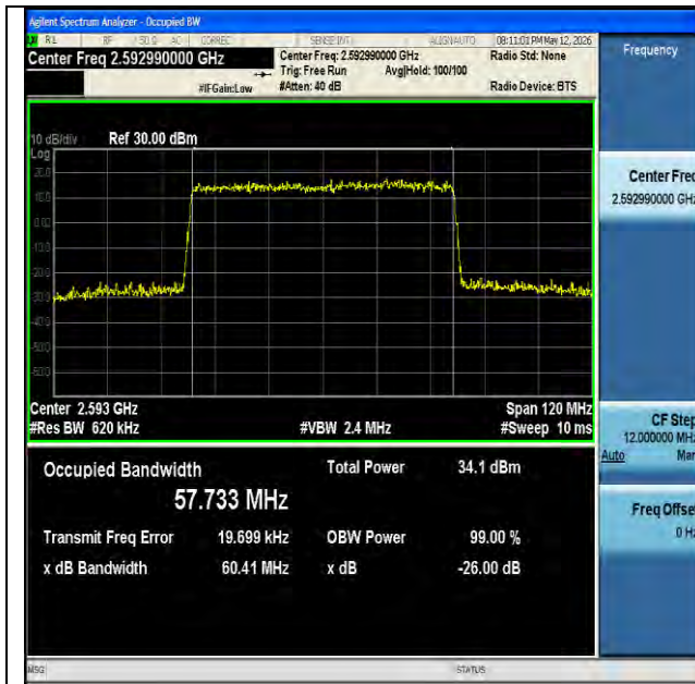
NTNV-n41-PC2-30-60-M-DFT-QPSK-Outer_Full-Ant1-PASS
