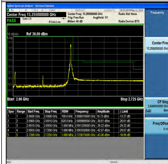
NTNV-n41-PC2-30-30-H-CP-QPSK-Edge_1RB_Right-PASS
