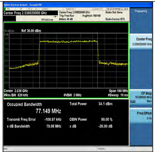
NTNV-n41-PC2-30-80-L-DFT-QPSK-Outer_Full-Ant1-PASS
