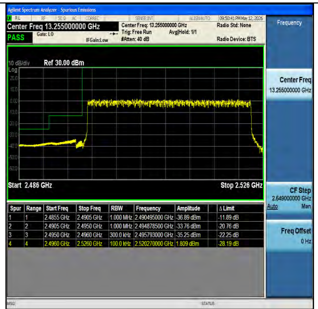
NTNV-n41-PC2-30-30-L-DFT-BPSK-Outer_Full-PASS
