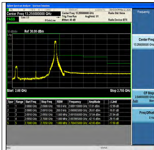
NTNV-n41-PC2-30-10-H-DFT-BPSK-Edge_1RB_Right-PASS
