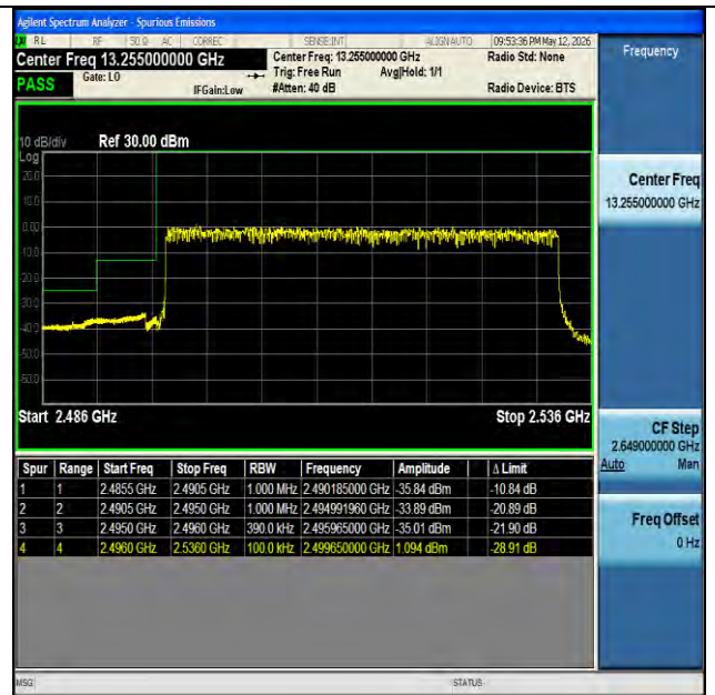
NTNV-n41-PC2-30-40-L-DFT-BPSK-Outer_Full-PASS
