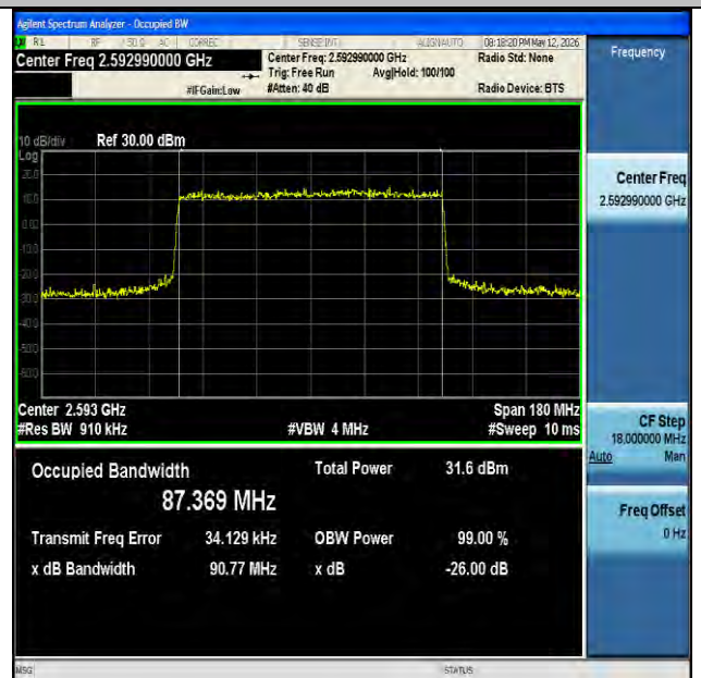
NTNV-n41-PC2-30-90-M-CP-64QAM-Outer_Full-Ant1-PASS
