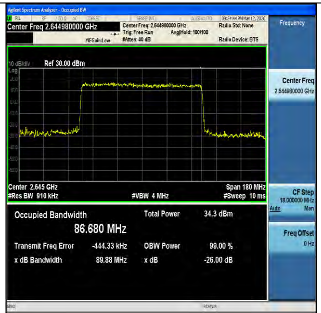
NTNV-n41-PC2-30-90-H-DFT-BPSK-Outer_Full-Ant1-PASS
