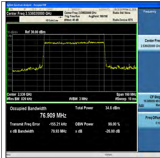
NTNV-n41-PC2-30-80-L-DFT-BPSK-Outer_Full-Ant1-PASS
