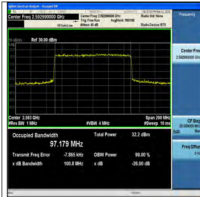
NTNV-n41-PC2-30-100-M-CP-QPSK-Outet_Full-Ant1-PASS
