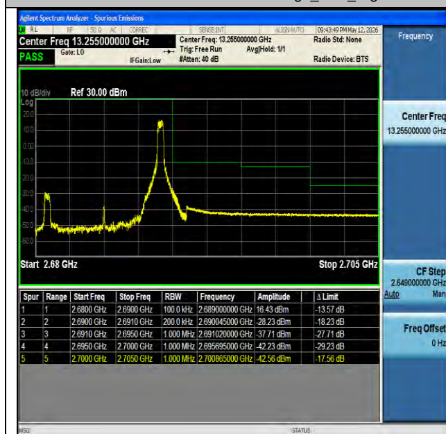
NTNV-n41-PC2-30-10-H-CP-QPSK-Edge_1RB_Right-PASS
