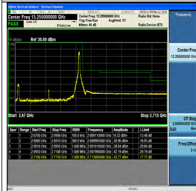
NTNV-n41-PC2-30-20-H-CP-QPSK-Edge_1RB_Right-PASS
