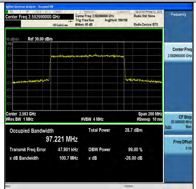
NTNV-n41-PC2-30-100-M-CP-256QAM-Outet_Full-Ant1-PASS
