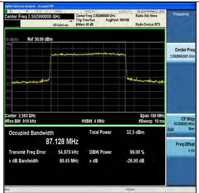
NTNV-n41-PC2-30-90-M-CP-QPSK-Outer_Full-Ant1-PASS
