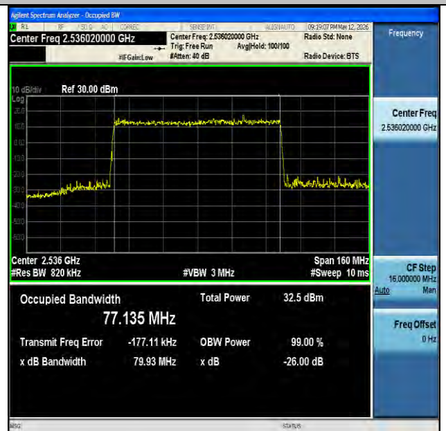
NTNV-n41-PC2-30-80-L-DFT-64QAM-Outer_Full-Ant1-PASS
