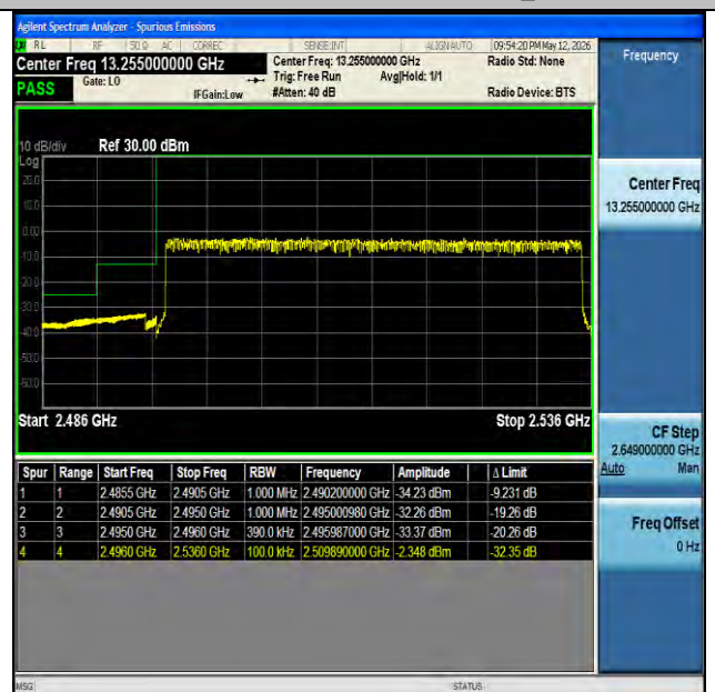
NTNV-n41-PC2-30-40-L-CP-QPSK-Outer_Full-PASS
