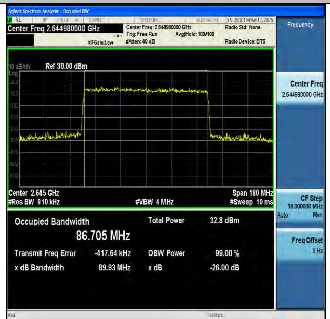
NTNV-n41-PC2-30-90-H-DFT-16QAM-Outer_Full-Ant1-PASS
