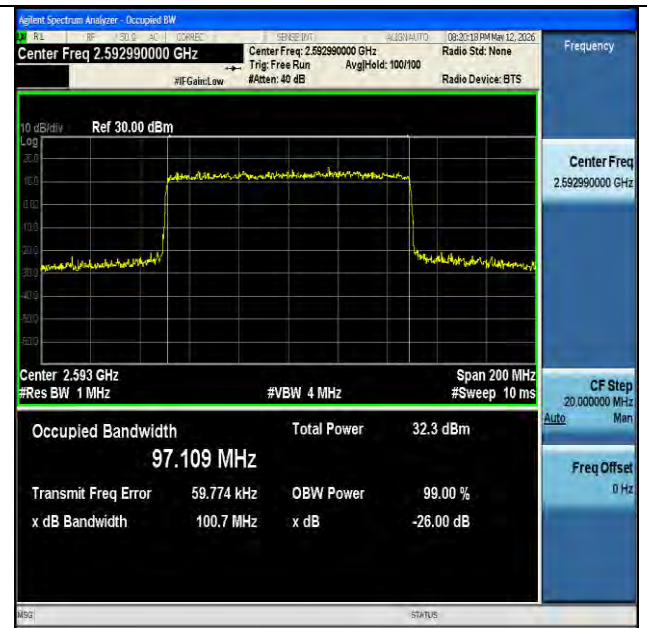
NTNV-n41-PC2-30-100-M-CP-16QAM-Outet_Full-Ant1-PASS
