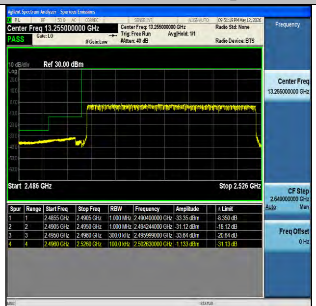
NTNV-n41-PC2-30-30-L-CP-QPSK-Outer_Full-PASS
