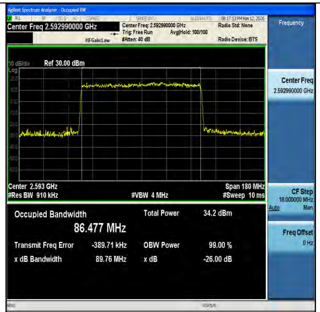
NTNV-n41-PC2-30-90-M-DFT-QPSK-Outer_Full-Ant1-PASS
