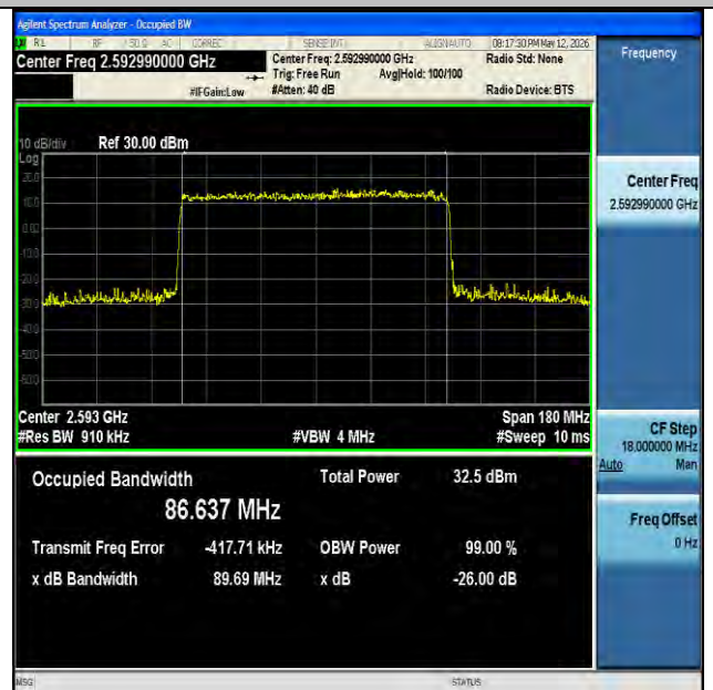
NTNV-n41-PC2-30-90-M-DFT-64QAM-Outer_Full-Ant1-PASS
