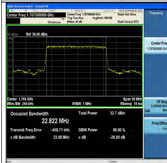
NTNV-n66-PC3-15-25-H-DFT-BPSK-Outer_Full-Ant1-PASS
