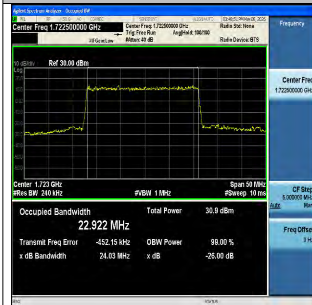
NTNV-n66-PC3-15-25-L-DFT-16QAM-Outer_Full-Ant1-PASS
