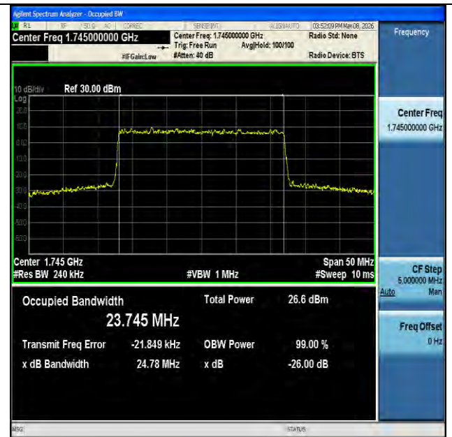
NTNV-n66-PC3-15-25-M-CP-256QAM-Outer_Full-Ant1-PASS
