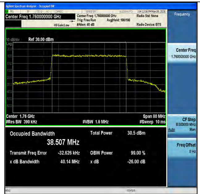
NTNV-n66-PC3-15-40-H-CP-16QAM-Outer_Full-Ant1-PASS
