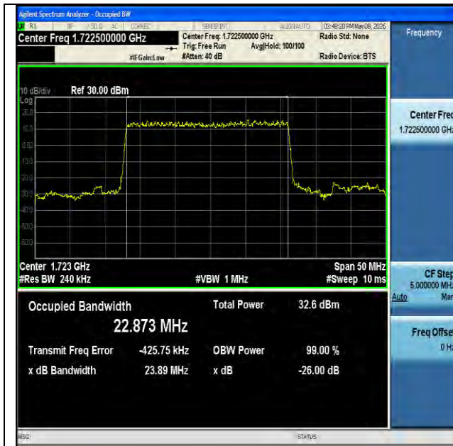
NTNV-n66-PC3-15-25-L-DFT-BPSK-Outer_Full-Ant1-PASS
