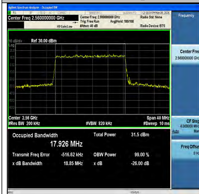
NTNV-n7-PC3-15-20-H-DFT-64QAM-Outer_Full-Ant1-PASS
