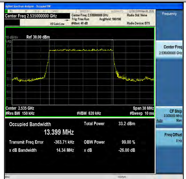
NTNV-n7-PC3-15-15-M-DFT-BPSK-Outer_Full-Ant1-PASS
