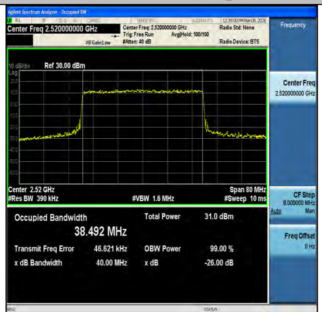
NTNV-n7-PC3-15-40-L-CP-16QAM-Outer_Full-Ant1-PASS
