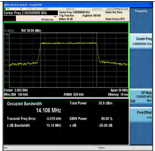
NTNV-n7-PC3-15-15-H-CP-QPSK-Outer_Full-Ant1-PASS
