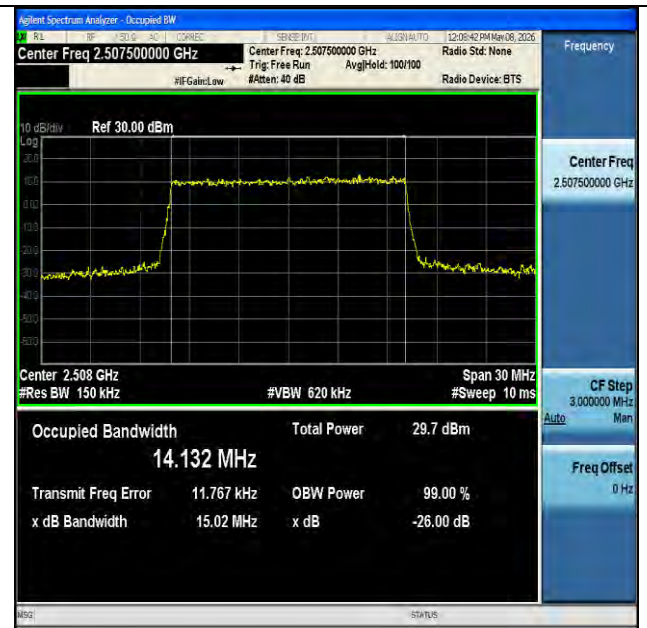
NTNV-n7-PC3-15-15-L-CP-64QAM-Outer_Full-Ant1-PASS
