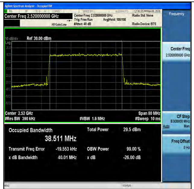
NTNV-n7-PC3-15-40-L-DFT-256QAM-Outer_Full-Ant1-PASS
