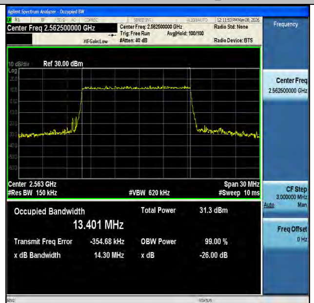
NTNV-n7-PC3-15-15-H-DFT-64QAM-Outer_Full-Ant1-PASS
