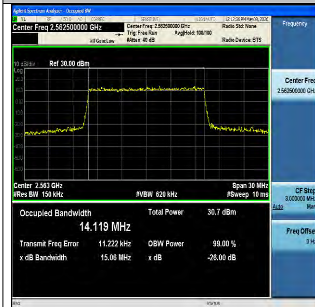
NTNV-n7-PC3-15-15-H-CP-16QAM-Outer_Full-Ant1-PASS
