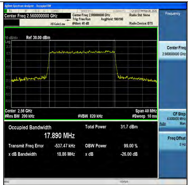
NTNV-n7-PC3-15-20-H-DFT-16QAM-Outer_Full-Ant1-PASS
