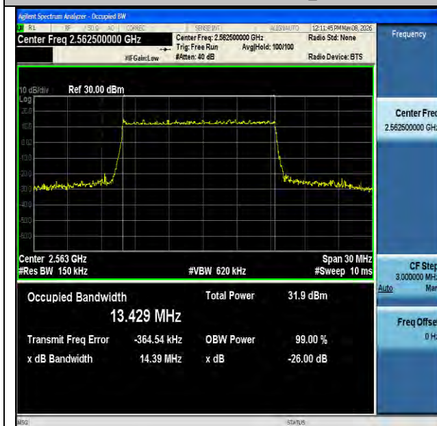
NTNV-n7-PC3-15-15-H-DFT-16QAM-Outer_Full-Ant1-PASS
