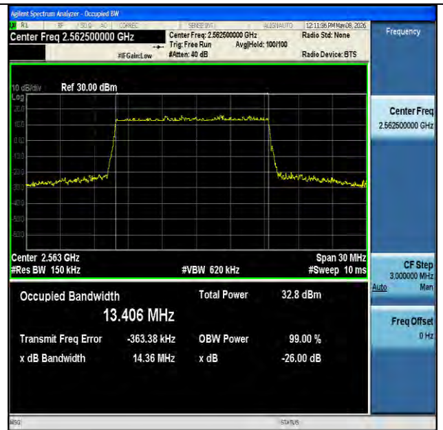
NTNV-n7-PC3-15-15-H-DFT-QPSK-Outer_Full-Ant1-PASS
