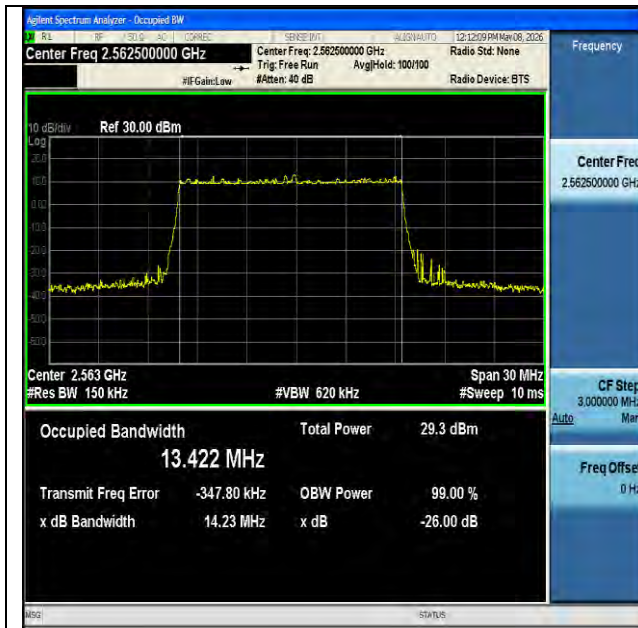
NTNV-n7-PC3-15-15-H-DFT-256QAM-Outer_Full-Ant1-PASS
