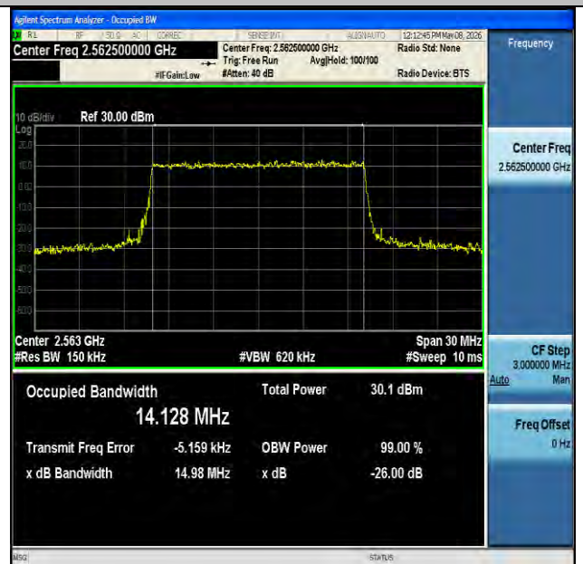
NTNV-n7-PC3-15-15-H-CP-64QAM-Outer_Full-Ant1-PASS
