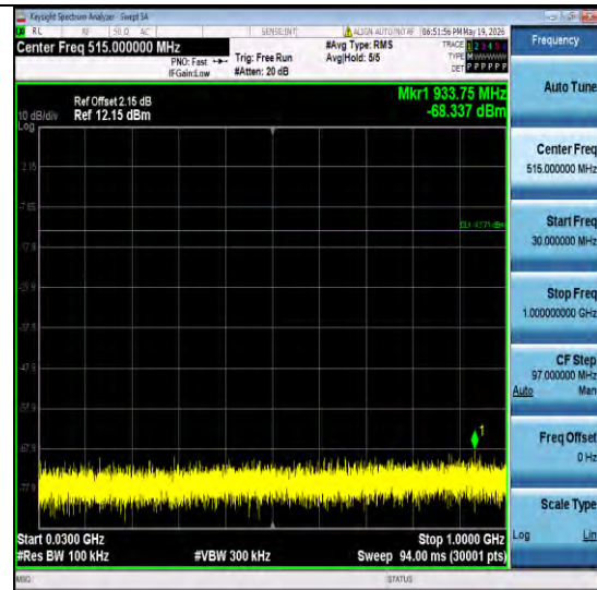
2DH5-Ant6-2441-30~1000-PASS
