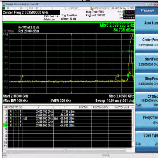
3DH5-Ant6-2402-PASS
