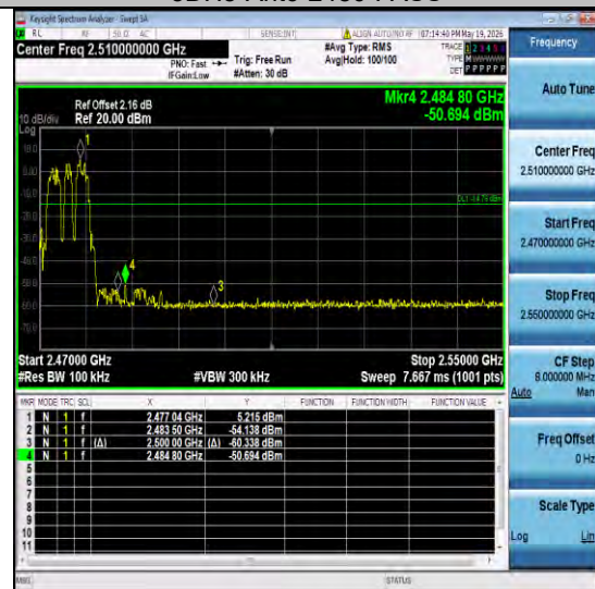
3DH5-Ant6-Hop_2480-PASS
