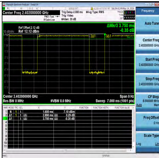
NTNV-3DH5-Ant6-2402
