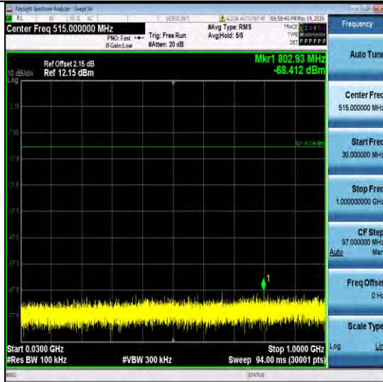
3DH5-Ant6-2441-30~1000-PASS
