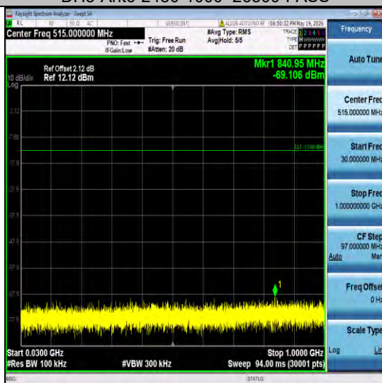
2DH5-Ant6-2402-30~1000-PASS
