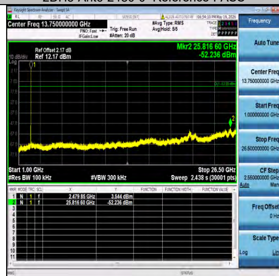
2DH5-Ant6-2480-1000~26500-PASS
