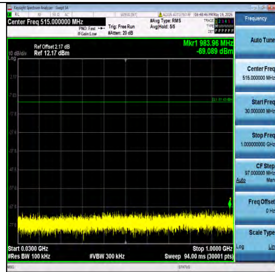
DH5-Ant6-2480-30~1000-PASS
