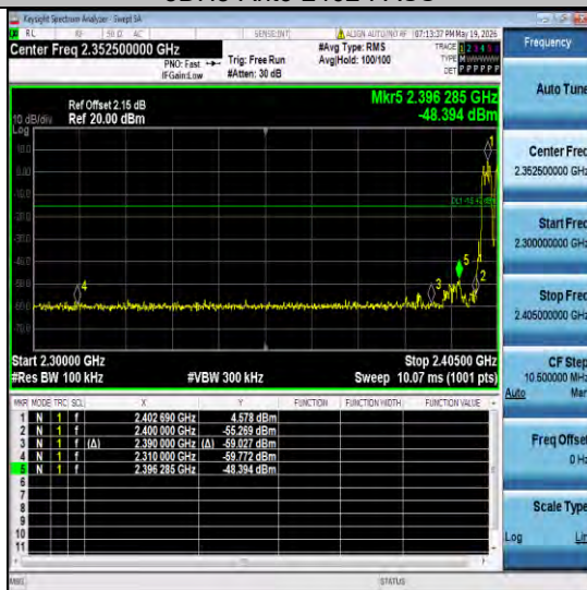
3DH5-Ant6-Hop_2402-PASS
