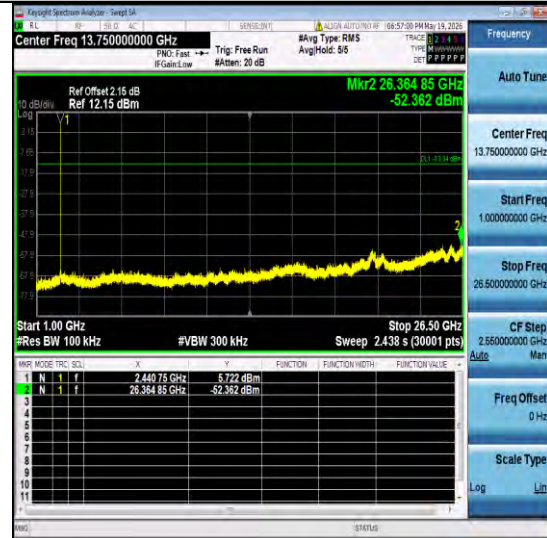
3DH5-Ant6-2441-1000~26500-PASS
