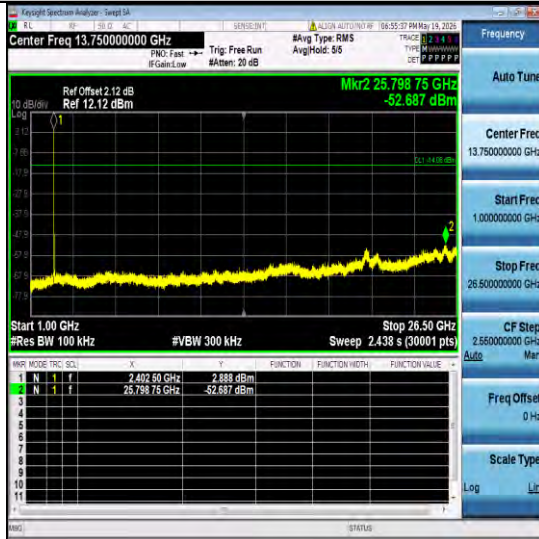
3DH5-Ant6-2402-1000~26500-PASS
