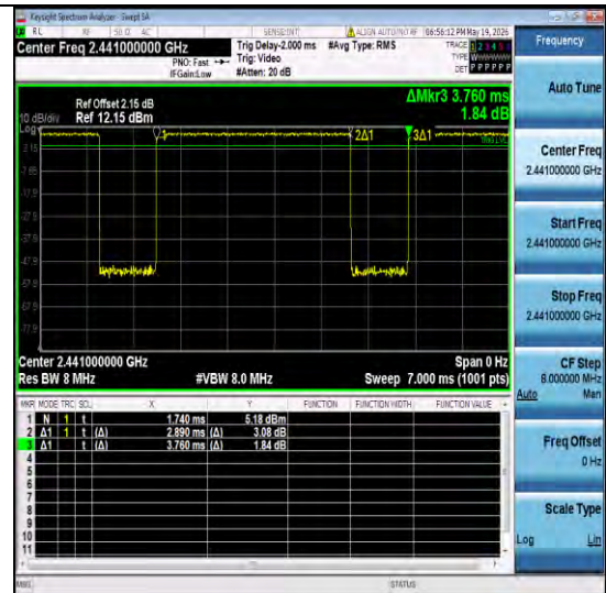
NTNV-3DH5-Ant6-2441
