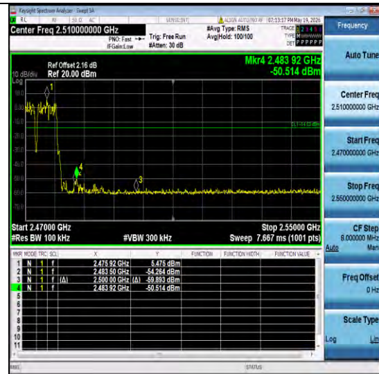
2DH5-Ant6-Hop_2480-PASS
