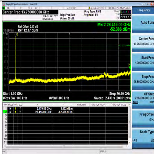
3DH5-Ant6-2480-1000~26500-PASS
