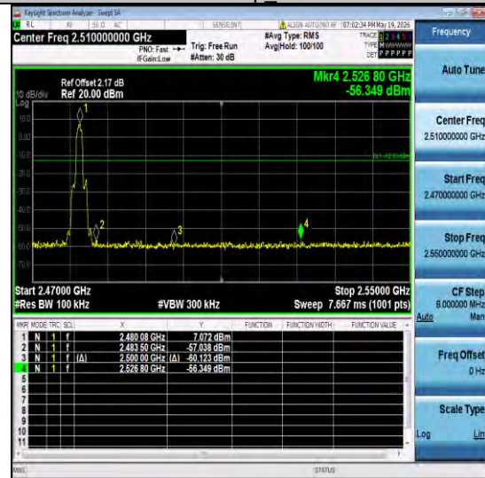
3DH5-Ant6-2480-PASS
