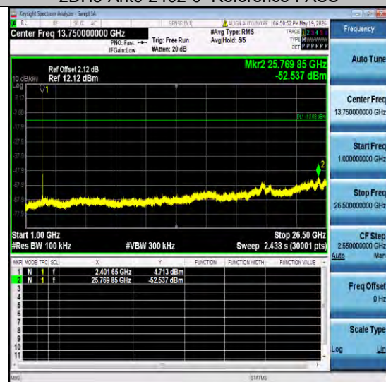
2DH5-Ant6-2402-1000~26500-PASS
