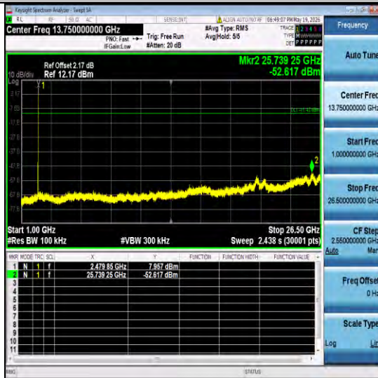
DH5-Ant6-2480-1000~26500-PASS
