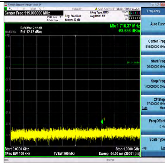
3DH5-Ant6-2402-30~1000-PASS
