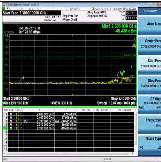
2DH5-Ant6-Hop_2402-PASS
