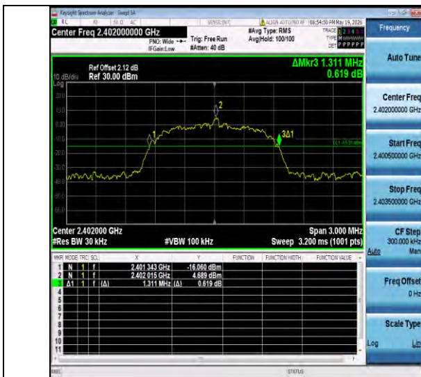
3DH5-Ant6-2402
