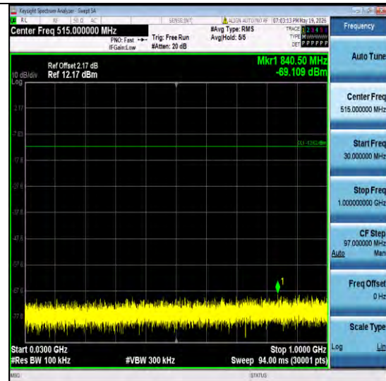
3DH5-Ant6-2480-30~1000-PASS
