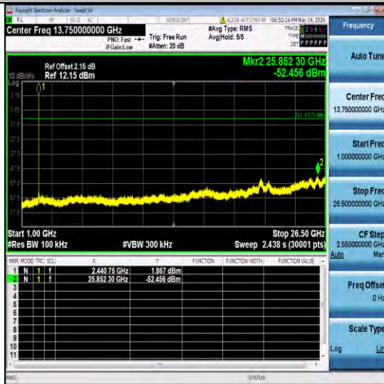
2DH5-Ant6-2441-1000~26500-PASS
