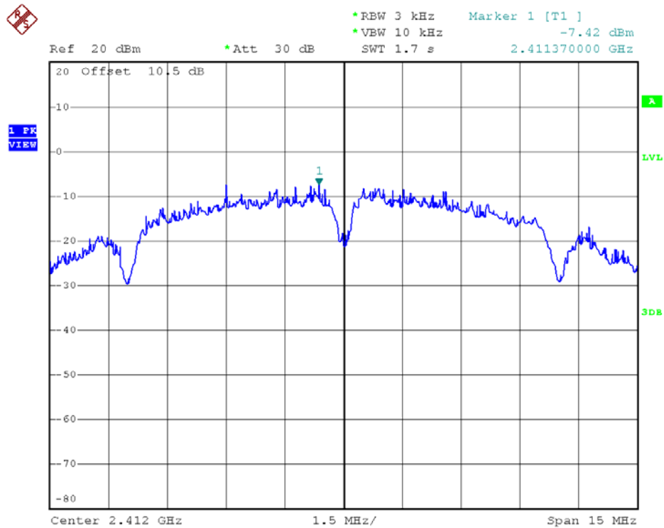
802.11b - Channel 1
