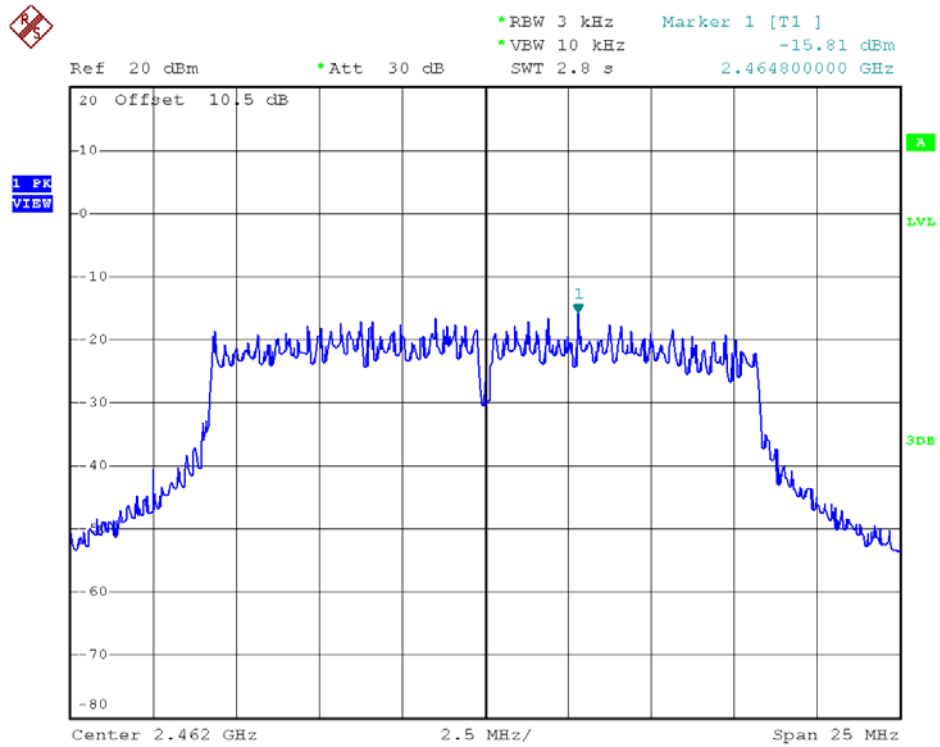
802.11g - Channel 11
