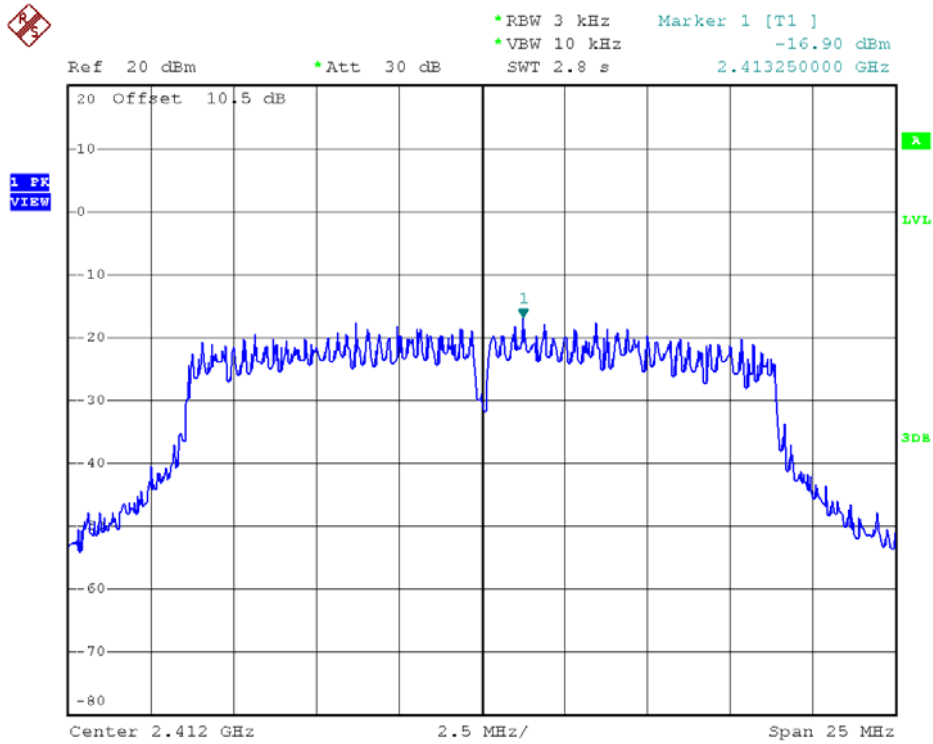
802.11n20 - Channel 1
