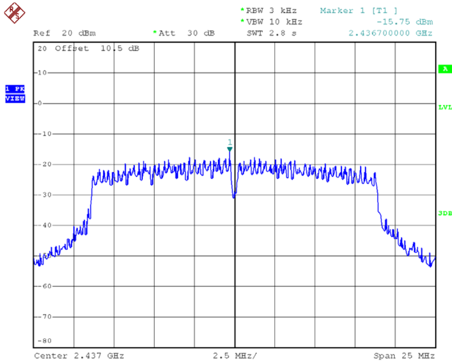
802.11n20 - Channel 6
