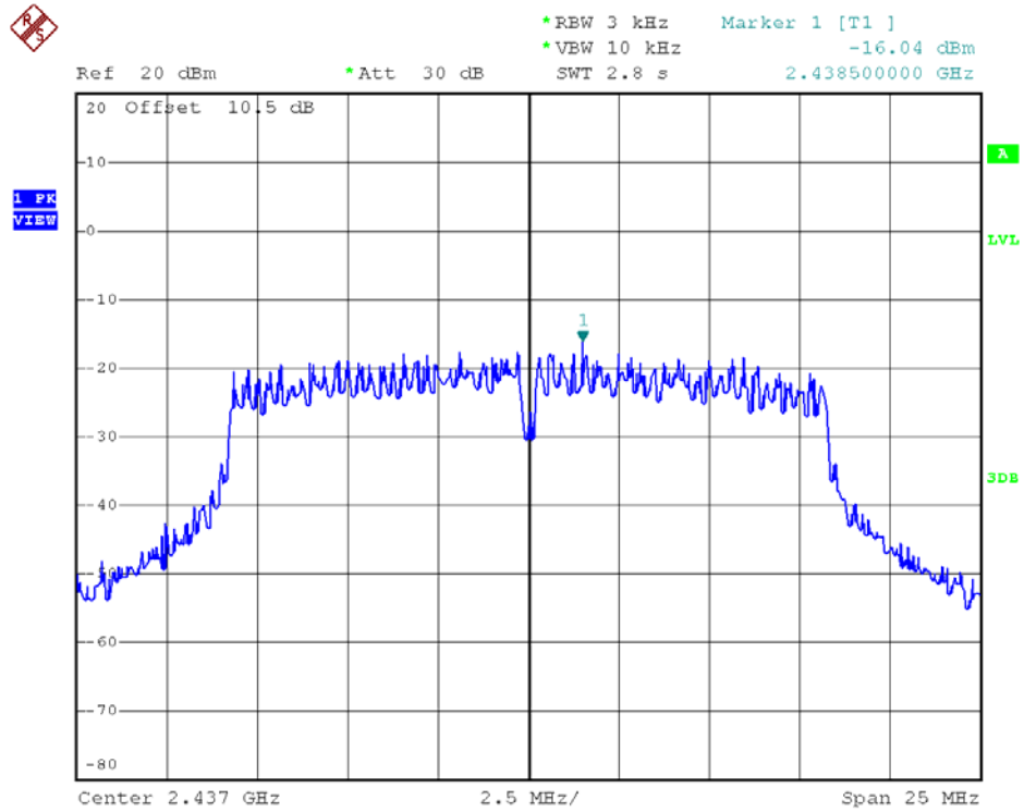
802.11g - Channel 6
