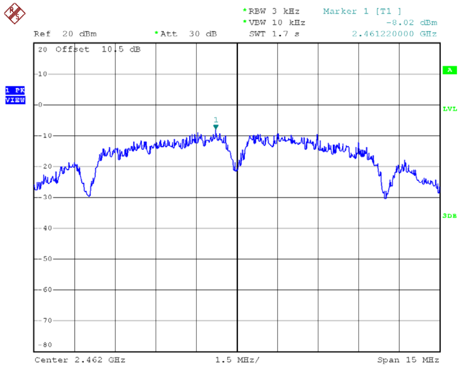
802.11b - Channel 11
