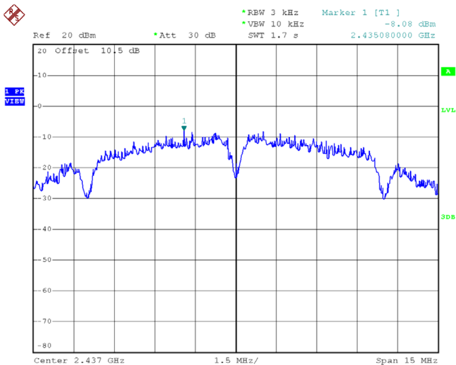
802.11b - Channel 6
