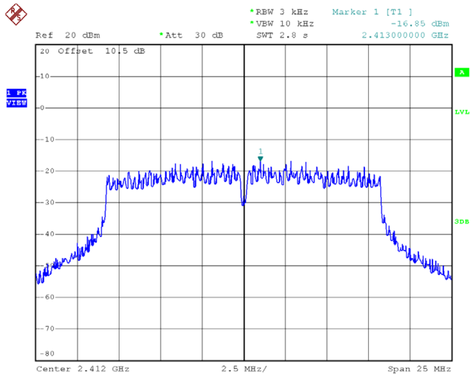
802.11g - Channel 1
