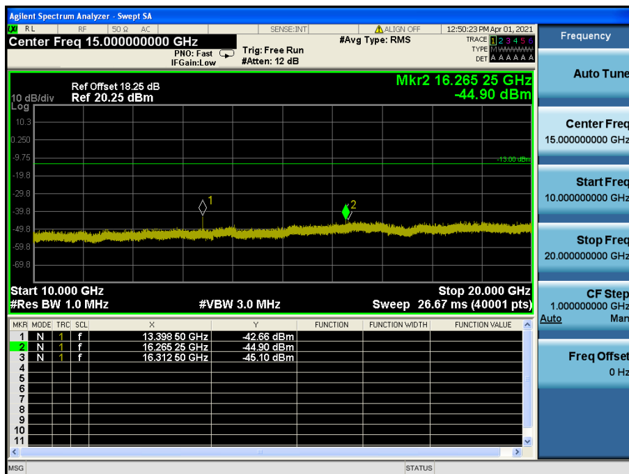
LTE Band 25(2) / 1.4 MHz / 16QAM - RB Size/Offset (3/0) – High Channel
