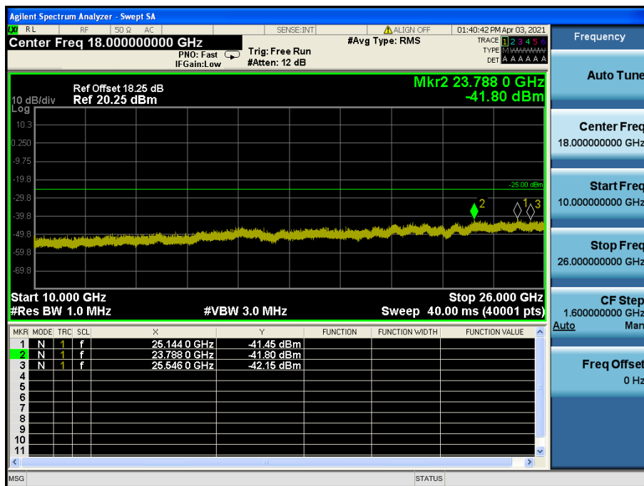
LTE Band 7 / 5 MHz / QPSK - RB Size/Offset (6/0) – Low Channel
