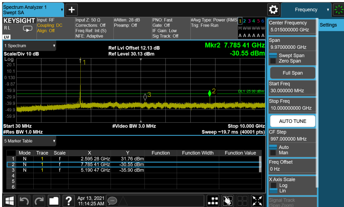
LTE Band 41(38) / 5 MHz / QPSK - RB Size/Offset (1/24) – Mid Channel
