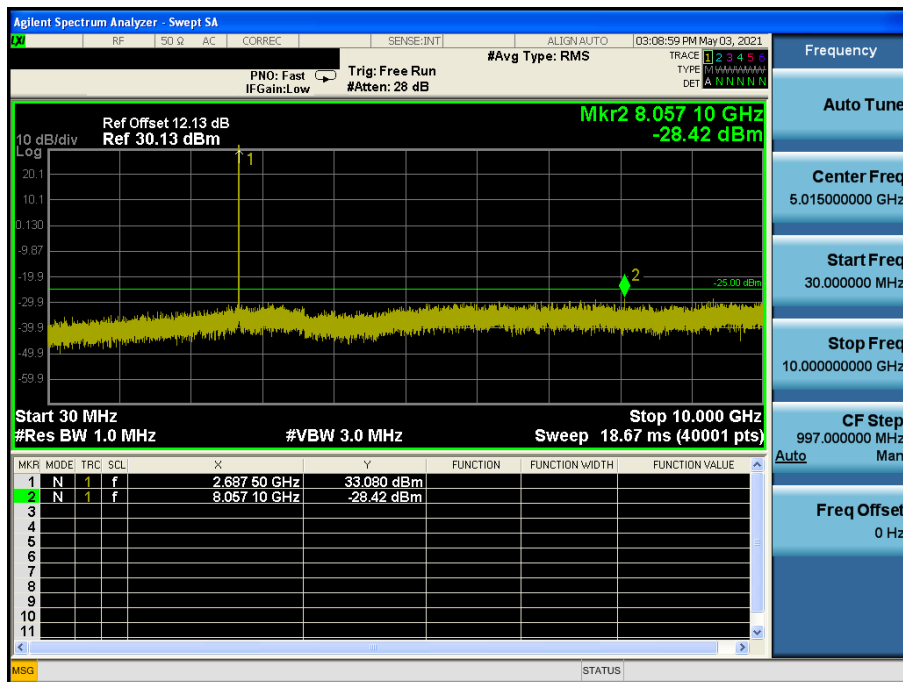
LTE Band 41(38) / 10 MHz / QPSK - RB Size/Offset (50/0) – High Channel
