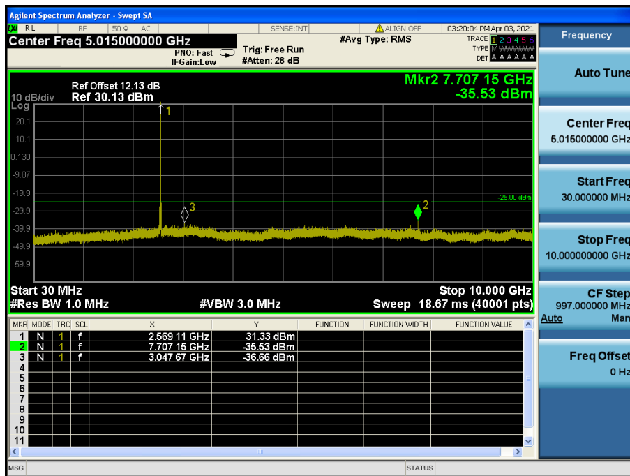
LTE Band 7 / 20 MHz / QPSK - RB Size/Offset (1/99) – High Channel
