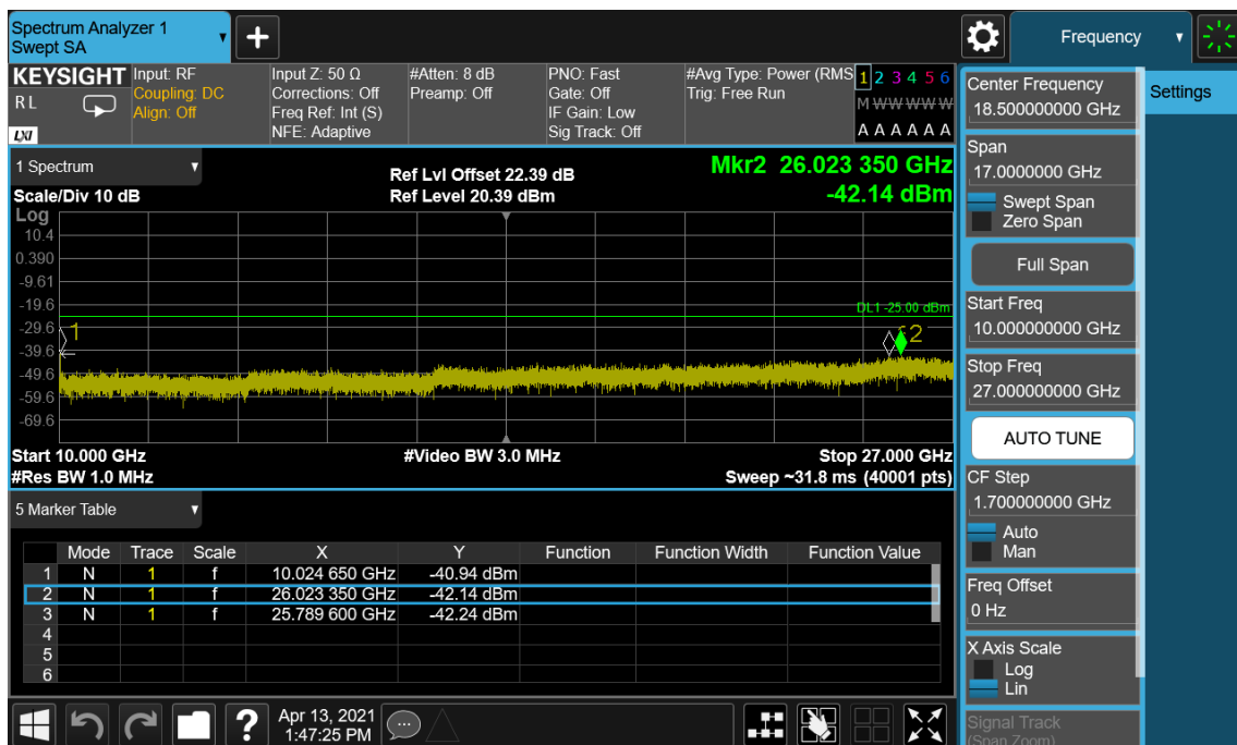
LTE Band 41(38) / 20 MHz / 16QAM - RB Size/Offset (1/50) –Low Channel
