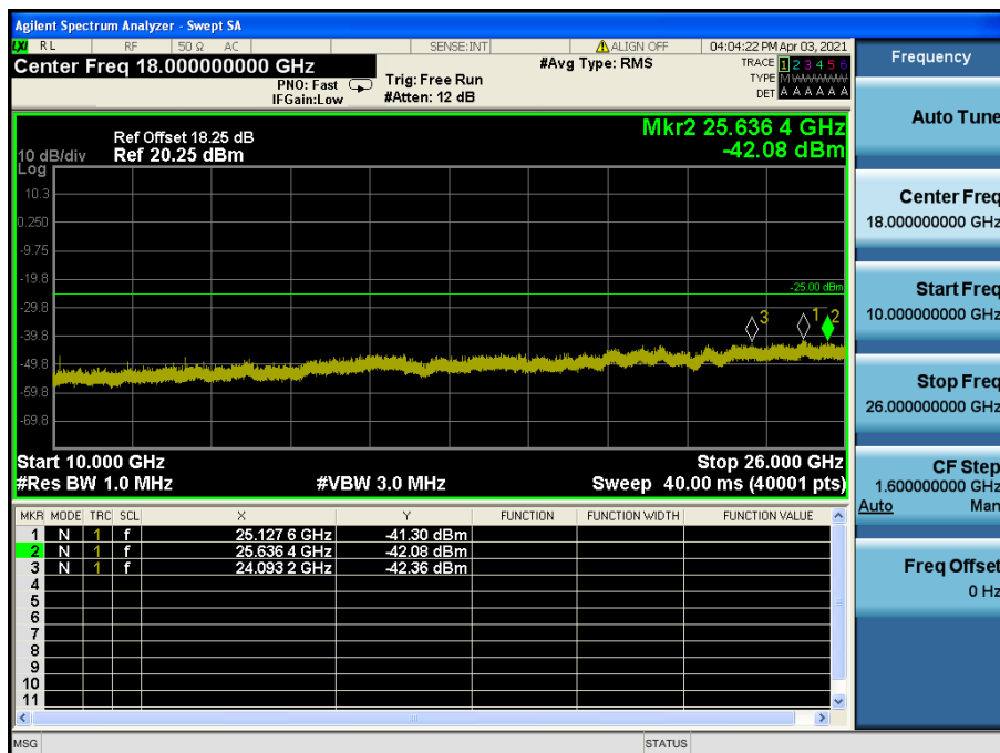
LTE Band 7 / 10 MHz / 16QAM - RB Size/Offset (1/25) – Mid Channel
