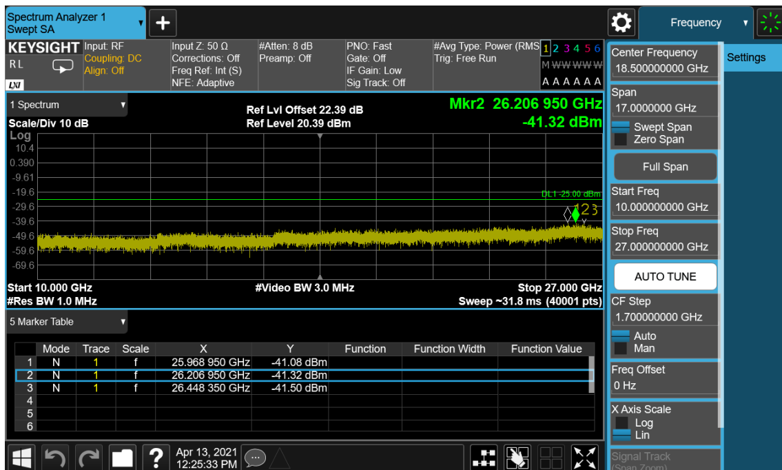
LTE Band 41(38) / 20 MHz / QPSK - RB Size/Offset (100/0) – High Channel
