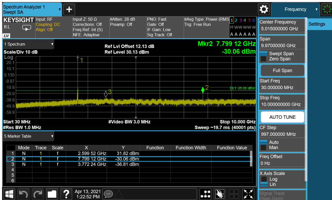
LTE Band 41(38) / 15 MHz / 16QAM - RB Size/Offset (1/74) – Mid Channel
