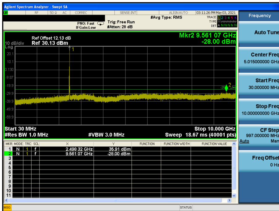
LTE Band 41(38) / 5 MHz / QPSK - RB Size/Offset (1/12) – Low Channel
