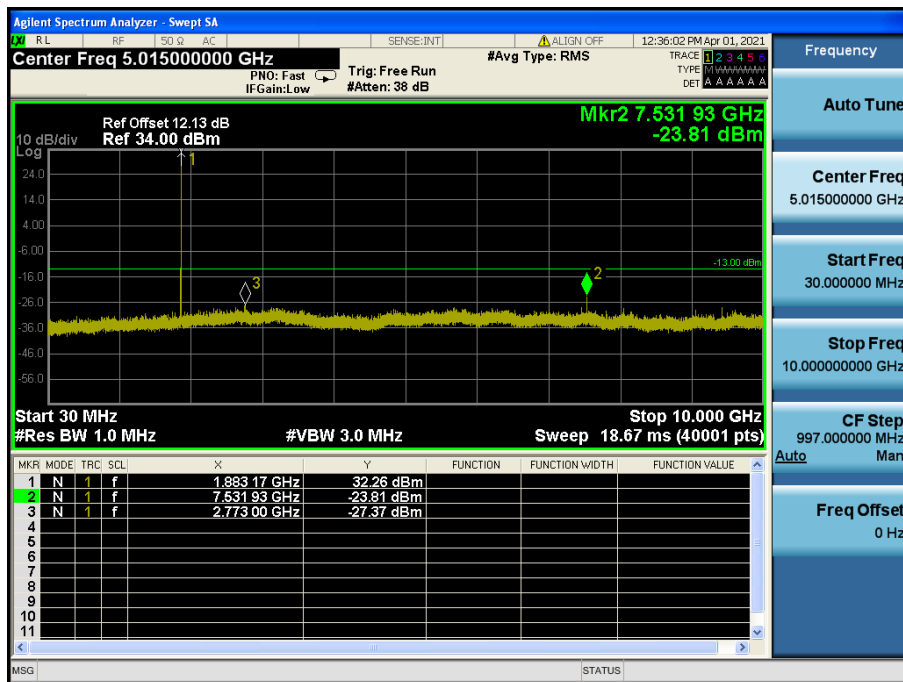
LTE Band 25(2) / 1.4 MHz / 16QAM - RB Size/Offset (1/5) – Mid Channel
