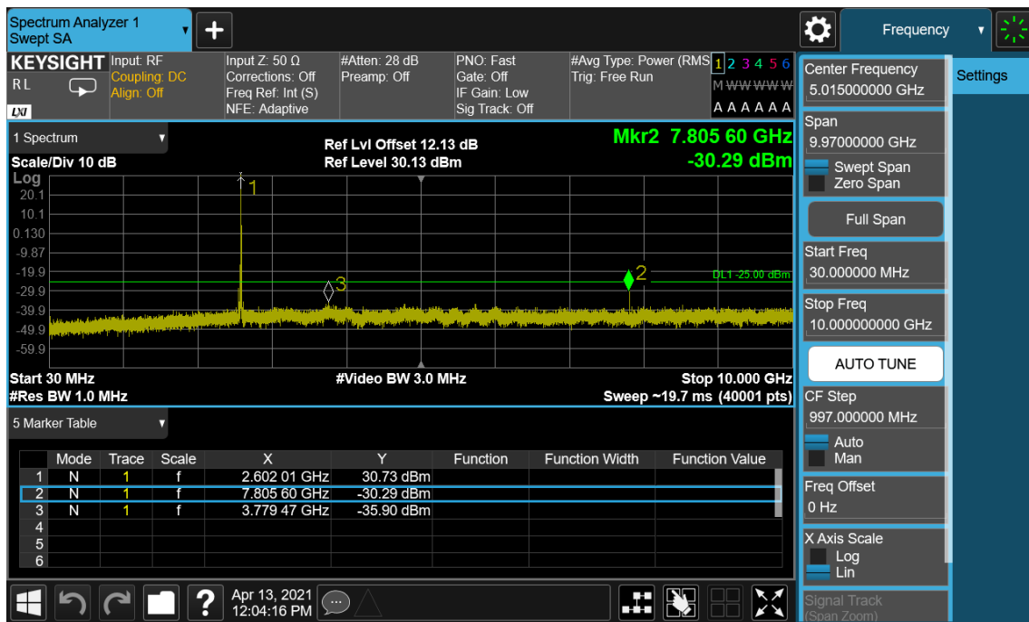
LTE Band 41(38) / 20 MHz / QPSK - RB Size/Offset (1/99)–Mid Channel
