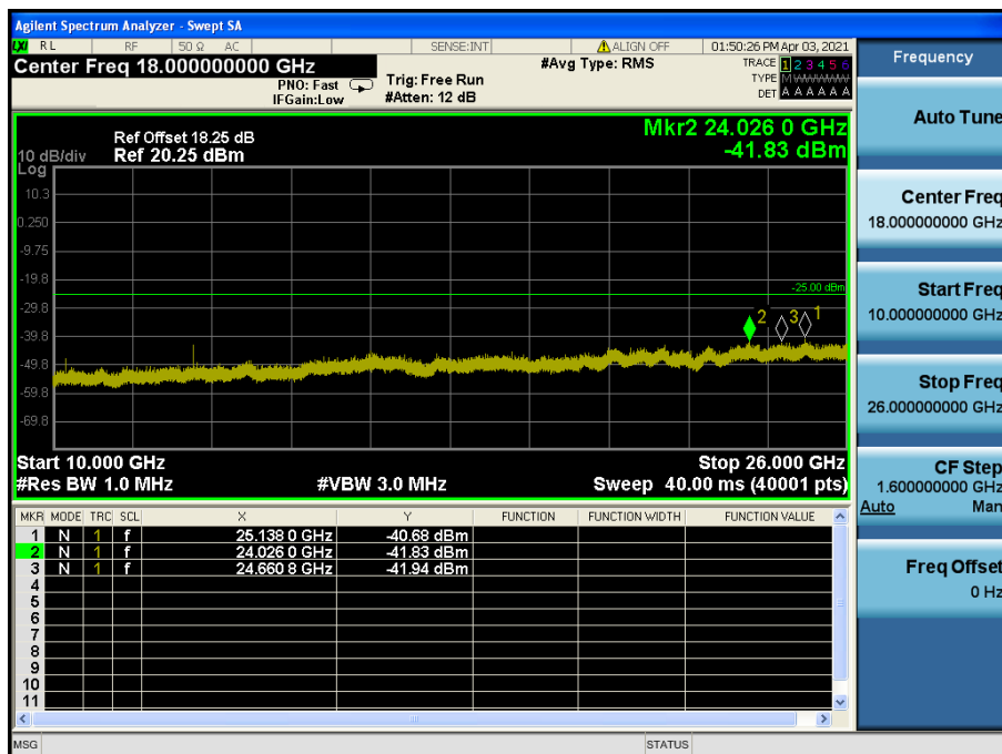
LTE Band 7 / 5 MHz / QPSK - RB Size/Offset (1/0) – High Channel
