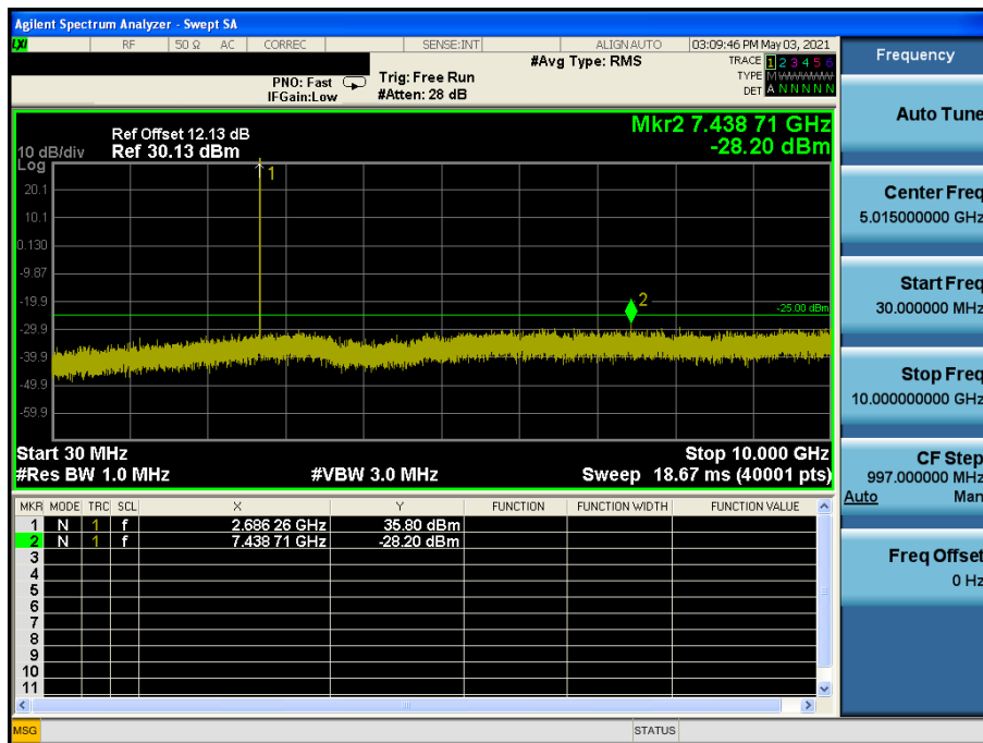
LTE Band 41(38) / 5 MHz / 16QAM - RB Size/Offset (12/0) – High Channel
