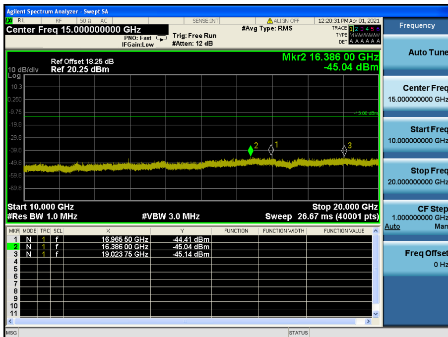
LTE Band 25(2) / 1.4 MHz / 16QAM - RB Size/Offset (1/2) – Low Channel
