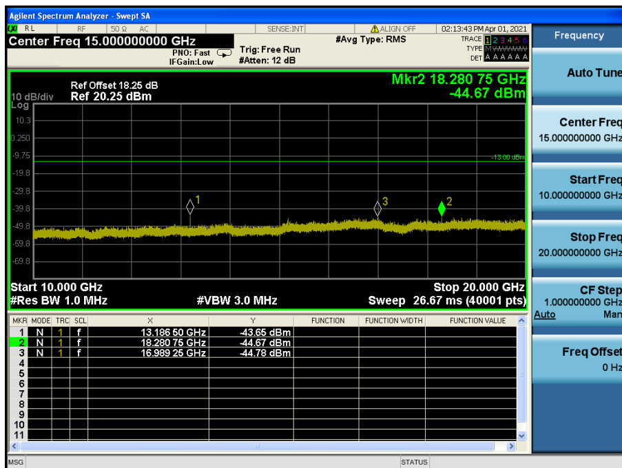
LTE Band 25(2) / 3 MHz / 16QAM - RB Size/Offset (1/14) – Mid Channel
