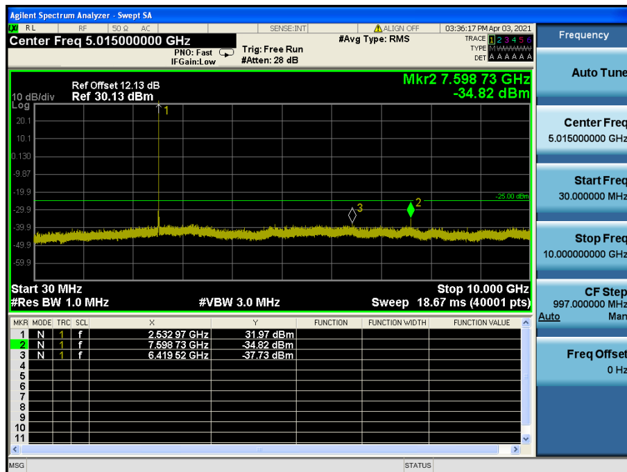
LTE Band 7 / 5 MHz / 16QAM - RB Size/Offset (1/0) – Mid Channel
