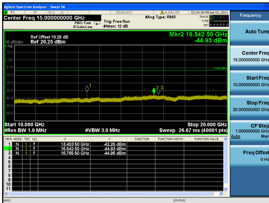
LTE Band 25(2) / 3 MHz / 16QAM - RB Size/Offset (1/14) – High Channel
