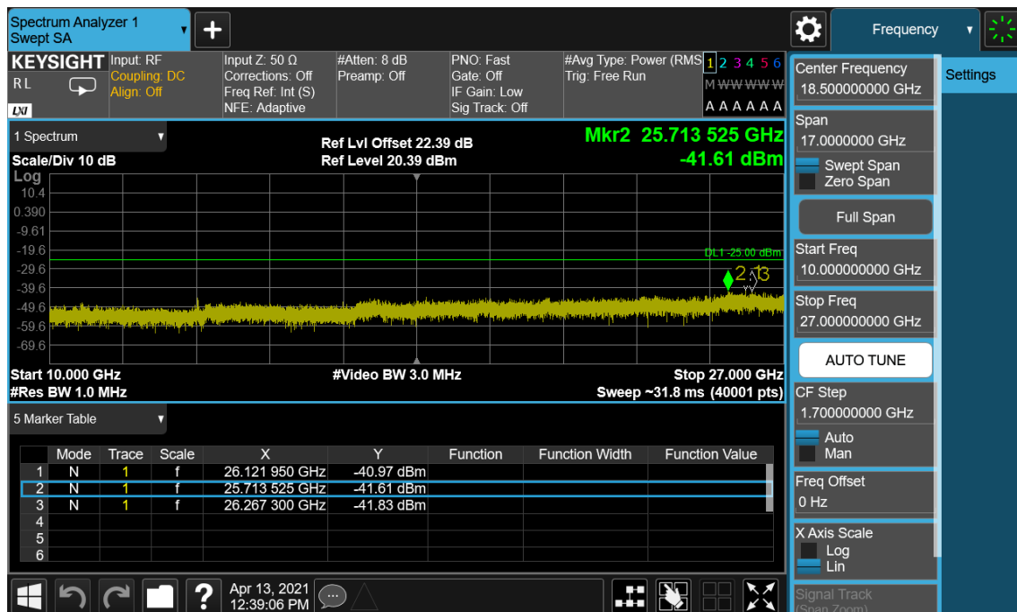
LTE Band 41(38) / 5 MHz / 16QAM - RB Size/Offset (12/0) – High Channel
