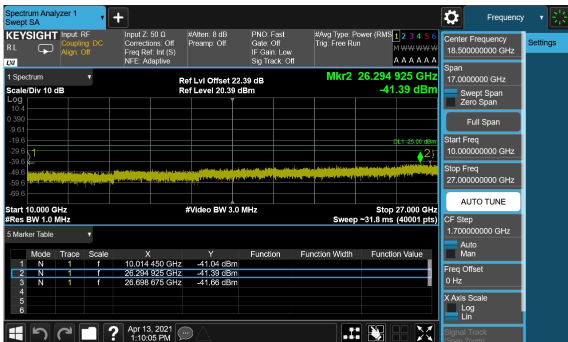
LTE Band 41(38) / 15 MHz / 16QAM - RB Size/Offset (1/36)–Low Channel
