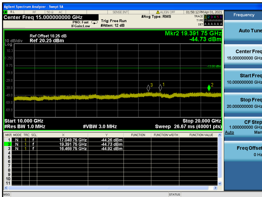
LTE Band 25(2) / 3 MHz / 16QAM - RB Size/Offset (1/7) – Low Channel
