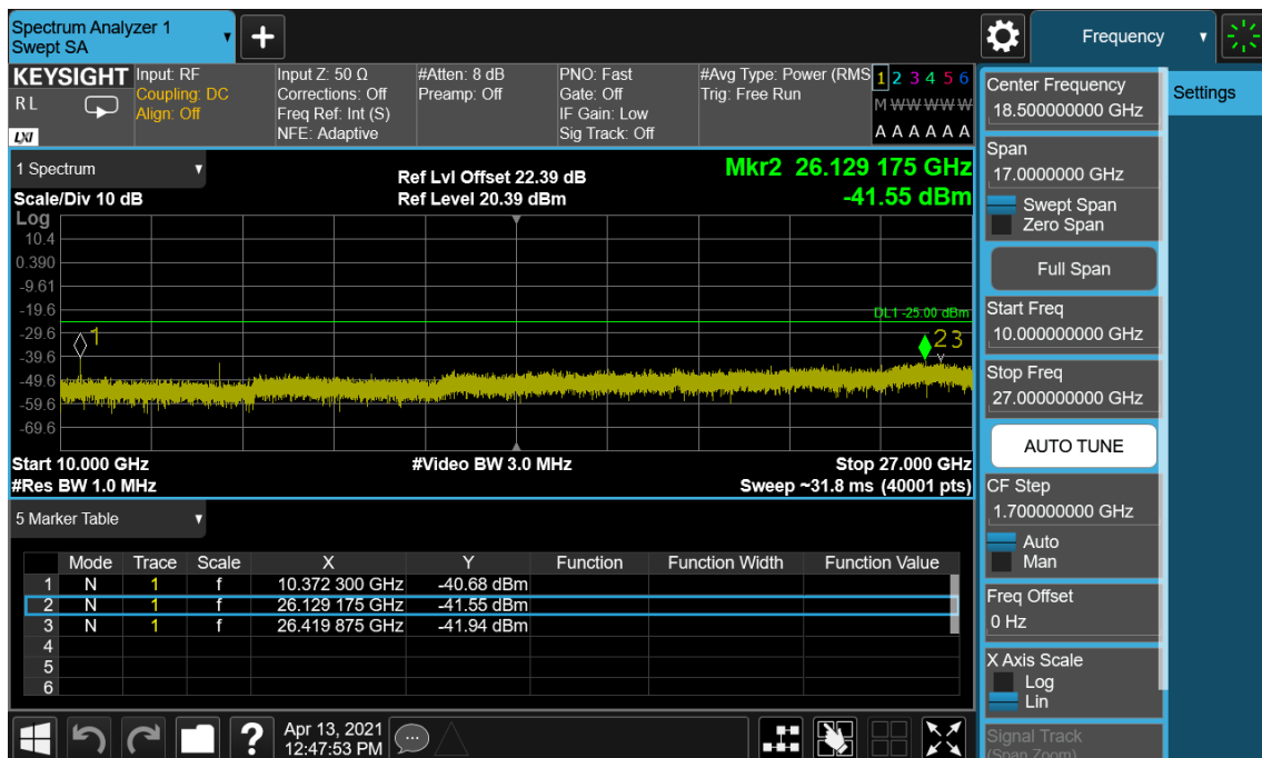
LTE Band 41(38) / 10 MHz / 16QAM - RB Size/Offset (1/25) – Mid Channel
