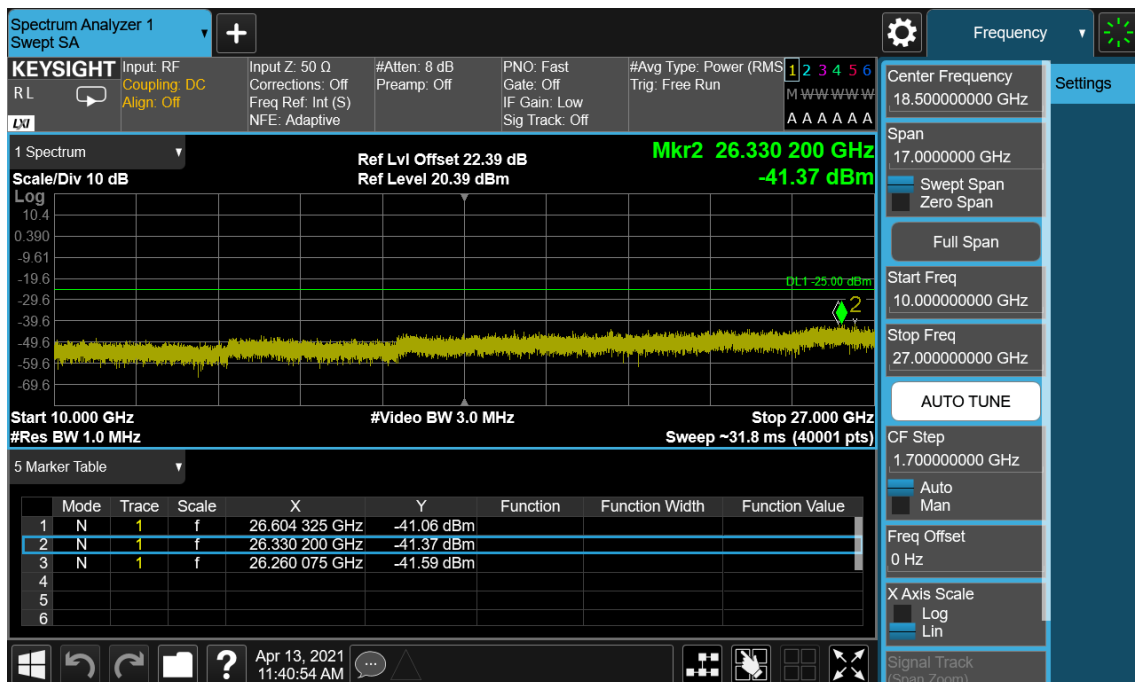
LTE Band 41(38) / 10 MHz / QPSK - RB Size/Offset (50/0) – High Channel
