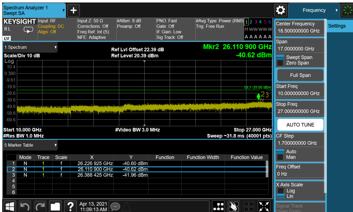
LTE Band 41(38) / 5 MHz / QPSK - RB Size/Offset (1/12) – Low Channel
