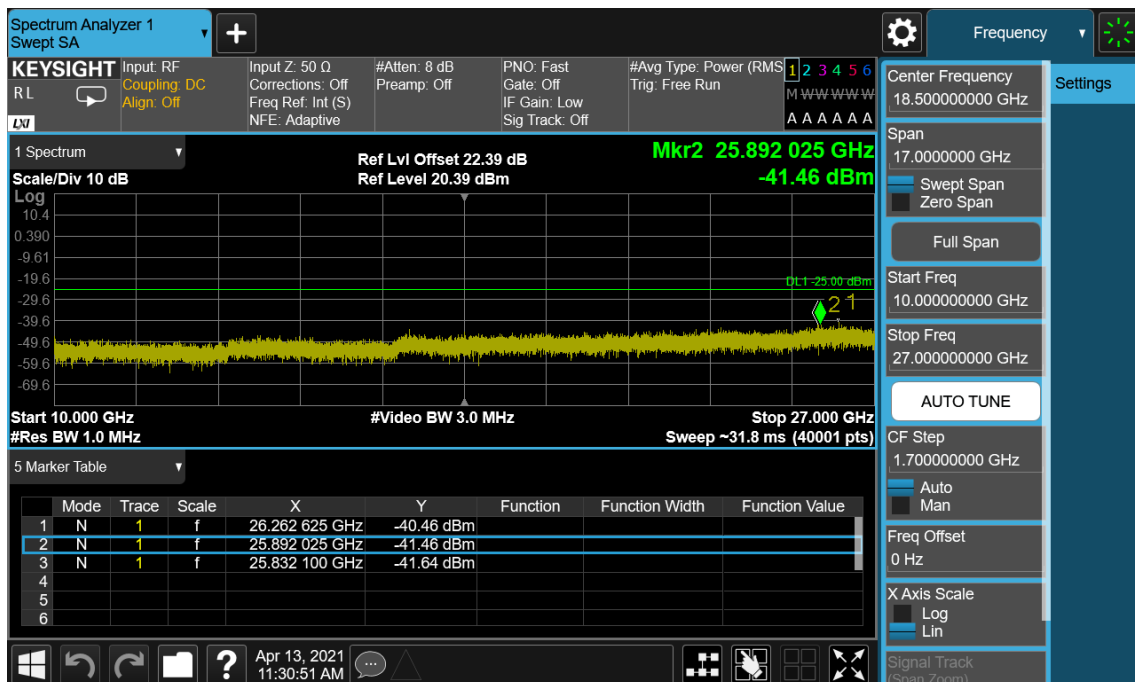
LTE Band 41(38) / 10 MHz / QPSK - RB Size/Offset (50/0) – Low Channel
