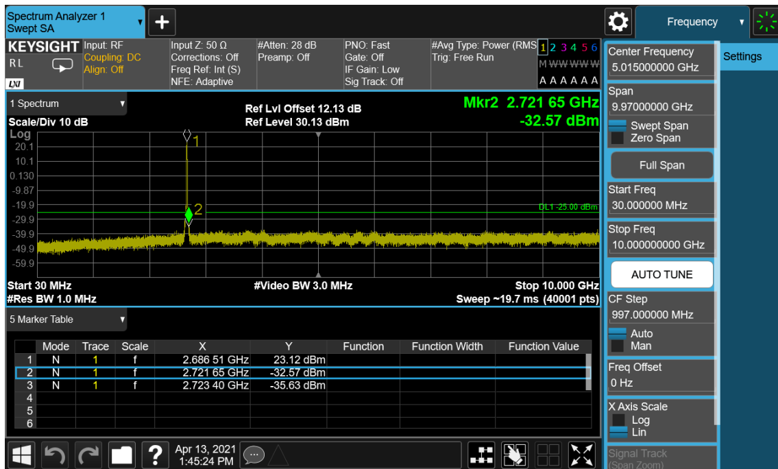
LTE Band 41(38) / 15 MHz / 16QAM - RB Size/Offset (75/0) – High Channel
