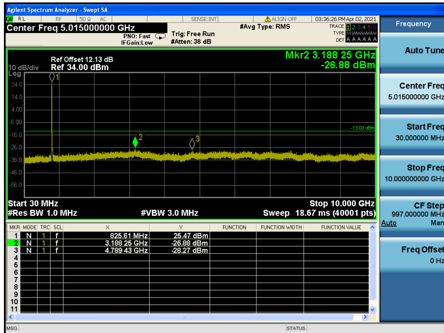
LTE Band 26 / 15MHz / QPSK - RB Size/Offset (75/0) - Low Channel
