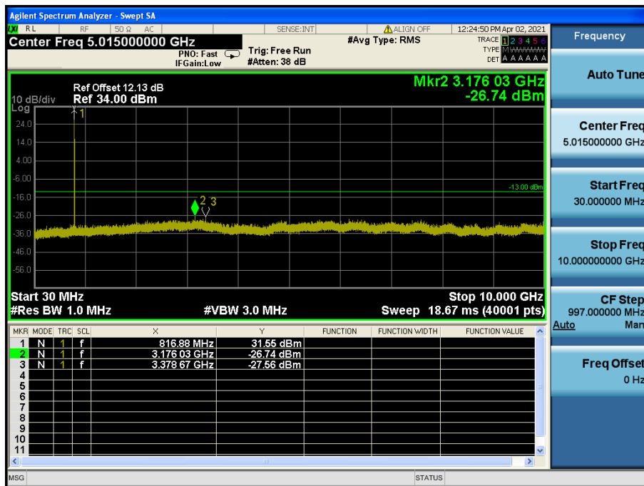
LTE Band 26 / 5MHz / QPSK - RB Size/Offset (1/12) - Low Channel
