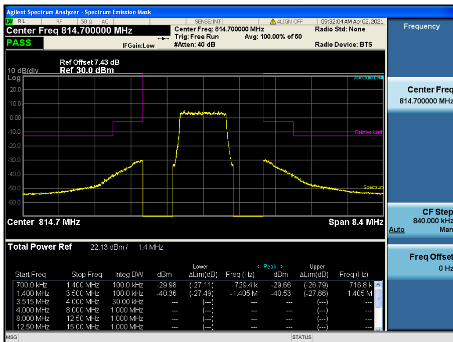
LTE Band 26 / 1.4MHz / 16QAM - RB Size/Offset (6/0) - Low Channel
