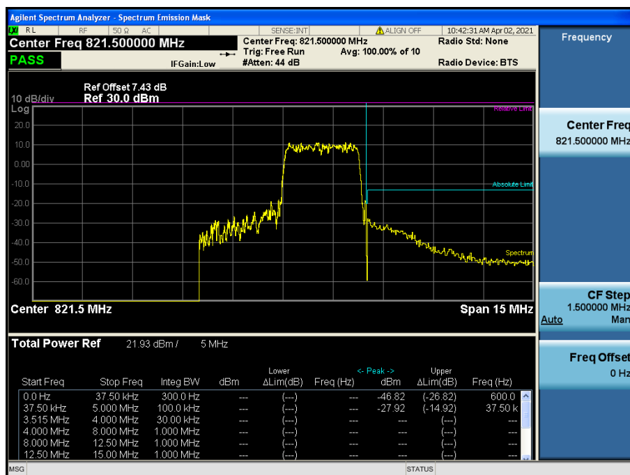
LTE Band 26 / 5MHz / 16QAM - RB Size/Offset (12/13)
