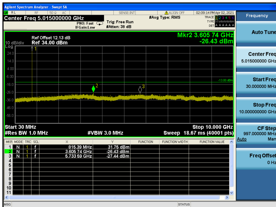
LTE Band 26 / 1.4MHz / 16QAM - RB Size/Offset (1/5) – Low Channel
