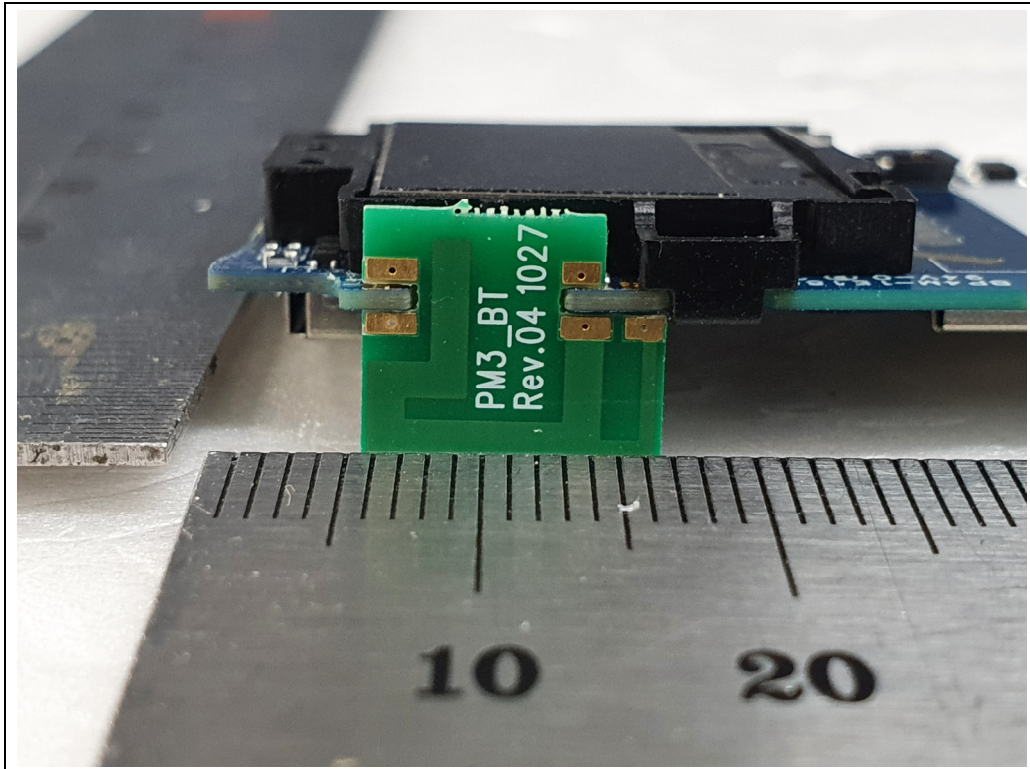
<BT Antenna>
