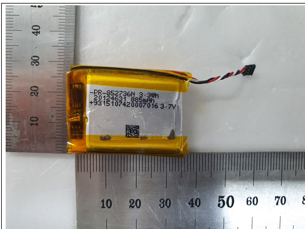
<Battery>
