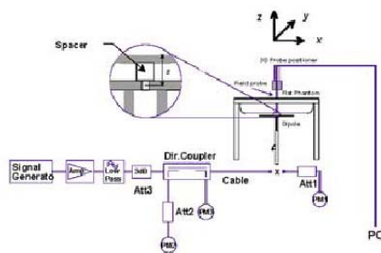
Figure 11.1 Dipole Verification Test Setup Diagram &amp; Photo
