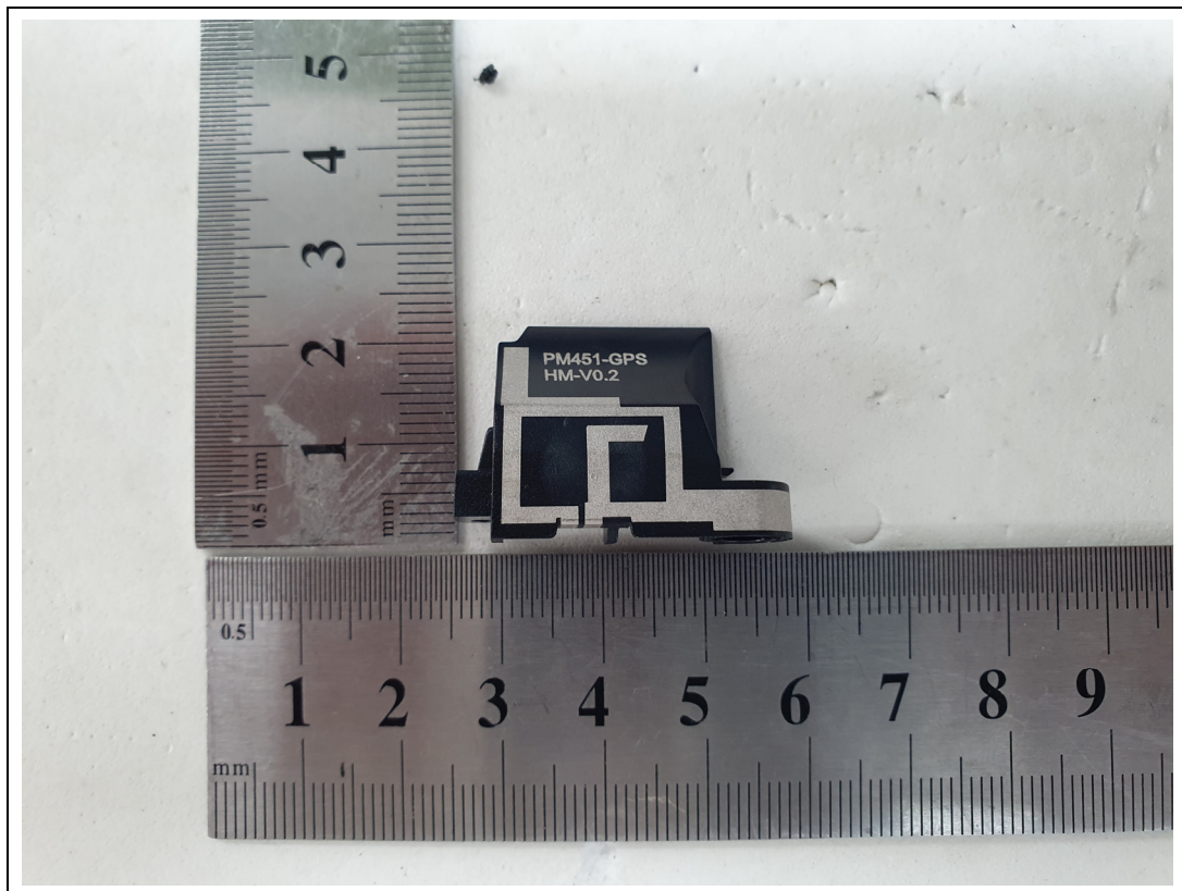
<GPS & WIFI & BT Antenna>
