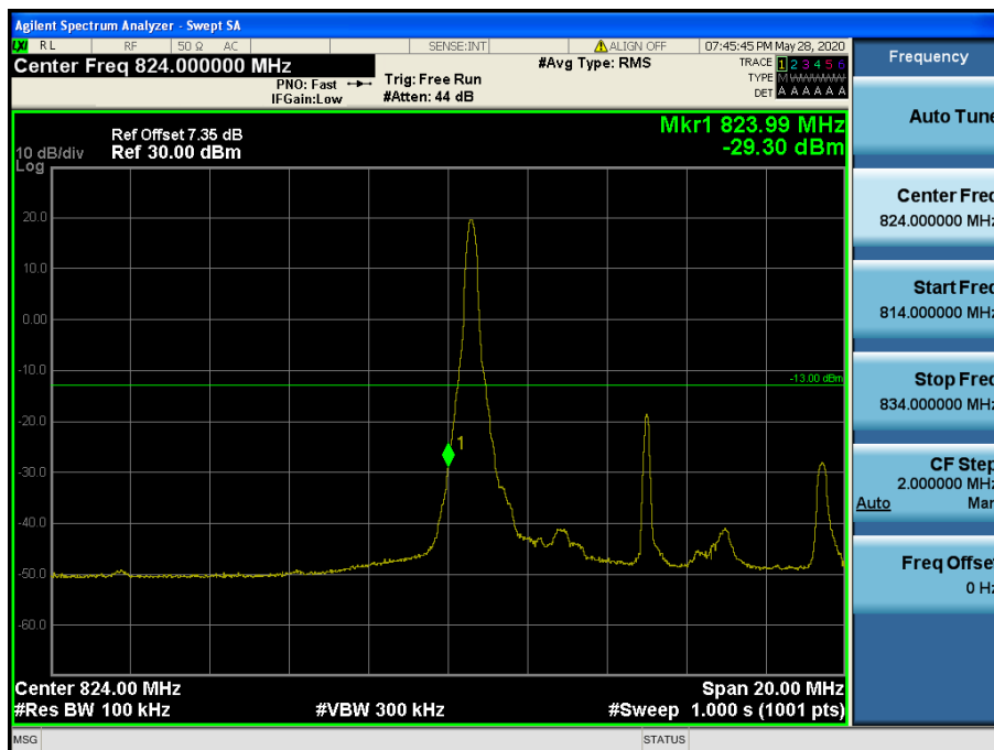
LTE Band 26 / 10 MHz / 16QAM - RB Size/Offset (1/0)
