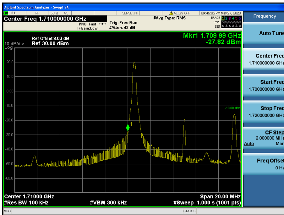
LTE Band 4 / 10 MHz / QPSK - RB Size/Offset (1/0)
