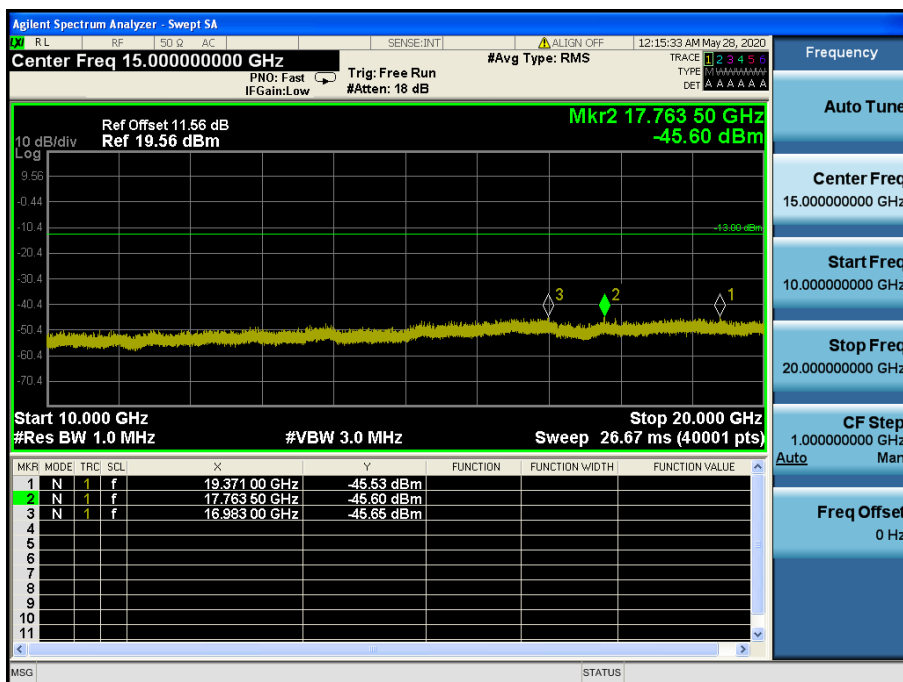
LTE Band 4 / 1.4 MHz / 16QAM - RB Size/Offset (1/0) – Mid Channel
