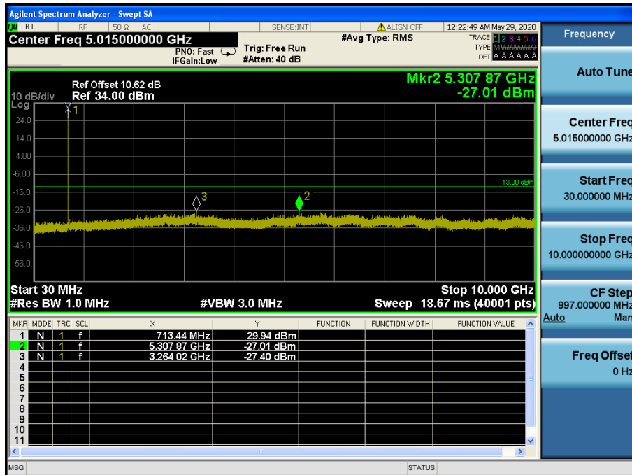
LTE Band 12 / 3 MHz / 16QAM - RB Size/Offset (1/0) – High Channel
