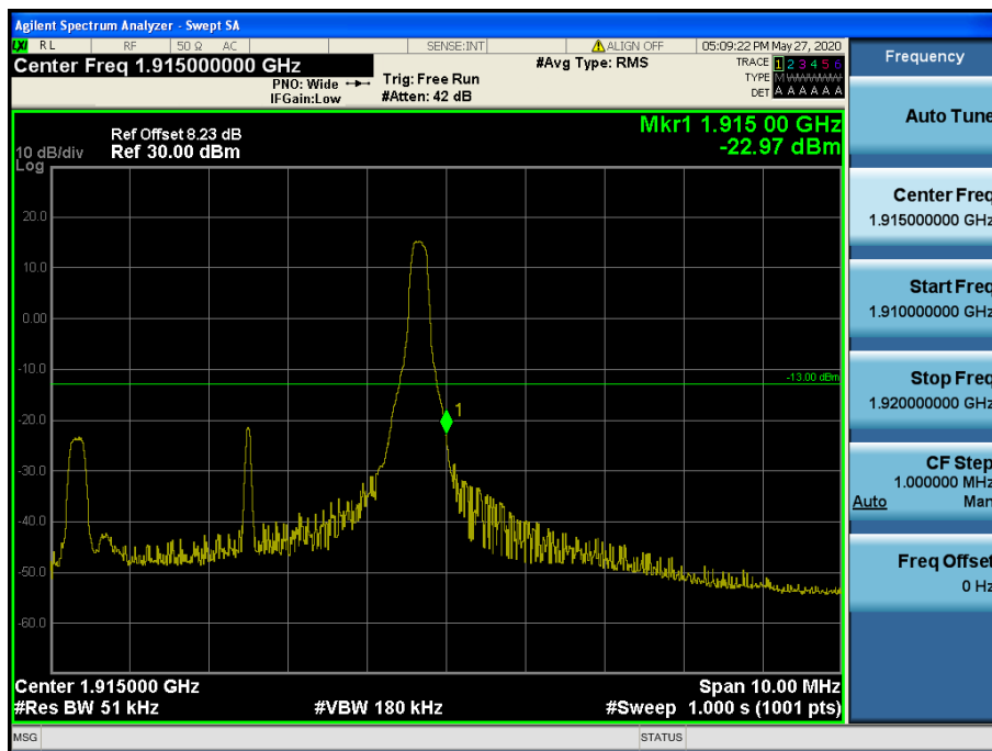
LTE Band 25 / 5 MHz / 16QAM - RB Size/Offset (1/24)
