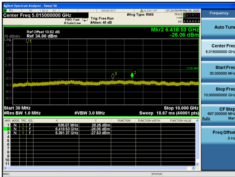
LTE Band 5, 26 / 5 MHz / 16QAM - RB Size/Offset (12/0) – Mid Channel
