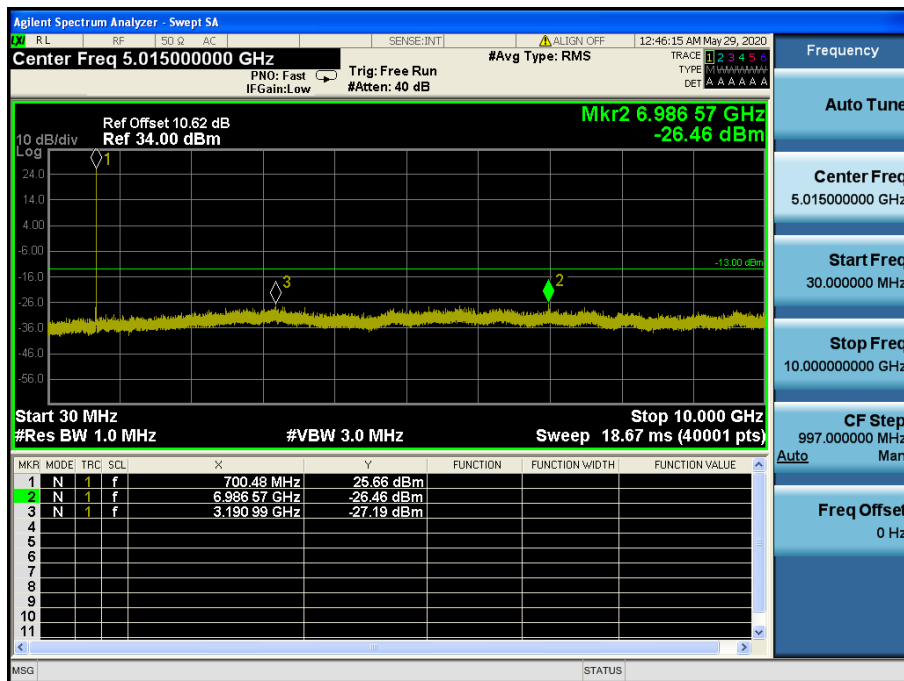
LTE Band 12 / 5 MHz / QPSK - RB Size/Offset (12/0) – Low Channel
