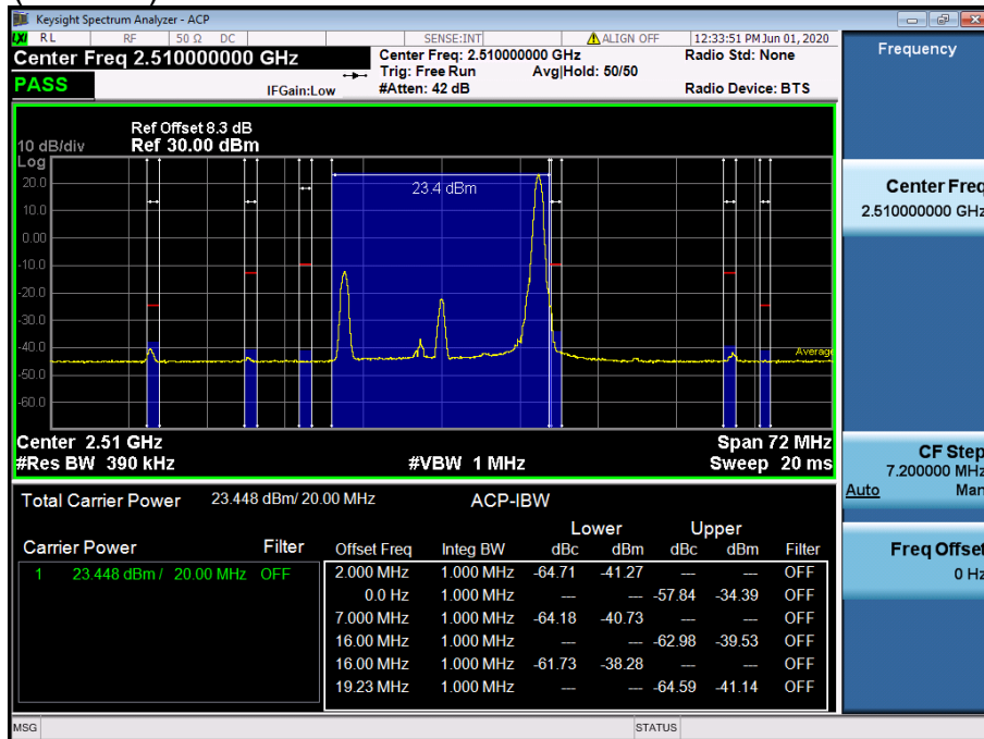
LTE Band 7 / 20 MHz / QPSK - RB Size/Offset (1/99)
