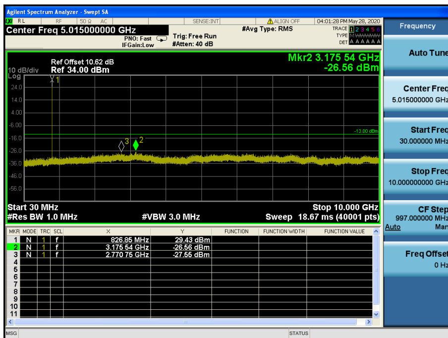
LTE Band 5, 26 / 5 MHz / QPSK - RB Size/Offset (1/12) – Low Channel
