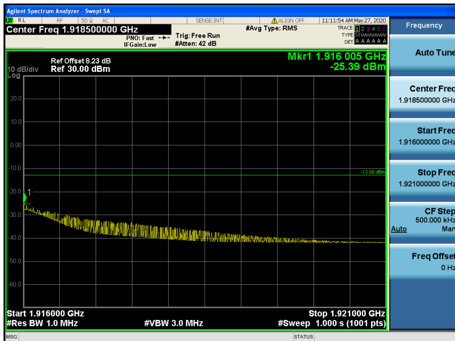
LTE Band 25 / 1.4 MHz / QPSK - RB Size/Offset (1/0)
