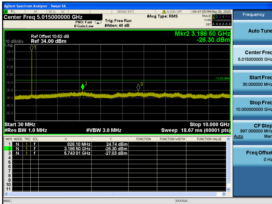
LTE Band 5, 26 / 10 MHz / QPSK - RB Size/Offset (25/12) – Low Channel
