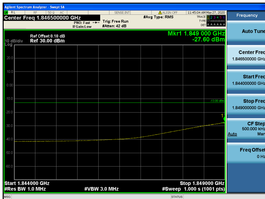
LTE Band 25 / 3 MHz / QPSK - RB Size/Offset (8/7)
