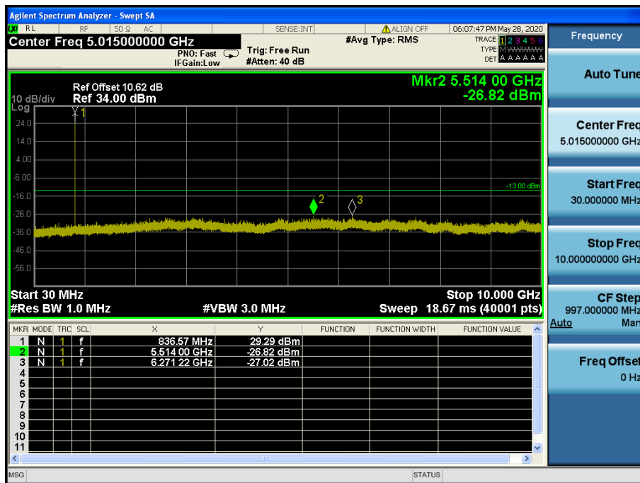
LTE Band 5, 26 / 1.4 MHz / 16QAM - RB Size/Offset (3/0) – Mid Channel
