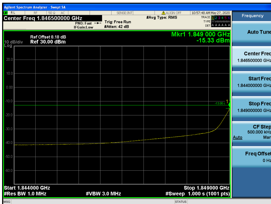
LTE Band 25 / 1.4 MHz / QPSK - RB Size/Offset (3/2)
