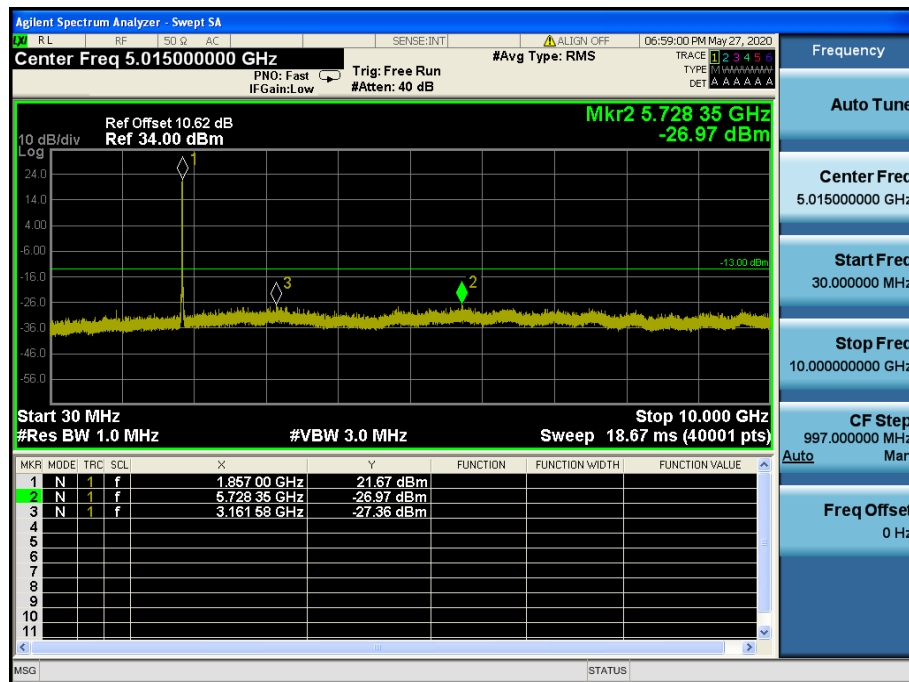
LTE Band 2, 25 / 20 MHz / 16QAM - RB Size/Offset (50/0) –Low Channel
