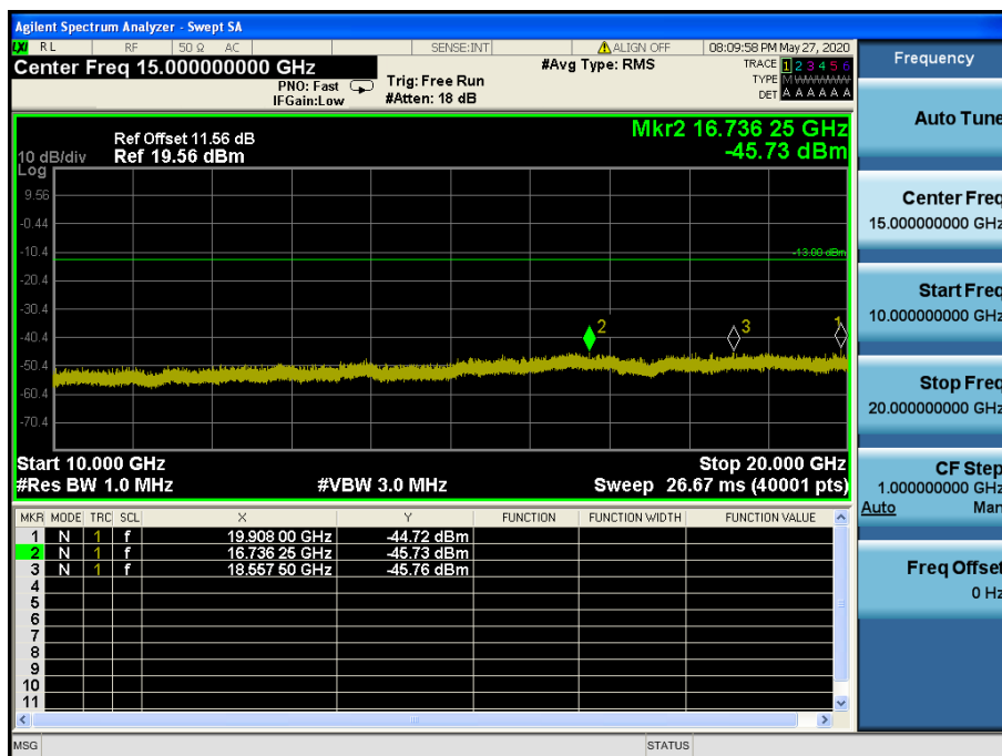
LTE Band 4 / 1.4 MHz / QPSK - RB Size/Offset (3/2) – High Channel
