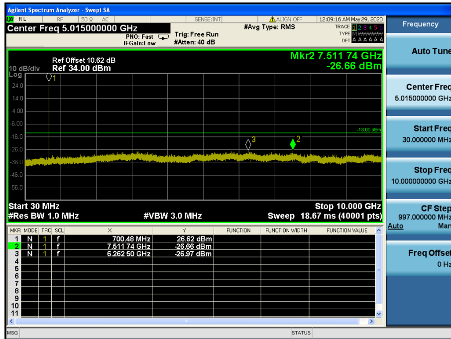
LTE Band 12 / 3 MHz / 16QAM - RB Size/Offset (8/0) – Low Channel
