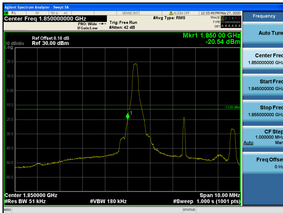
LTE Band 25 / 5 MHz / QPSK Offset/Size (1/0)
