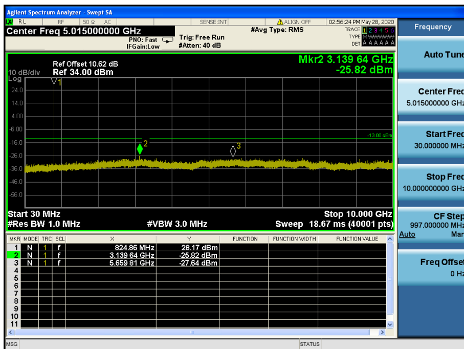
LTE Band 5, 26 / 1.4 MHz / QPSK - RB Size/Offset (6/0) – Low Channel
