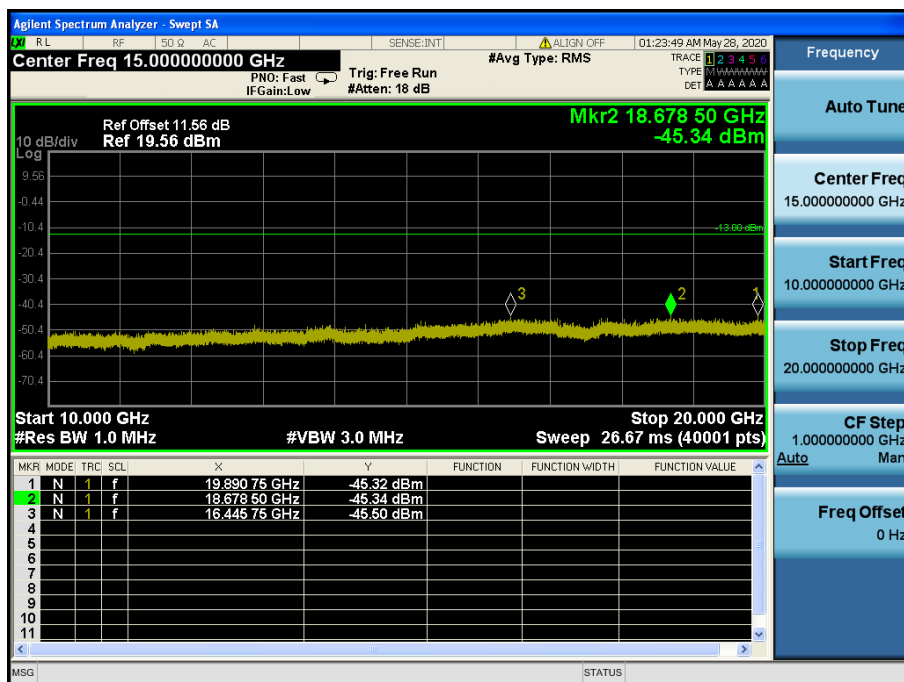
LTE Band 4 / 3 MHz / 16QAM - RB Size/Offset (15/0) – High Channel
