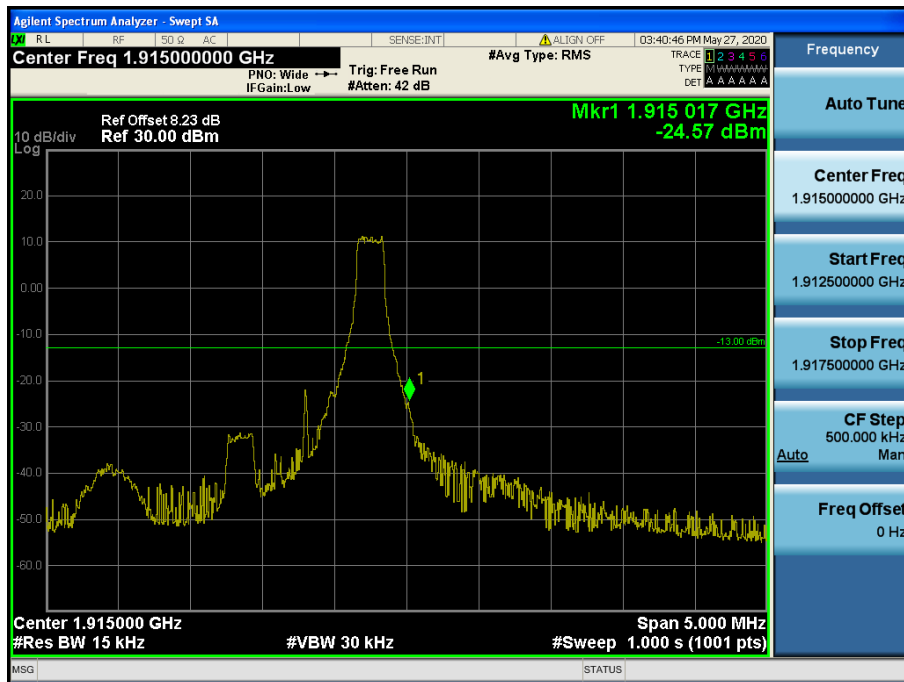
LTE Band 25 / 1.4 MHz / 16QAM - RB Size/Offset (1/5)
