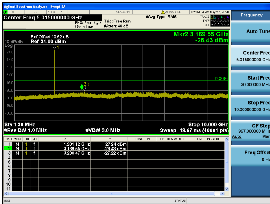
LTE Band 2, 25 / 15 MHz / QPSK - RB Size/Offset (1/0) – High Channel
