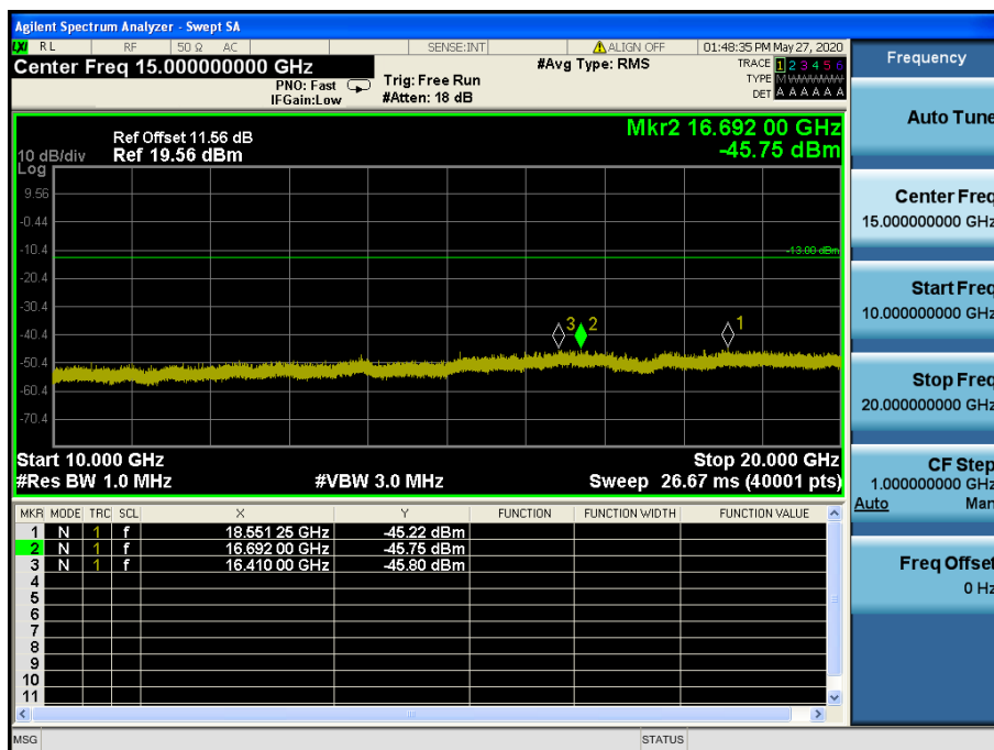
LTE Band 2, 25 / 15 MHz / QPSK - RB Size/Offset (1/36)–Low Channel
