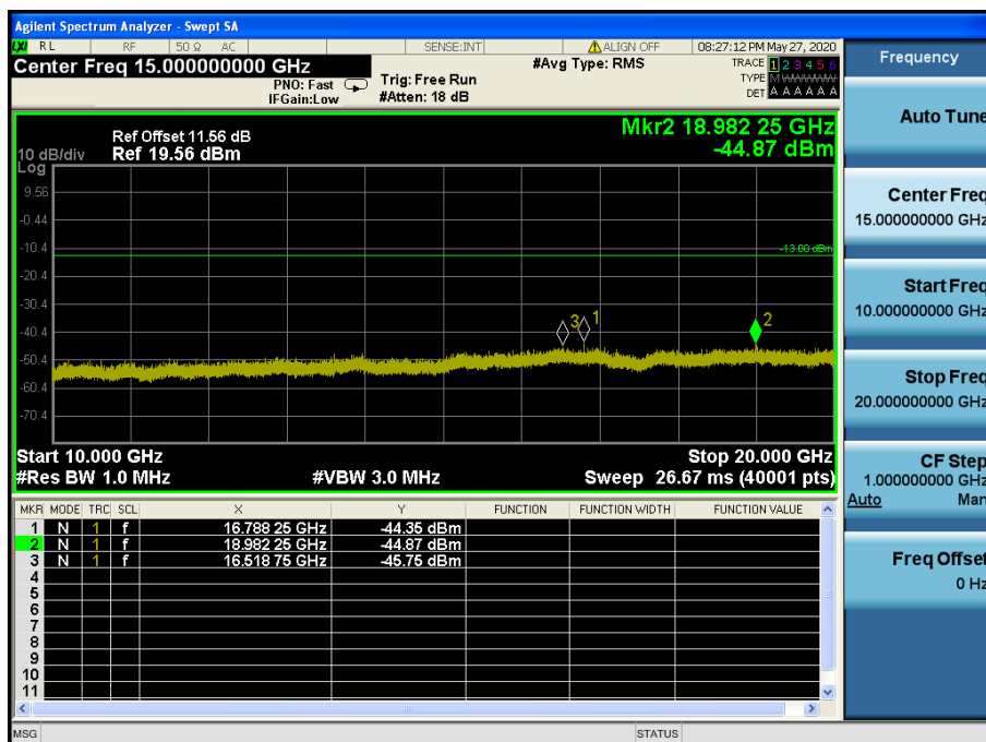
LTE Band 4 / 3 MHz / QPSK - RB Size/Offset (8/0) – Low Channel
