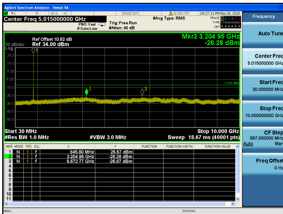
LTE Band 5, 26 / 5 MHz / QPSK - RB Size/Offset (12/0) – High Channel
