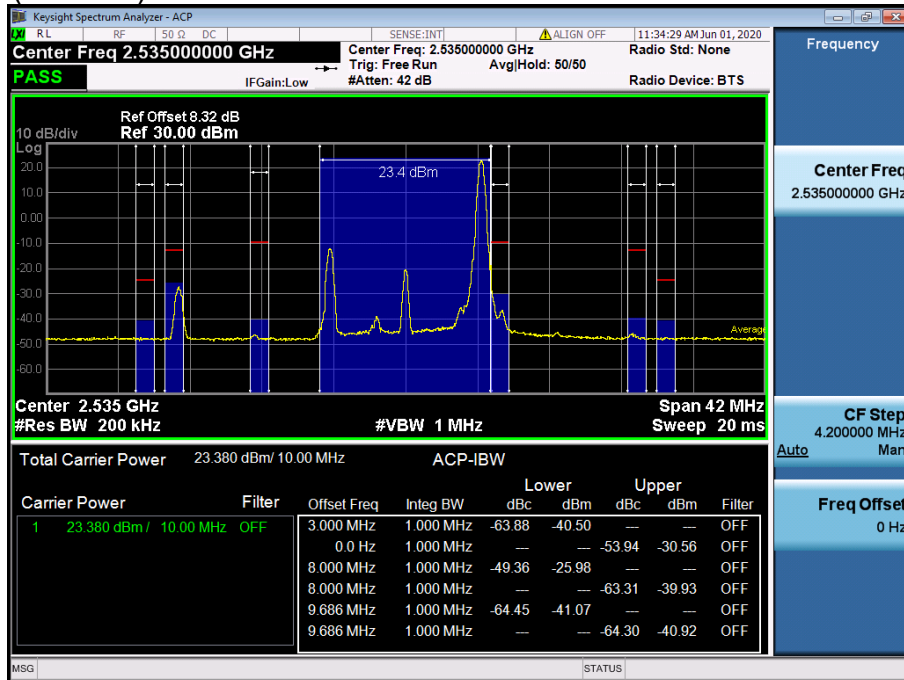
LTE Band 7 / 10 MHz / QPSK - RB Size/Offset (1/49)
