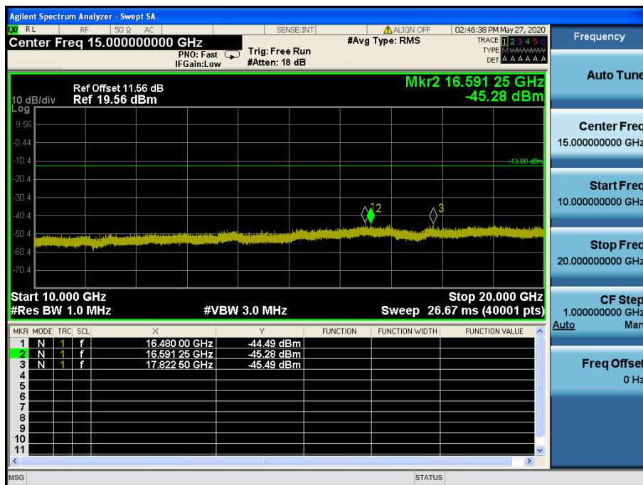
LTE Band 2, 25 / 20 MHz / QPSK - RB Size/Offset (1/50)–Mid Channel
