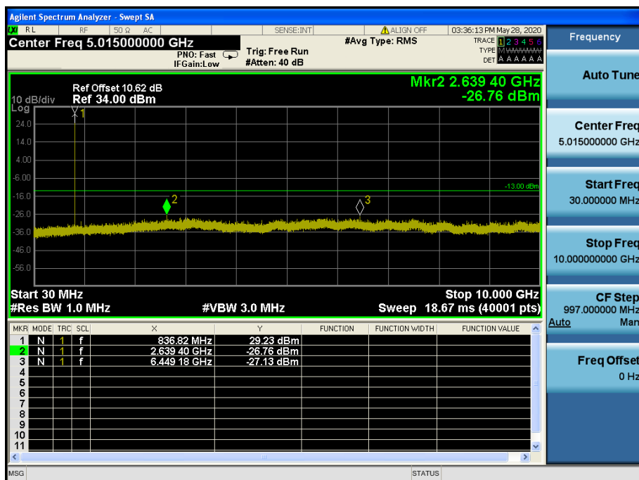
LTE Band 5, 26 / 3 MHz / QPSK - RB Size/Offset (1/7) – Mid Channel
