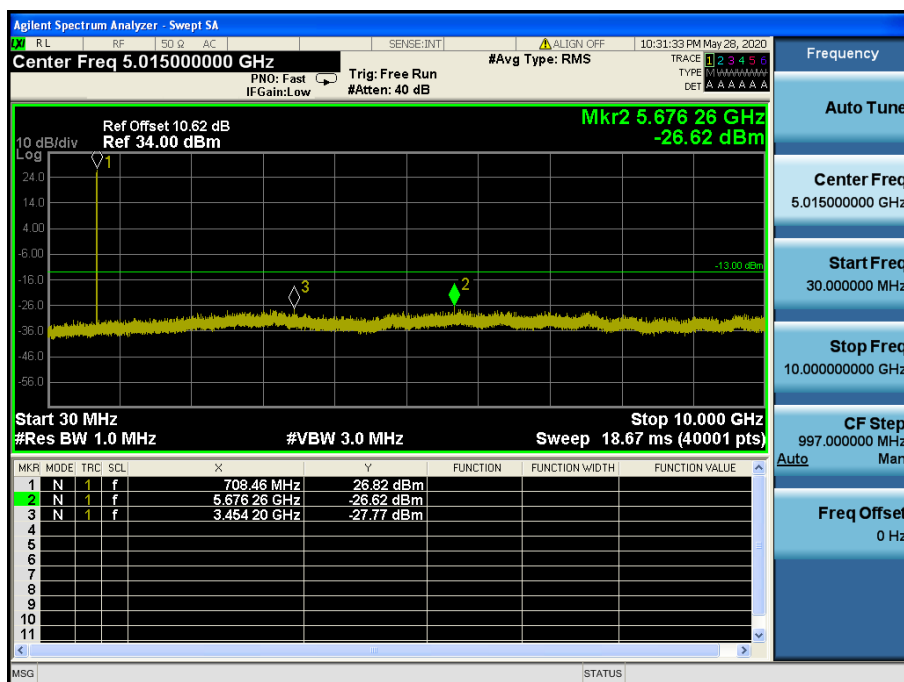
LTE Band 12 / 5 MHz / QPSK - RB Size/Offset (12/6) – Mid Channel
