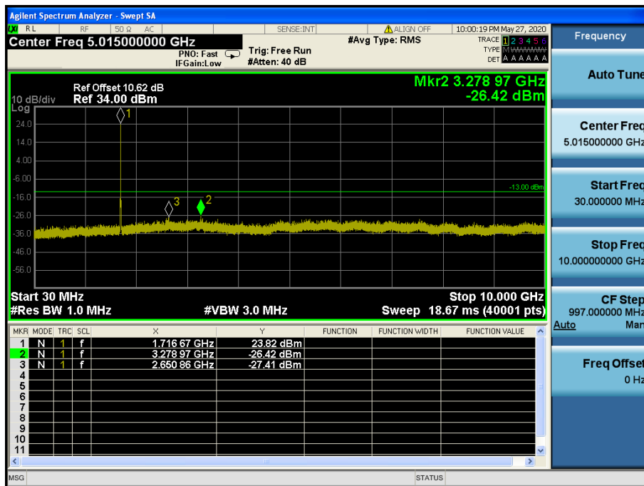
LTE Band 4 / 10 MHz / QPSK - RB Size/Offset (25/25) – Low Channel
