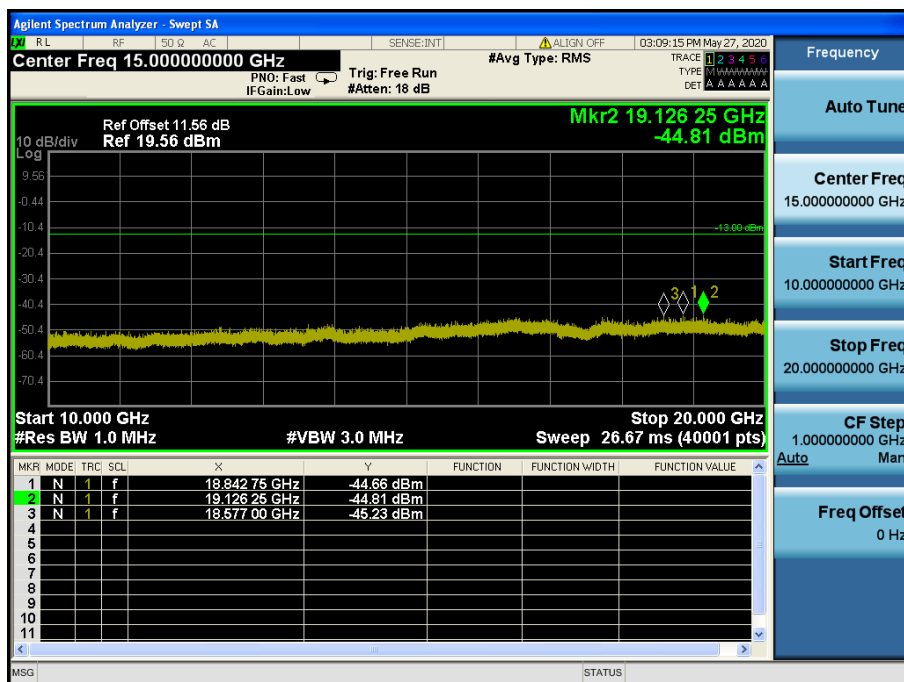
LTE Band 2, 25 / 20 MHz / QPSK - RB Size/Offset (100/0) – High Channel
