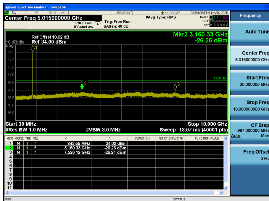
LTE Band 26 / 15 MHz / 16QAM - RB Size/Offset (36/39) – High Channel
