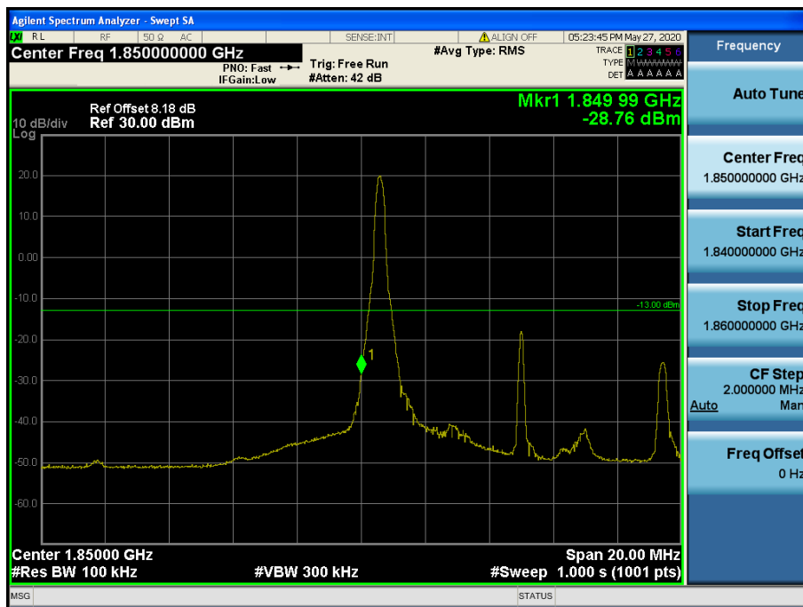
LTE Band 25 / 10 MHz / 16QAM - RB Size/Offset (1/0)
