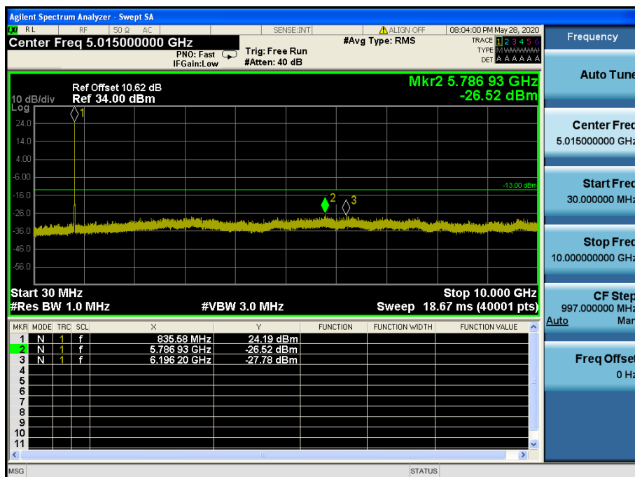
LTE Band 5, 26 / 10 MHz / 16QAM - RB Size/Offset (25/12) – Mid Channel
