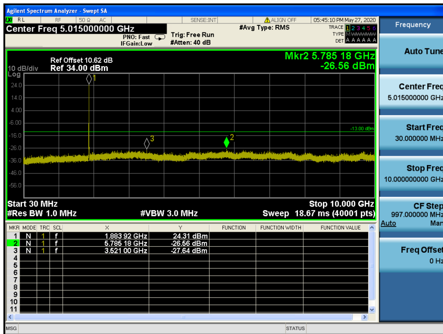
LTE Band 2, 25 / 10 MHz / 16QAM - RB Size/Offset (25/25) – Mid Channel
