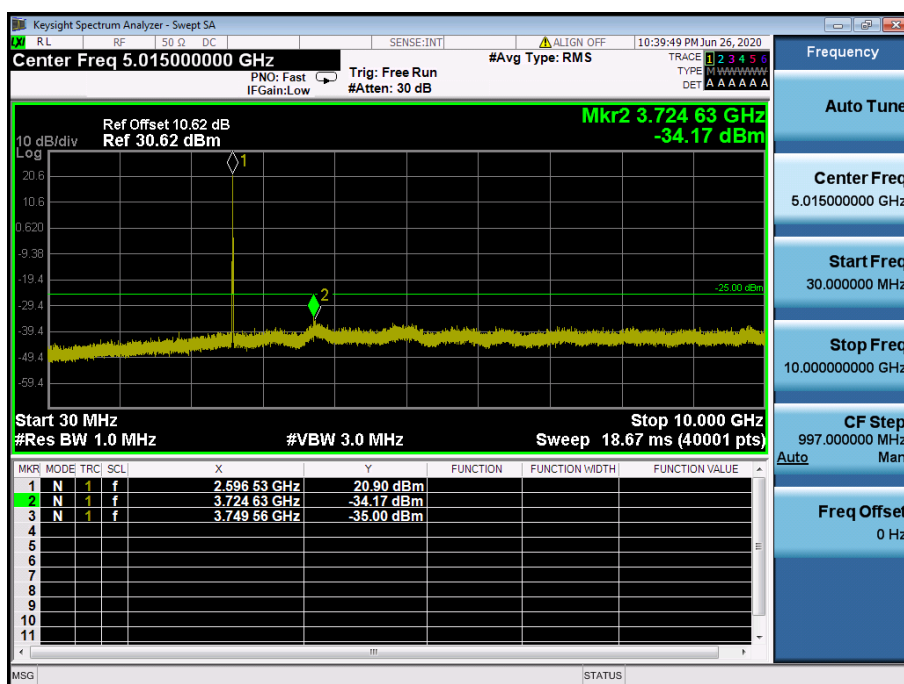
LTE Band 41 / 10 MHz / QPSK - RB Size/Offset (25/25) – Mid Channel
