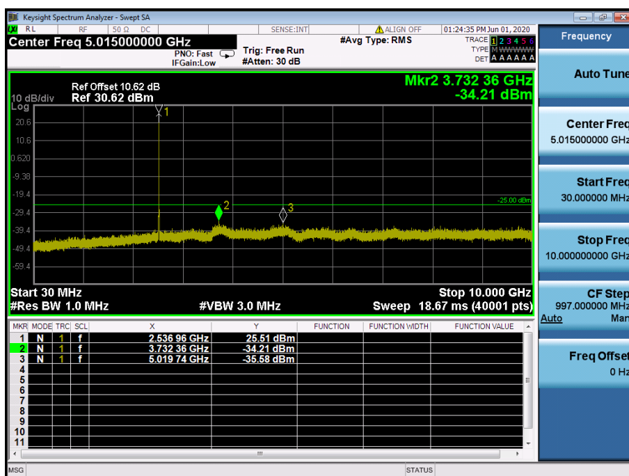
LTE Band 7 / 5 MHz / 16QAM - RB Size/Offset (12/13) – Mid Channel
