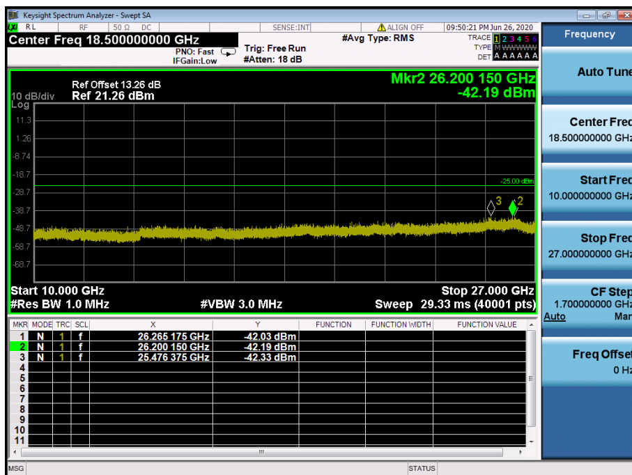
LTE Band 41 / 5 MHz / QPSK - RB Size/Offset (12/0) – Mid Channel
