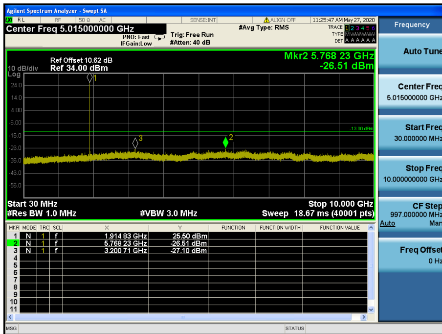
LTE Band 2, 25 / 1.4 MHz / QPSK - RB Size/Offset (3/3) – High Channel
