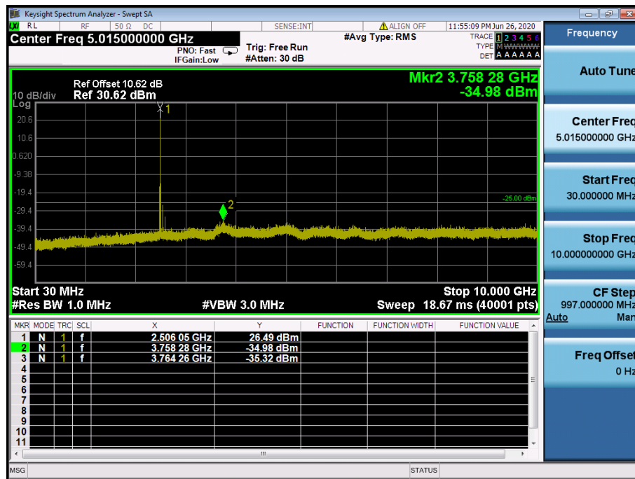
LTE Band 41 / 20 MHz / QPSK - RB Size/Offset (1/50) –Low Channel
