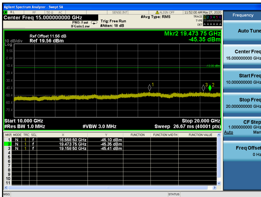
LTE Band 2, 25 / 3 MHz / QPSK - RB Size/Offset (8/0) – Mid Channel
