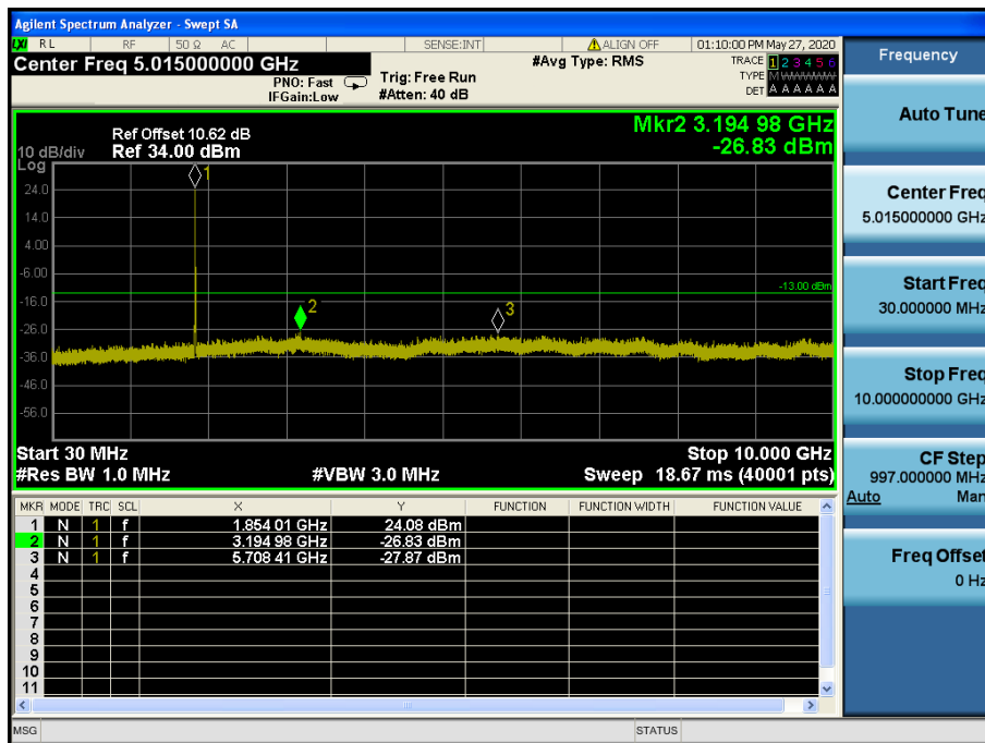
LTE Band 2, 25 / 10 MHz / QPSK - RB Size/Offset (25/0) – Low Channel
