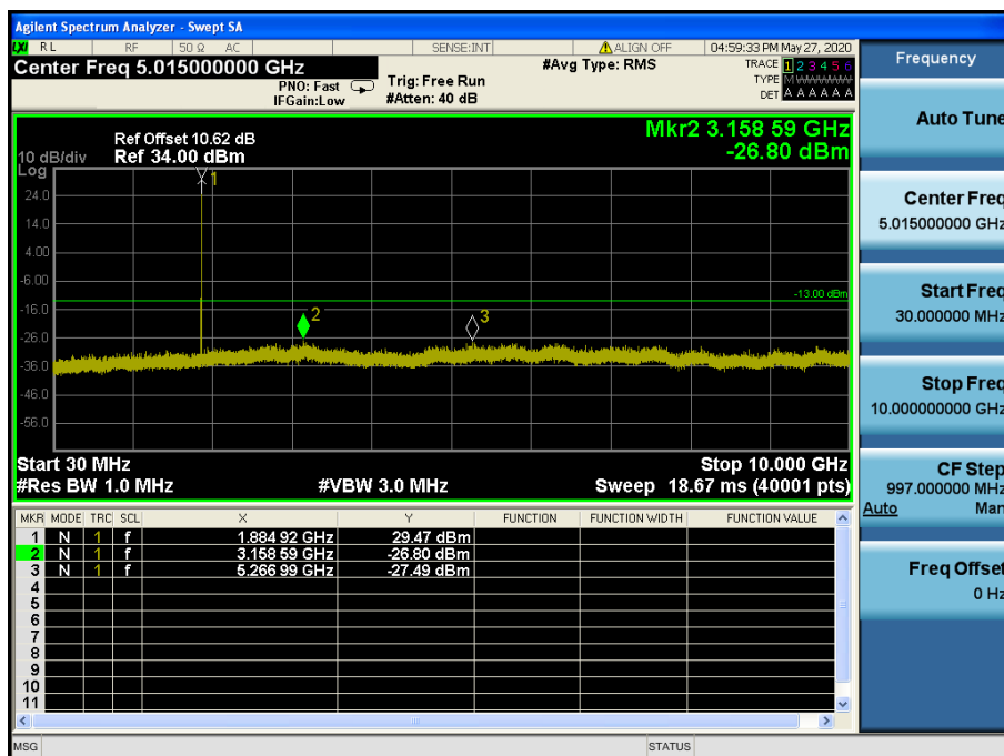
LTE Band 2, 25 / 5 MHz / 16QAM - RB Size/Offset (1/24) – Mid Channel
