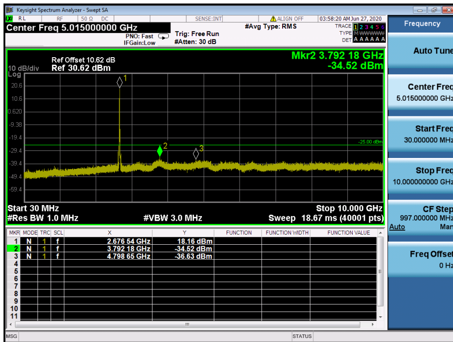
LTE Band 41 / 20 MHz / 16QAM - RB Size/Offset (50/25) – High Channel
