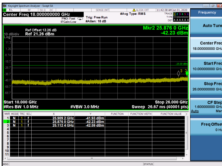
LTE Band 7 / 10 MHz / QPSK - RB Size/Offset (1/0) – High Channel
