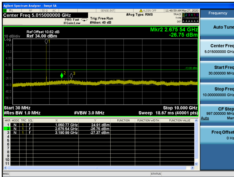
LTE Band 2, 25 / 3 MHz / QPSK - RB Size/Offset (15/0) – Low Channel
