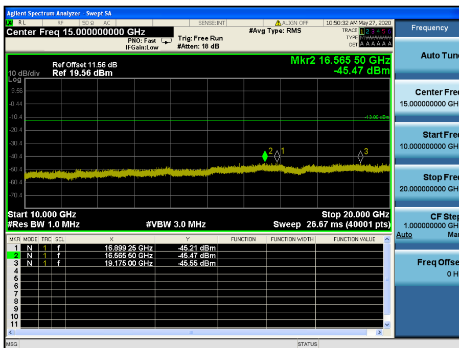
LTE Band 2, 25 / 1.4 MHz / QPSK - RB Size/Offset (1/2) – Low Channel
