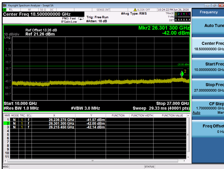
LTE Band 41 / 10 MHz / QPSK - RB Size/Offset (25/25) – Low Channel
