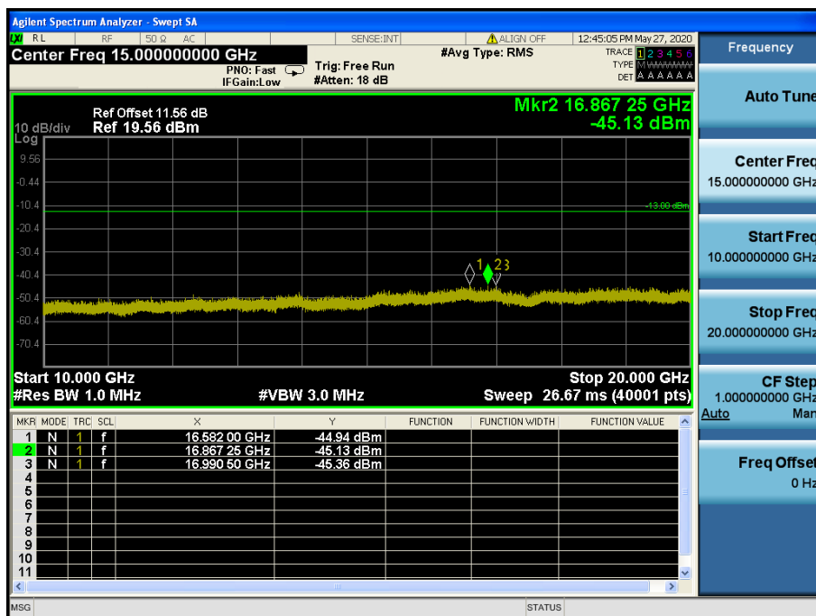
LTE Band 2, 25 / 5 MHz / QPSK - RB Size/Offset (1/12) – High Channel
