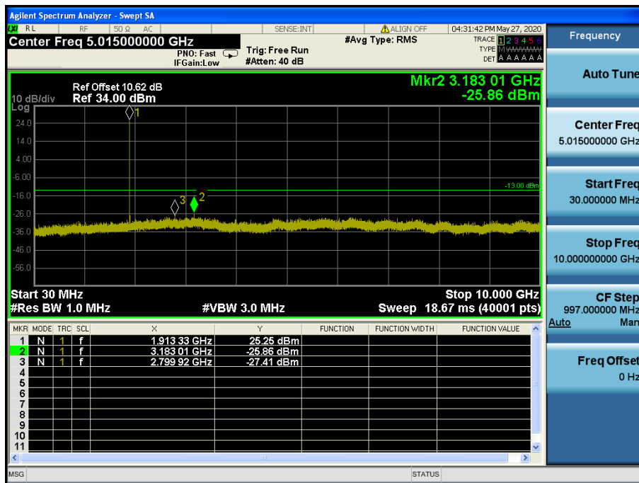
LTE Band 2, 25 / 3 MHz / 16QAM - RB Size/Offset (8/4) – High Channel
