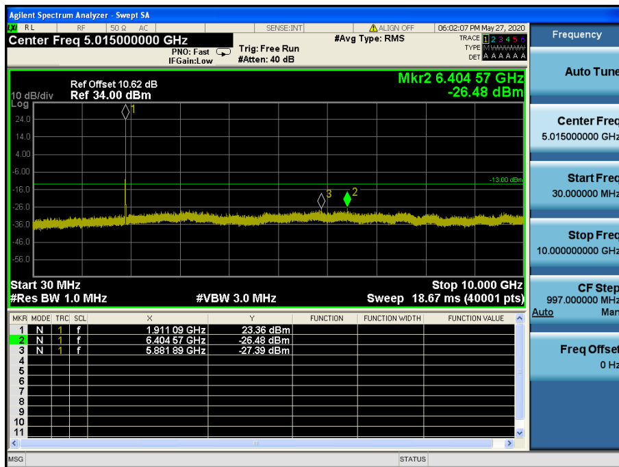
LTE Band 2, 25 / 10 MHz / 16QAM - RB Size/Offset (25/25) – High Channel
