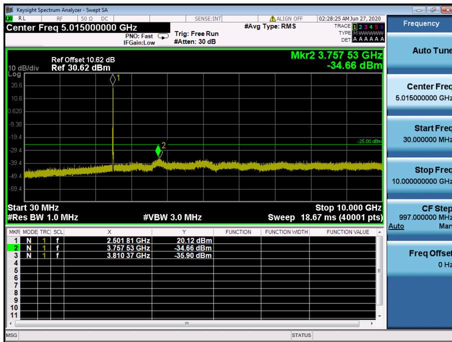
LTE Band 41 / 15 MHz / 16QAM - RB Size/Offset (36/18)-Low Channel
