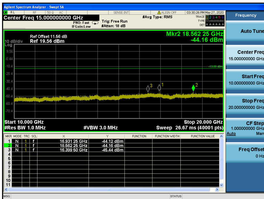
LTE Band 2, 25 / 1.4 MHz / 16QAM - RB Size/Offset (1/2) – Mid Channel
