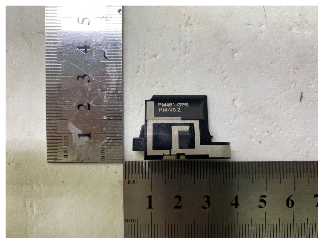
<WIFI Antenna>
