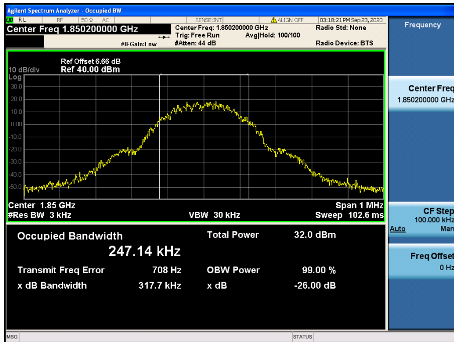
GPRS1900 &amp; Channel: 512
