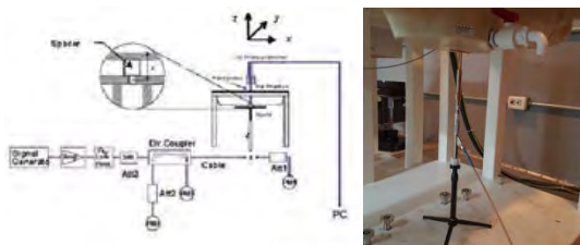
Figure 10.1 Dipole Verification Test Setup Diagram & Photo
